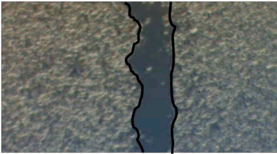
B pCMV-control
