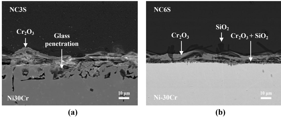
Figure 4.18: Micrographs of Ni-30Cr alloy after 24 h of immersion in (a) NC3S and (b) NC6S at 1100^\circ\text{C}
