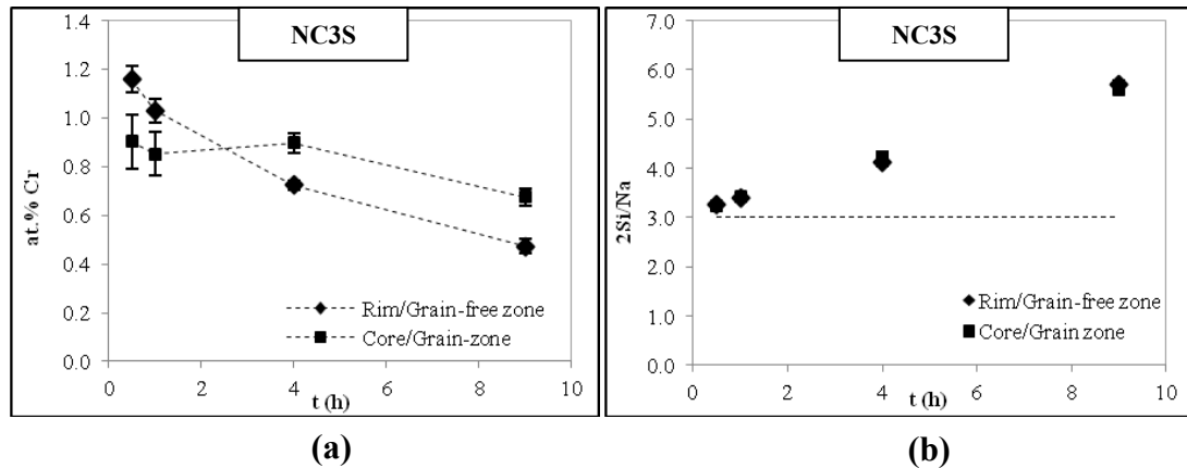
Figure 5.20: Plots of (a) distribution of dissolved Cr (at.%) and (b) evolution of 2Si/Na ratio as a function of time in NC3S at 1300°C under oxidising atmosphere (air). The dotted lines in (a) are guides to the eyes whereas the dotted line in (b) is the theoretical ratio
