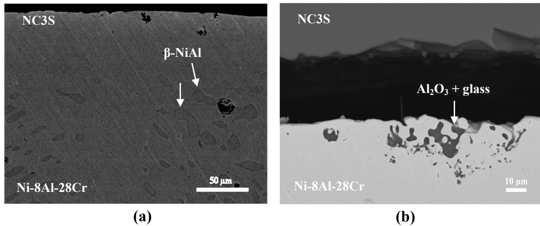
Figure 4.32: Micrographs of preoxidised Ni-8Al-28Cr (24 h in air at 1100 ^\circ\text{C} ) after 2 h of immersion in NC3S at 1100 ^\circ\text{C} with magnification of (a) 500x and (b) 1000x
