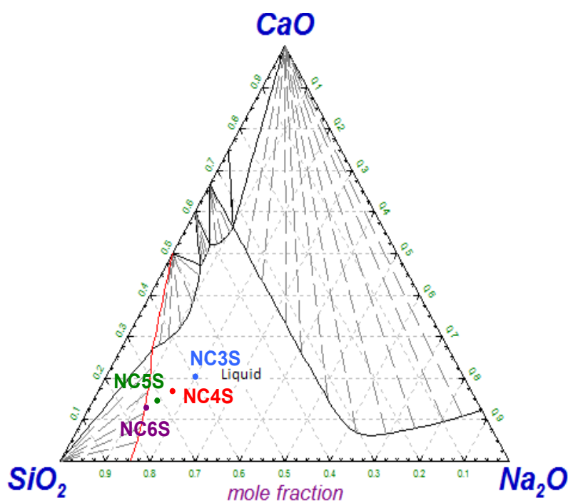
Figure C.1: Ternary phase diagram of Na 2 O-CaO-SiO 2 system at 1300°C
