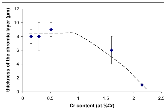
Figure 4.22: Thickness of the Cr 2 O 3 layer on the preoxidised Cr or Ni-30Cr samples after 24 h of immersion in N1.5S, N2S and NC3S at 1050°C (or 1100°C for the Ni-30Cr alloy) as a function of Cr content measured near the glass/oxide layer interface. The dotted line is a guide to the eyes.
