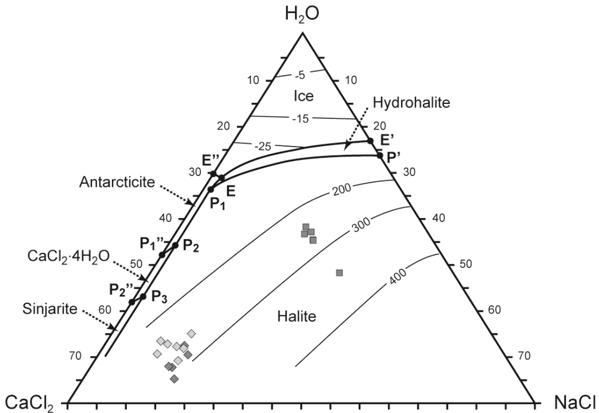
Figure 65: Vapor-saturated phase equilibria in the \text{H}_2\text{O-NaCl-CaCl}_2 system showing isotherms (in degrees Celsius) of halite solubility and ice-melting (modified after Steele-MacInnis et al., 2011). Diamond symbols represent data for type-I fluid inclusions (dark grey diamond => Lolwa occurrence; light grey diamond => Mitukuluku occurrence) and square symbols for type-IIA fluid inclusions (dark grey square => Lolwa occurrence; no type-IIA fluid inclusions were found in Mitukuluku occurrence). Abbreviations: E = \text{H}_2\text{O-CaCl}_2\text{-NaCl} eutectic ( -52.0\text{ }^\circ\text{C} ); E' = \text{H}_2\text{O-NaCl} eutectic ( -21.2\text{ }^\circ\text{C} ); E'' = \text{H}_2\text{O-CaCl}_2 eutectic ( -49.9\text{ }^\circ\text{C} ); P1 = \text{H}_2\text{O-CaCl}_2\text{-NaCl} first peritectic ( -22.4\text{ }^\circ\text{C} ); P2 = \text{H}_2\text{O-CaCl}_2\text{-NaCl} second peritectic ( 29.0\text{ }^\circ\text{C} ); P3 = \text{H}_2\text{O-CaCl}_2\text{-NaCl} third peritectic ( 45.0\text{ }^\circ\text{C} ); P' = \text{H}_2\text{O-NaCl} peritectic ( 0.1\text{ }^\circ\text{C} ); P1'' = \text{H}_2\text{O-CaCl}_2 first peritectic ( 30.1\text{ }^\circ\text{C} ); P2'' = \text{H}_2\text{O-CaCl}_2 second peritectic ( 45.1\text{ }^\circ\text{C} ).
