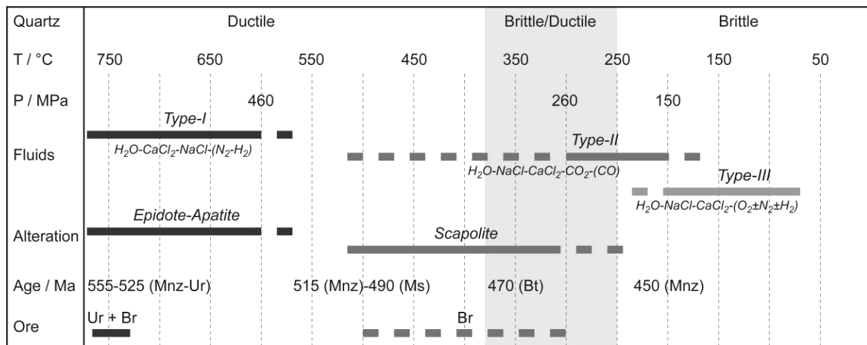
Figure 82: Fluid evolution, with respective P-T trapping conditions, related to fluid-rock alteration and uranium mineralization. Minerals on brackets represent the dating material and ages are from this study and from John (2001). Abbreviations: Br = Brannerite; Bt = Biotite; Mnz = Monazite; Ms = Muscovite; Ur = Uraninite.
