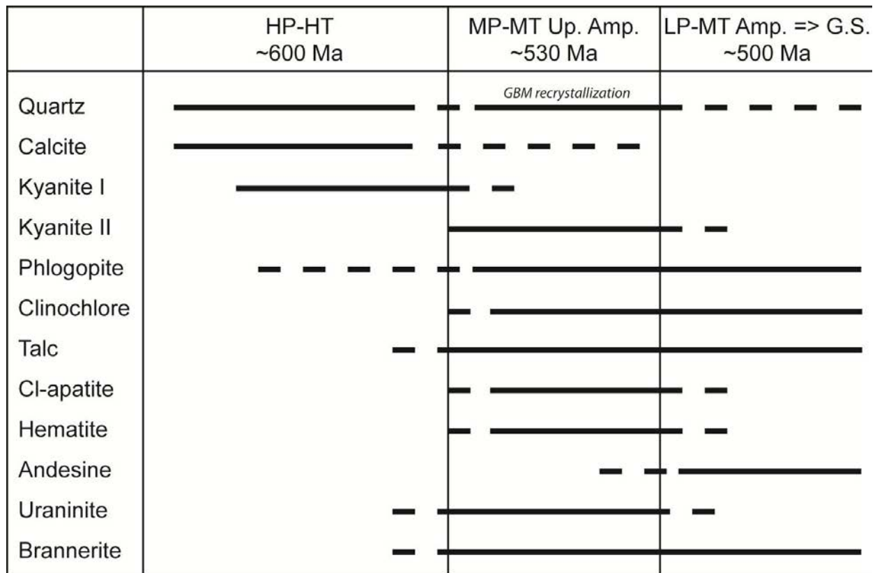
Figure 61: General paragenetic sequence of the kyanite±talc micaschist from Lolwa (Kabompo dome) and Mitukuluku (Solwezi dome) occurrences in the internal zone. Abbreviations: Up. Amp. = Upper Amphibolite; G.S. = Greenschist; GBM = Grain boundary migration.
