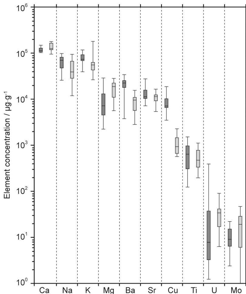
Figure 66: Box diagram of Ca, Na, K, Mg, Ba, Sr, Cu, Ti, U and Mo element concentrations in Lolwa (dark grey) and Mitukuluku (light grey) fluid inclusions. Lower whiskers, bottoms of boxes, central lines, tops of boxes and upper whiskers represent 5 th , 25 th , 50 th , 75 th and 95 th percentiles, respectively.
