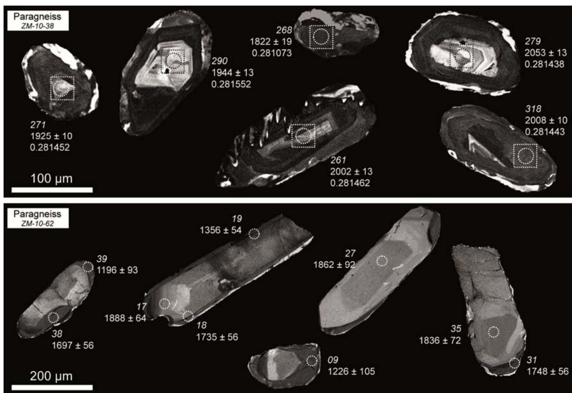
Figure 14: Cathodoluminescence images of some analyzed zircon grains of the paragneissic rocks from the Solwezi dome. Dotted circles represent the points of analyses. Italic numbers are the referees label (see complementary data) and regular numbers are the ^{207}\text{Pb}/^{206}\text{Pb} ages with concordance >95% and the ^{176}\text{Hf}/^{177}\text{Hf}(t) ratio.
