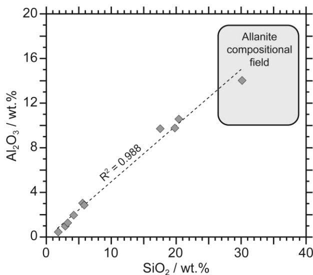
Figure 76: \text{Al}_2\text{O}_3 vs. \text{SiO}_2 diagram for electron microprobe analyses of altered monazite grains (dark grey diamonds). The linear trend toward the allanite compositional field defined after 30 analyses reported in Deer et al. (1997), suggests that the monazite alteration leads to allanite replacement.
