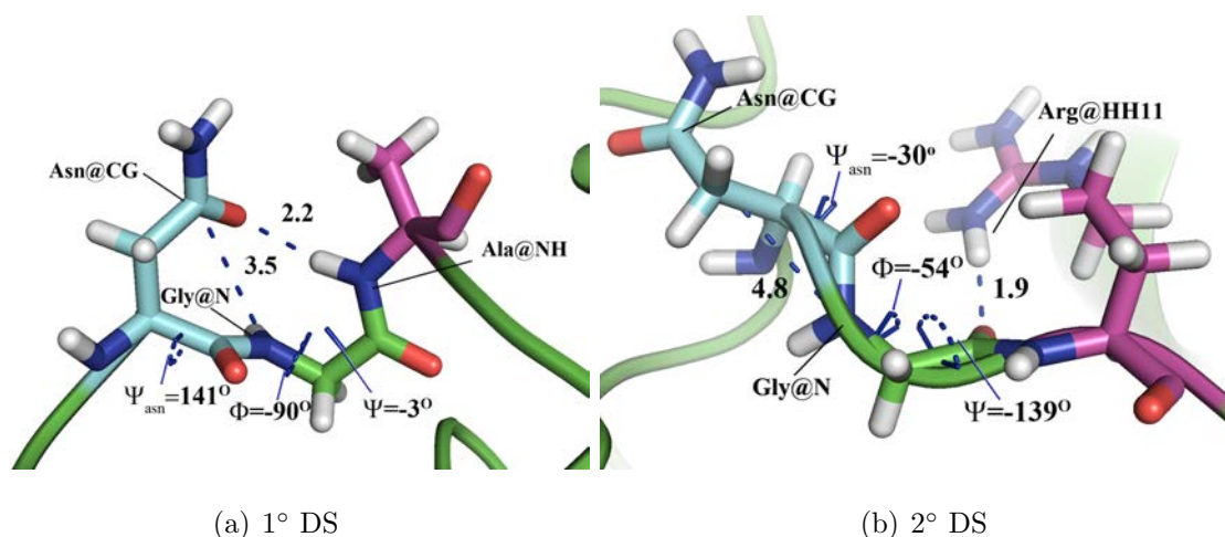
Figure 5.15. Representative structures of 1° and 2° deamidation sites (DS) showing the most frequently observed interactions and dihedrals, sample WOW. Asn, Gly and the rest of the peptide are colored with cyan, green and purple, respectively.
