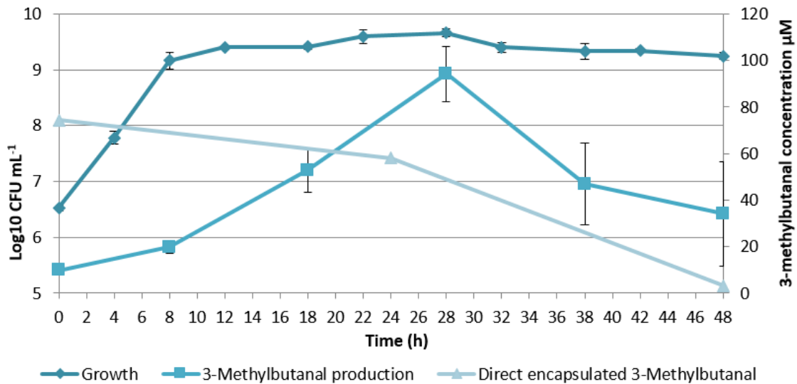
Figure 15. C. maltaromaticum LMA28 growing and 3-methylbutanal production kinetics.
