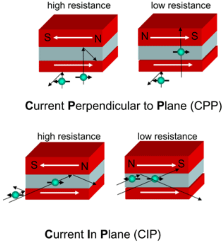
Figure 1.14 Schematic of current perpendicular to plane (CPP) and the current in plane (CIP) geometry [25].
