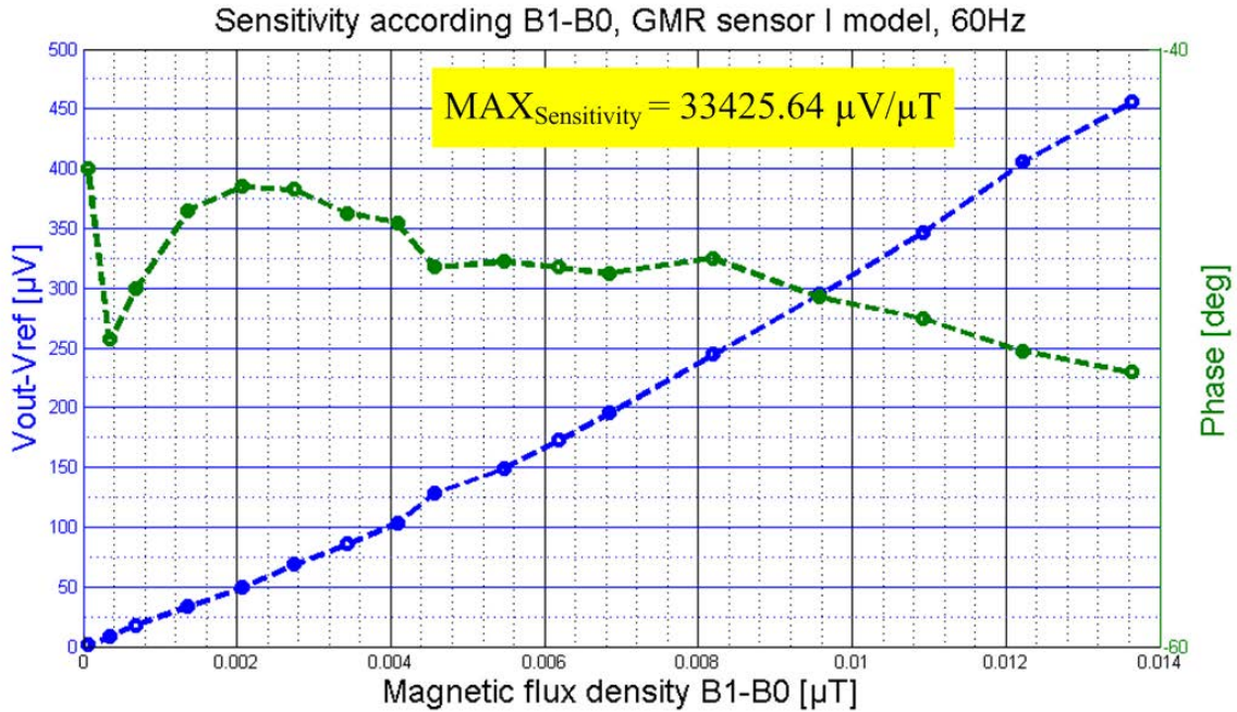
Figure 2.31 The output voltage result by GMR sensor I ( \mu\text{V} ) and phase calculation (deg) with two resistors ( 809 \Omega ) as a function of different magnetic flux density ( \mu\text{T} ) between two sensing elements GMR.
