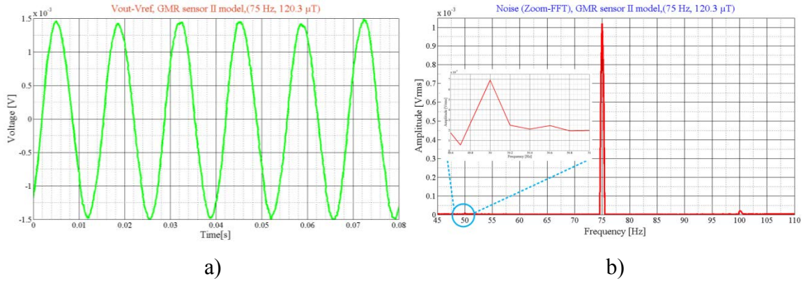
Figure 2.43 The GMR sensor’s output voltage ( V ) with 2.128\text{ k}\Omega (a) and FFT detection from V_{out}-V_{ref} of the GMR sensor for frequency 75\text{ Hz} (b).
