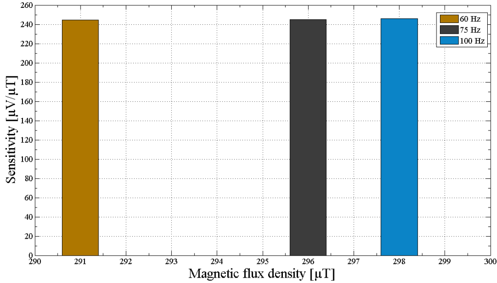
Figure 2.54 High value of sensitivity ( \mu V/\mu T ) as a function of B ( \mu T ) at f=60, 75, 100 Hz.
