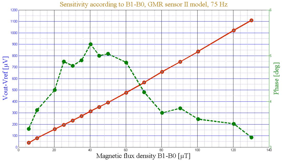
Figure 2.44 The output voltage results obtained by the probe GMR sensor ( \mu\text{V} ) and phase calculation (deg) with one resistor ( 2.128\text{ K}\Omega ) as a function of the changes in magnetic flux density ( \mu\text{T} ).
