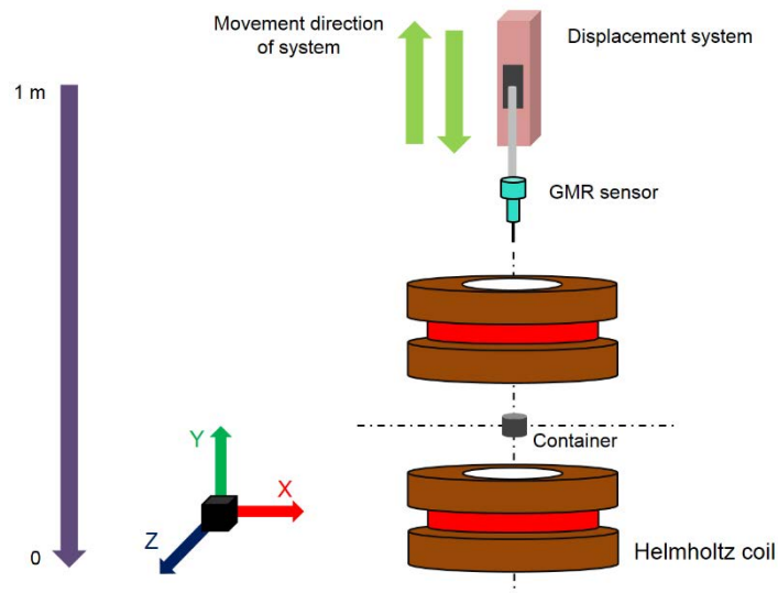
Figure 2.12 Positioning the displacement system of the GMR sensor.
