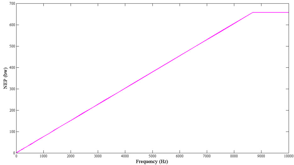
Figure 2.21 Noise equivalent power according to frequency (Hz).
