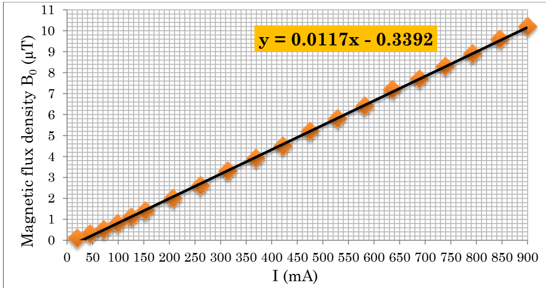
Figure 2.35 Measurement the magnetic flux density B_0 ( \mu T ) as a function of the input current ( mA ) applied to 60 Hz.
