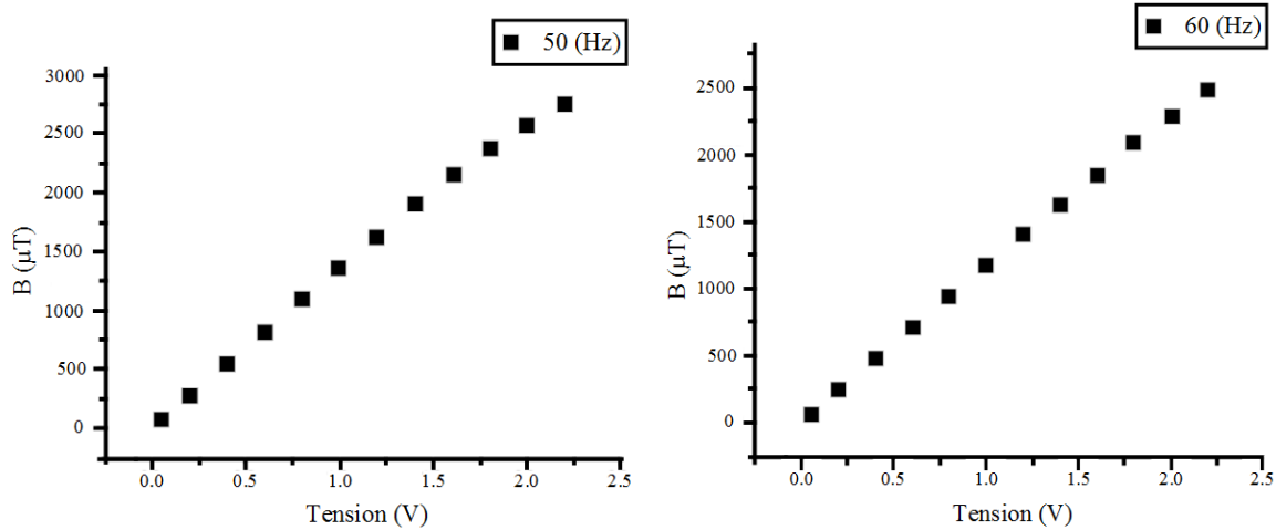
Figure 2.9 Measurement the magnetic flux density ( \mu\text{T} ) as a function of the input voltage applied to 50 and 60 Hz.
