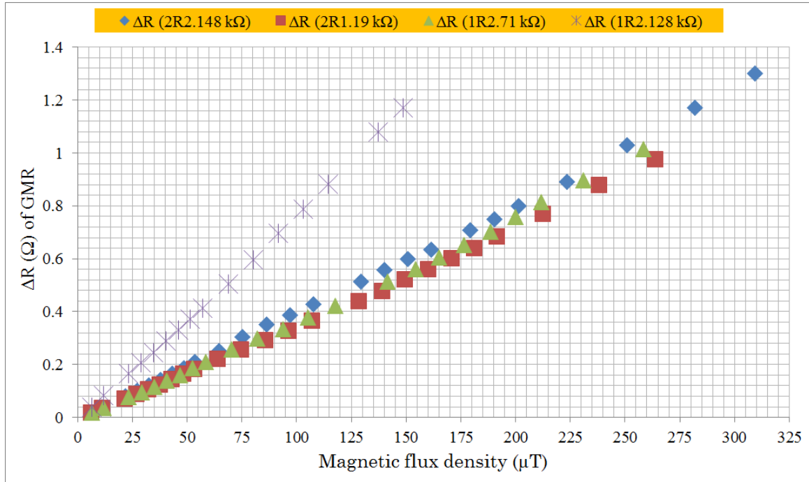
Figure 2.48 The values of \Delta R according to magnetic flux density ( \mu T ) by several resistances in interface supply card of the GMR sensor.
