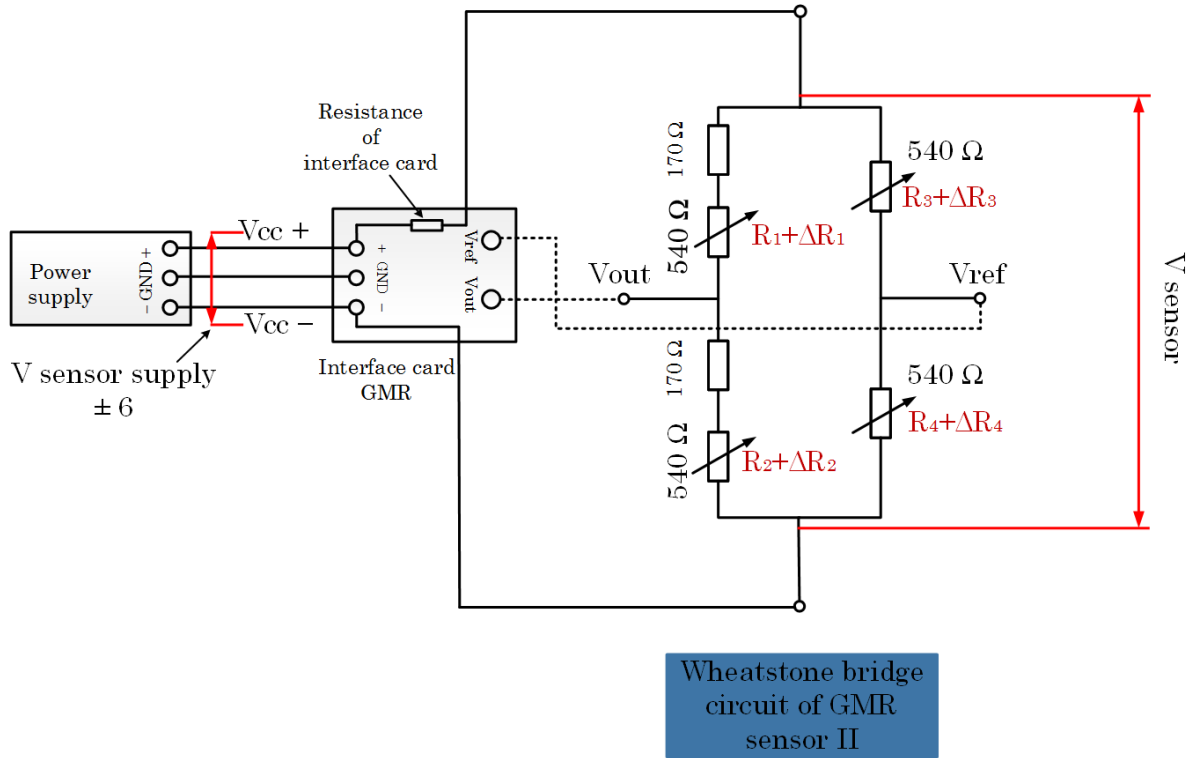
Figure 2.47 Schematic of the GMRII sensor (second model).
