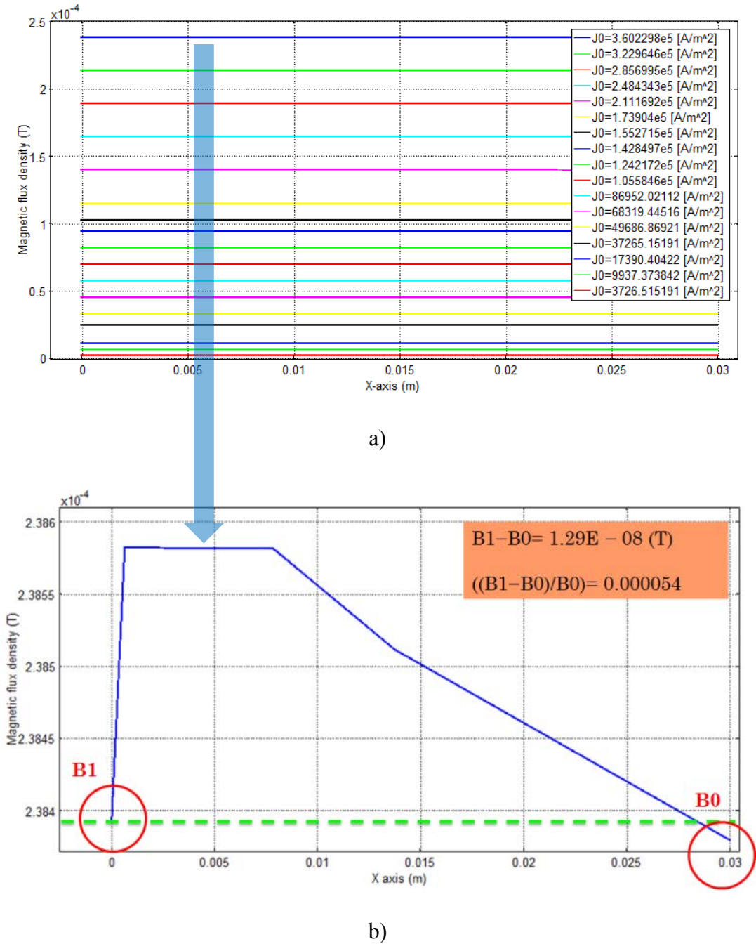
Figure 2.30 Distribution of the magnetic flux density (T) along the needle of sensor (a), zooming on a curve of the figure 2.30 (a) which presents the difference B between two GMR (b).
