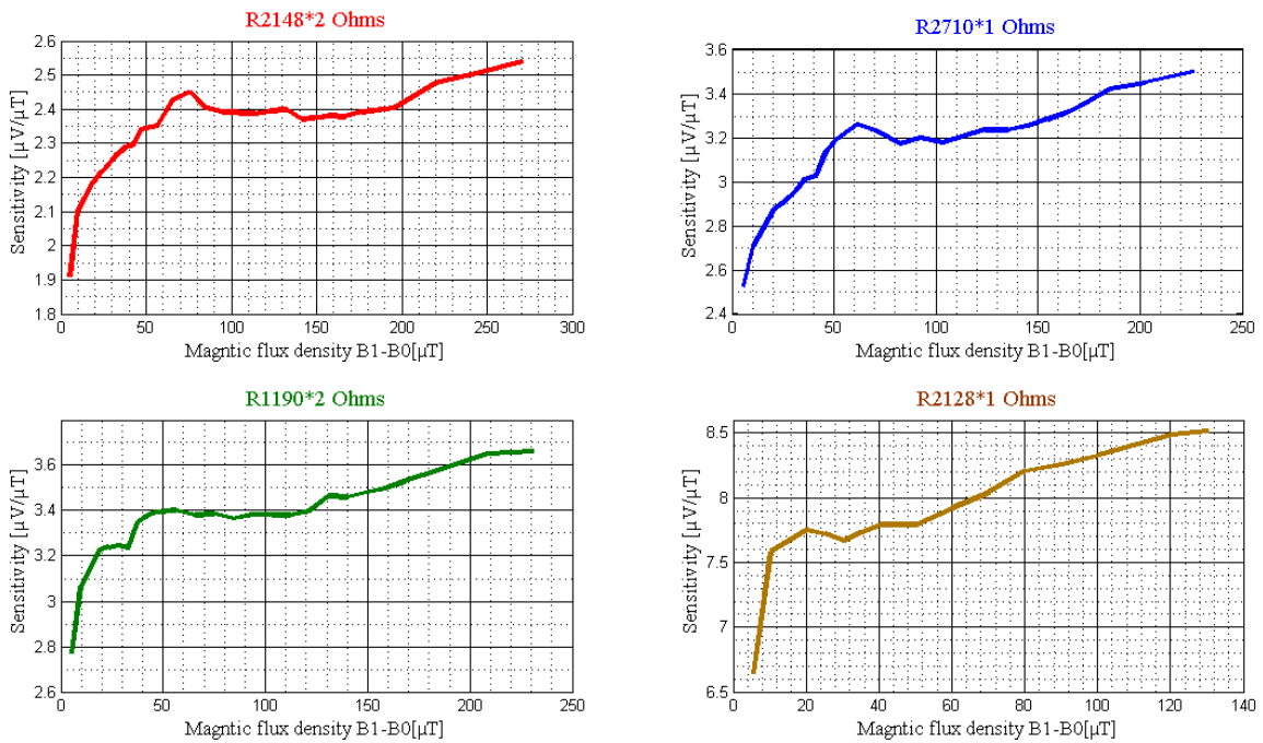
Figure 2.45 The relationship between sensitivity ( \mu\text{V}/\mu\text{T} ) and the magnetic flux density ( \mu\text{T} ) variations for different resistances values in the power supply card of the GMR sensor.
