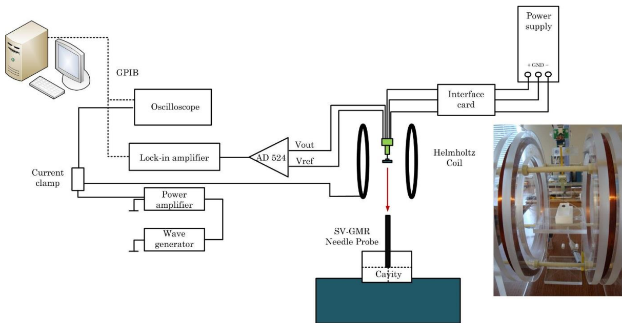
Figure 3.4 Measurement setup.
