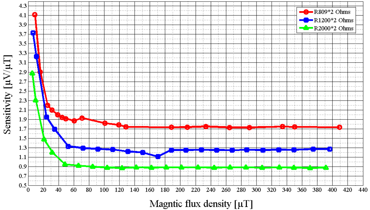
Figure 2.36 The relationship between sensitivity ( \mu V/\mu T ) and changes of the magnetic flux density ( \mu T ) by using several resistances in the interface card of the GMR sensor I.
