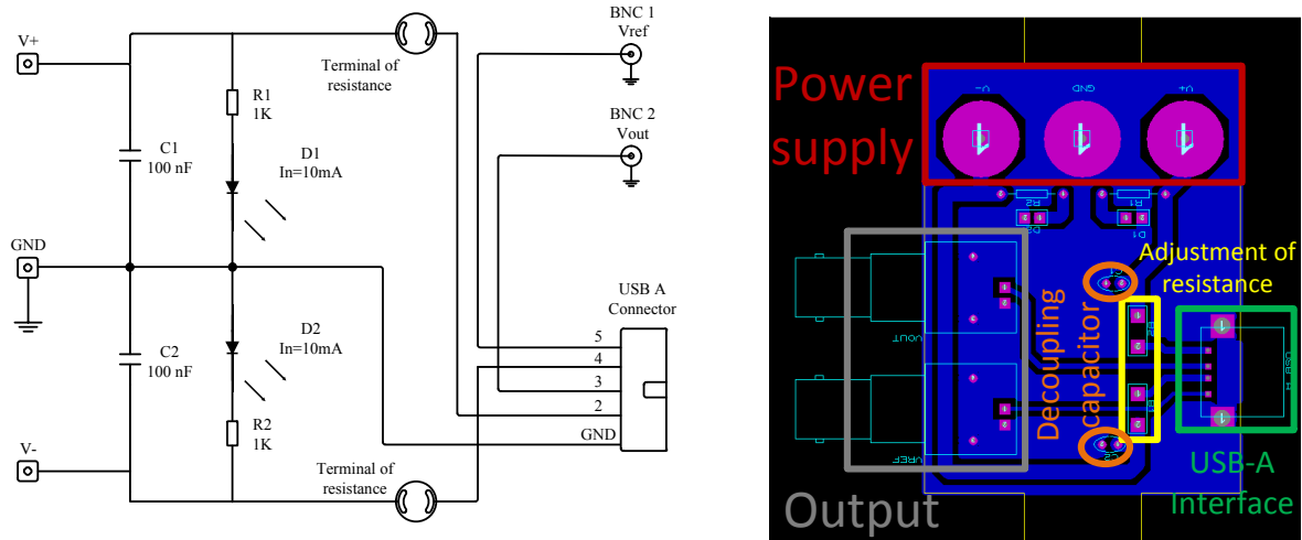
Figure 2.3 The schematic of connection card between sensor and power supply.
