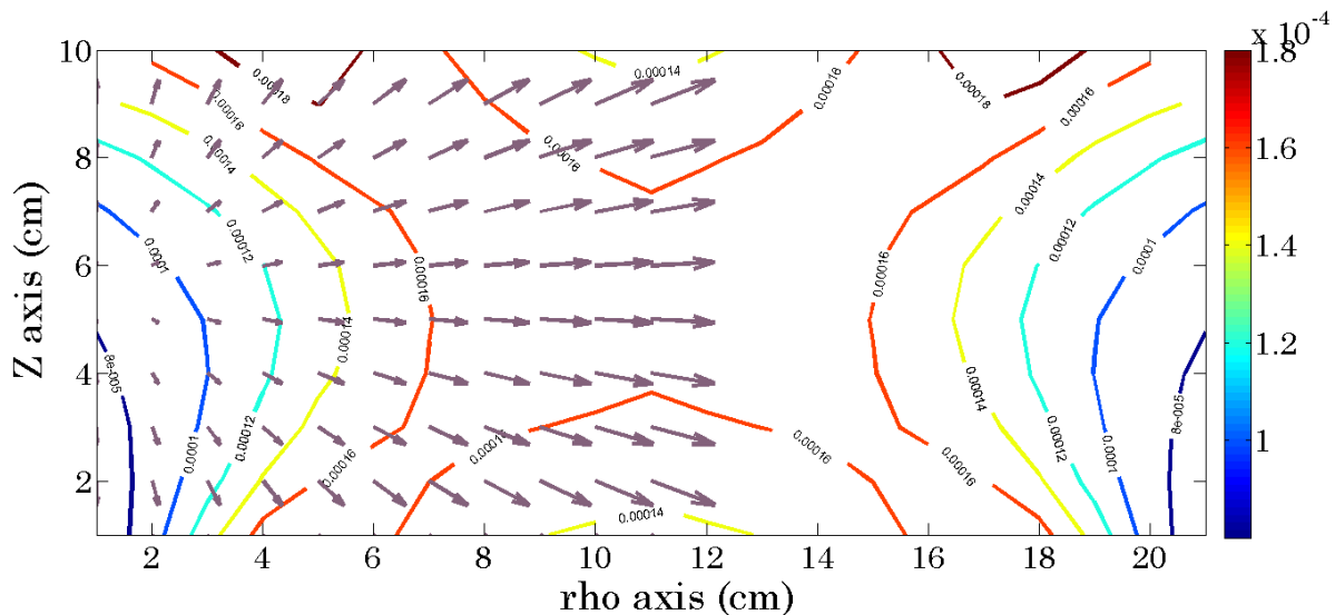
Figure 3.6 Distribution of magnetic flux density ( B ) in a sphere of the Helmholtz coil.
