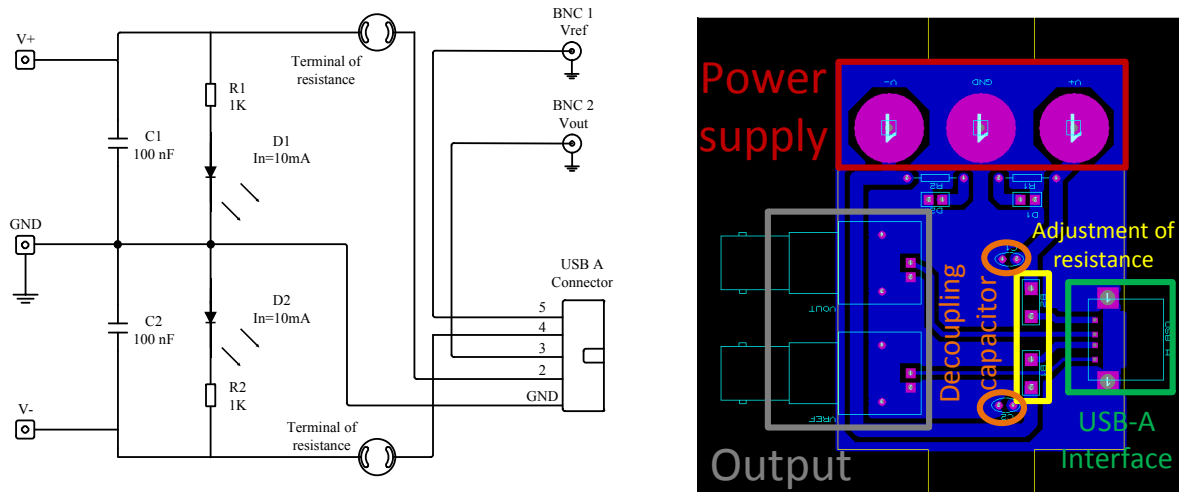
Figure 2.3 The schematic of connection card between sensor and power supply.
