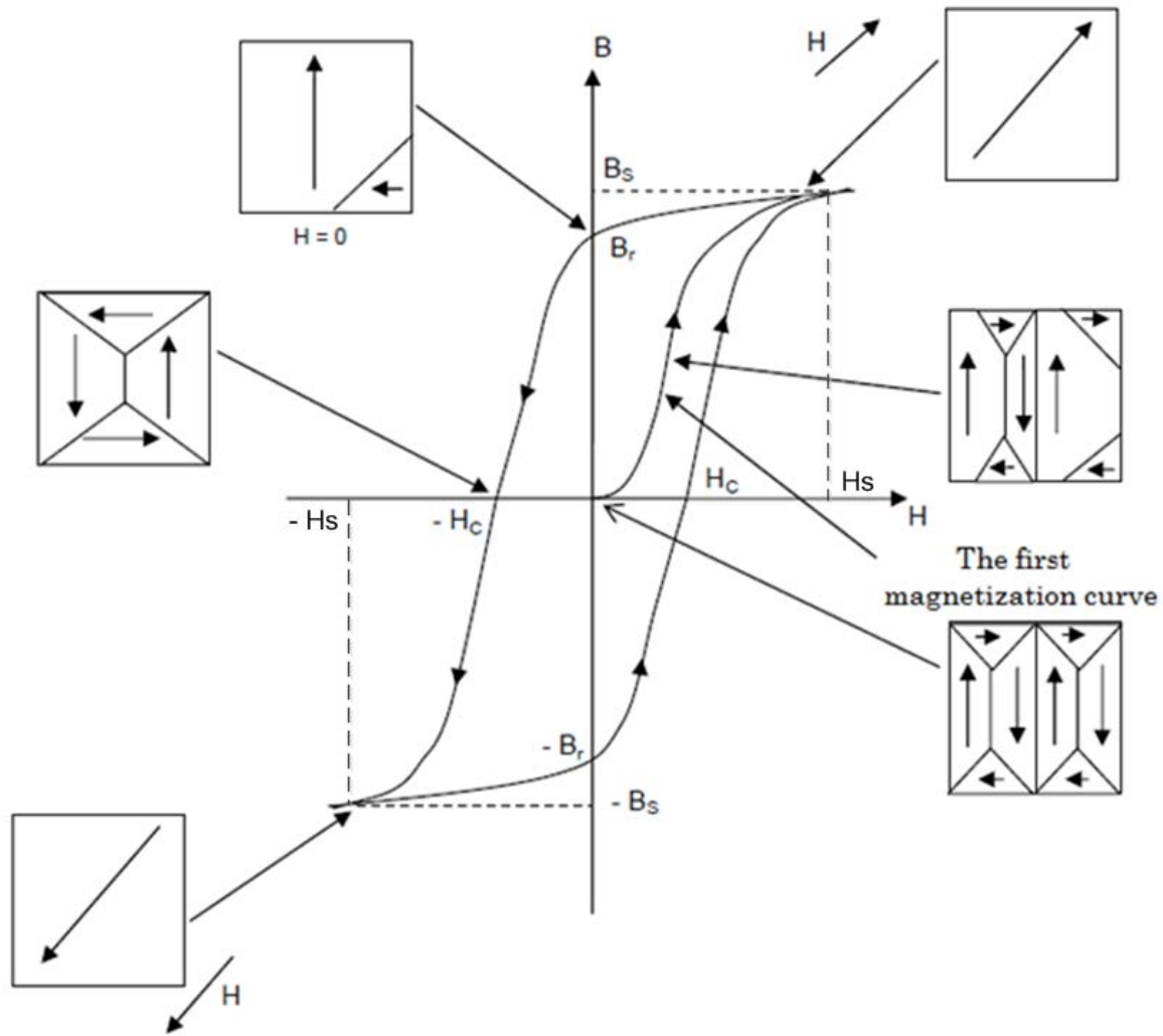
Figure 1.21 The basic magnetization curve and hysteresis loop of a ferromagnetic: B is refers to the magnetization of the particle; H is the magnetic field; B_s is saturation magnetization for H > H_s ; H_s is saturation field corresponding to B_s ; B_r is residual magnetization; H_c is coercive force or field necessary for the demagnetization of the particle [43].
