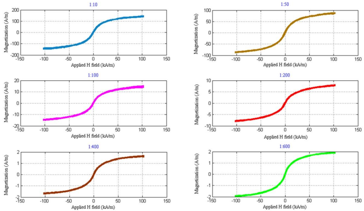
Figure 3.12 Hysteresis curve of fluids obtained from pure ferrofluid.
