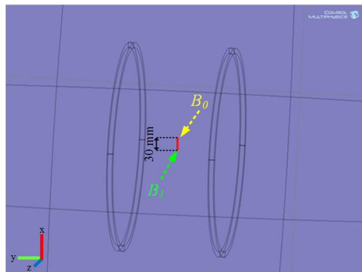
Figure 2.29 Calculation of the magnetic flux density ( B ) along the needle of sensor.
