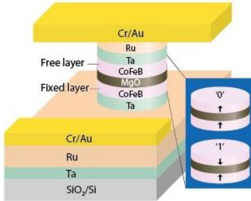
Figure 1.15 Structure representation of a magnetic tunnel junction (ferromagnetic layer fixed (CoFeB) and the other layer free to rotate in to each condition, low resistance ('0') or high resistance ('1'), MgO is a barrier layer [30].
