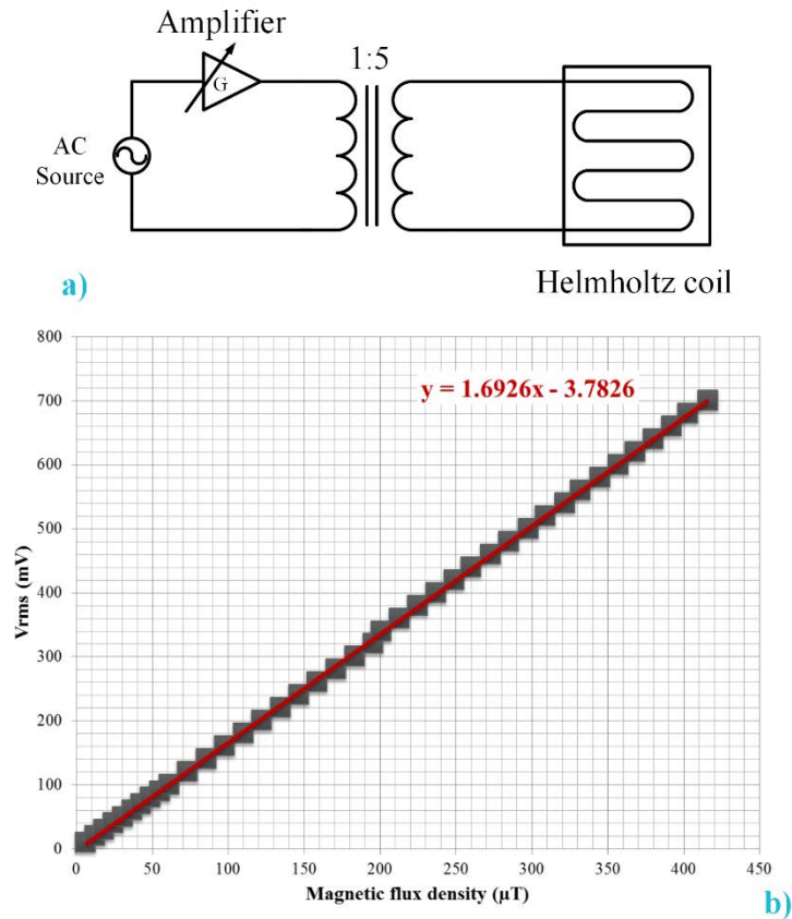
Figure 4.11 Helmholtz coil and its supply for operating in the frequency range 45-1000 Hz (a), measured magnetic flux density ( \mu\text{T} ) as a function of signal amplitude ( V_{\text{rms}} ) applied at 75 Hz (b).
