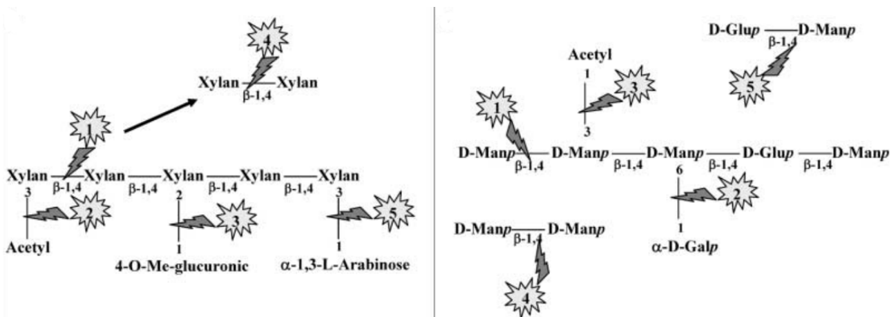
Figure 1.17. (Left) Enzymatic degradation of glucuronoxylans, found in hardwoods. 1 Endoxylanase, 2 acetylxyylan-esterase, 3 \alpha -glucuronidase, 4 \beta -xylosidase, 5 \alpha -arabinase. (Right) Enzymatic hydrolysis of glucomannan found in softwoods. 1 Endomannase, 2 \alpha -galactosidase, 3 acetylglucomannan-esterase, 4 \beta -mannosidase, 5 \beta -glucosidase (from Pérez et al. 2002).
