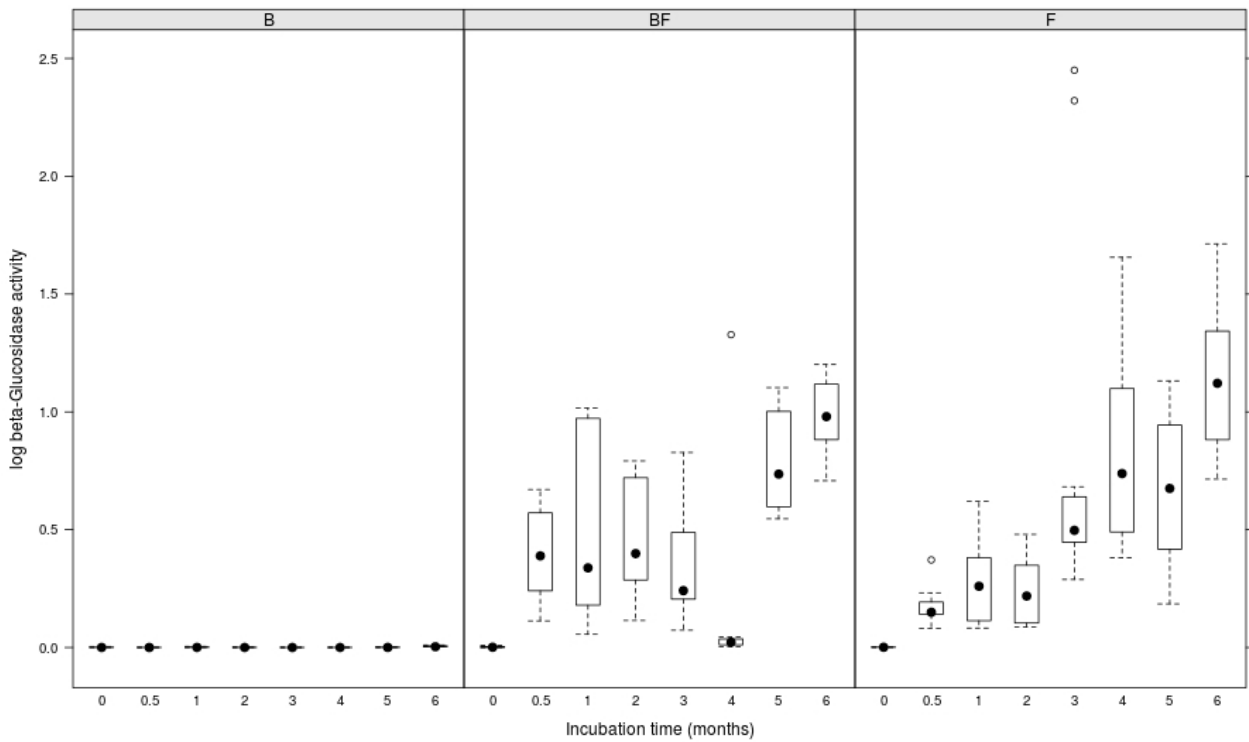
Figure 5.2. Logarithm of beta-glucosidase activity ( \text{nmol h}^{-1} \text{g}^{-1} of dry wood) as a function of incubation time and type of microbial inoculum. For B, n=4 ; for BF and F, n=8 .
