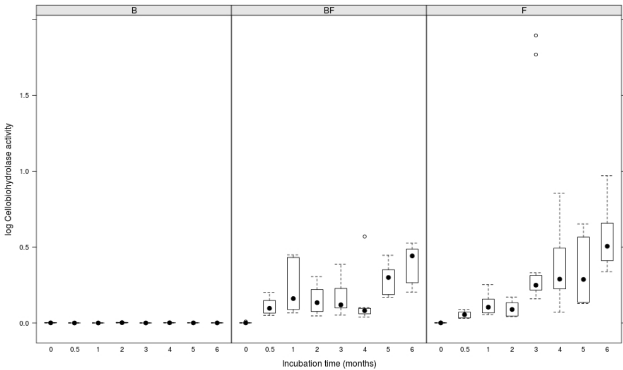
Figure 5.3. Logarithm of cellobiohydrolase activity ( \text{nmol h}^{-1} \text{g}^{-1} of dry wood) as a function of incubation time and type of microbial inoculum. For B, n=4 ; for BF and F, n=8 .
