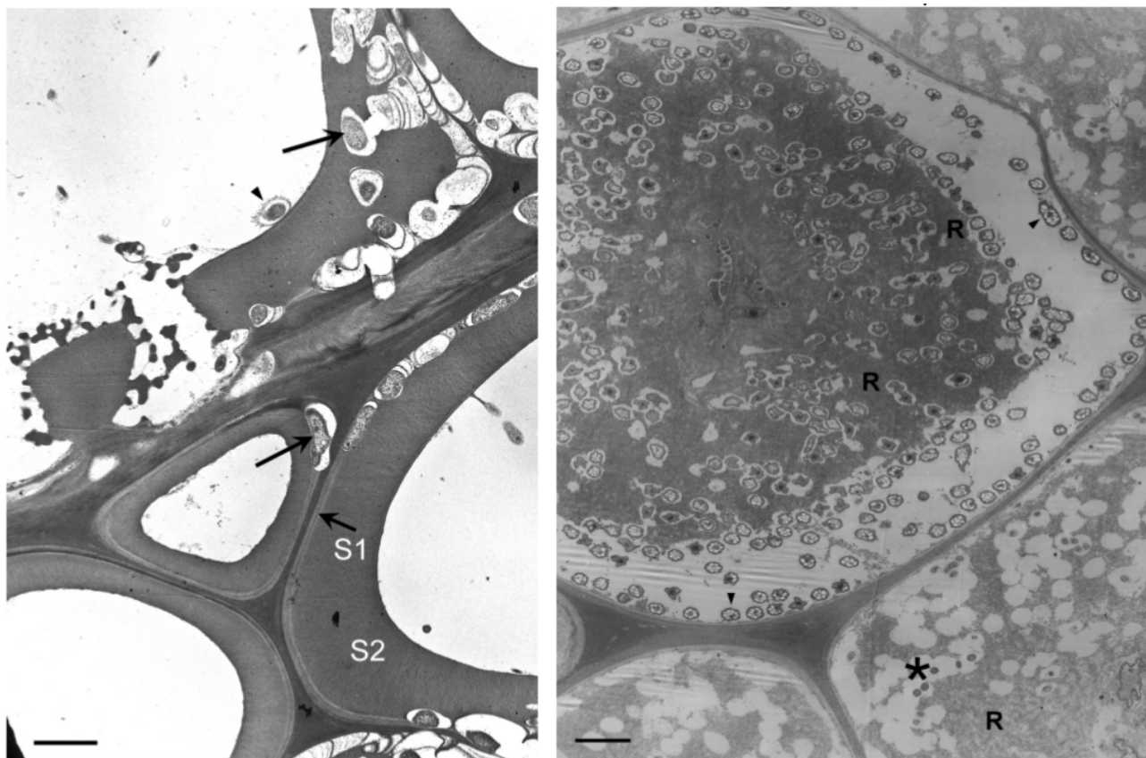
Figure 1.15. Transmission electron microscopy image of wood degraded by bacteria. Bar=2 \mu\text{m} . (Left) Fibre-tracheid walls in Alstonia scholaris wood attacked by tunnelling bacteria (arrows). Bacteria are present within S1 and S2 layers. The arrowhead points to a bacterium in close contact with the lumen face of the cell wall. (Right) Tracheid cell walls in Pinus sylvestris wood attacked by erosion bacteria (arrowheads), which are abundantly present along the cell wall and within cell wall residues (R) in one tracheid. Erosion bacteria are absent from other tracheids, which contain abundant cell wall residues and some scavenging bacteria (*) (from Singh 2007).
