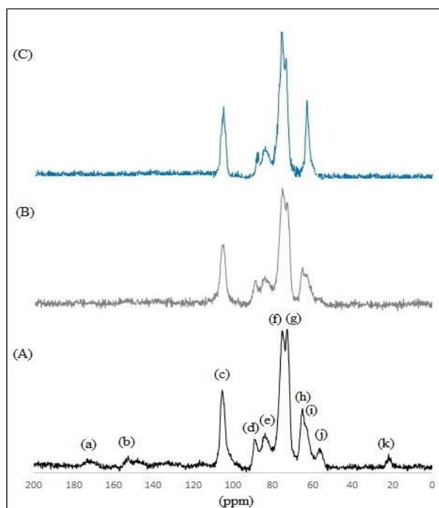
Figure IV.12. 13 C CP/MAS NMR spectra of miscanthus: (A) untreated, (B) pretreated with EDA-DMSO solution and (C) treated with DMIMMPh ionic liquid
