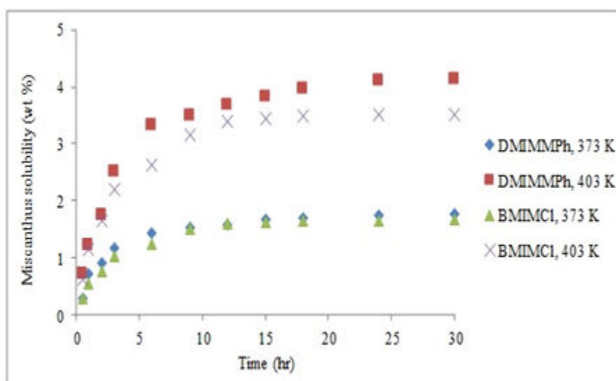
Figure IV.3. Effect of temperature on the miscanthus solubility in DMIMMPh and BMIMCl as a function of time at temperatures 373 and 403 K
