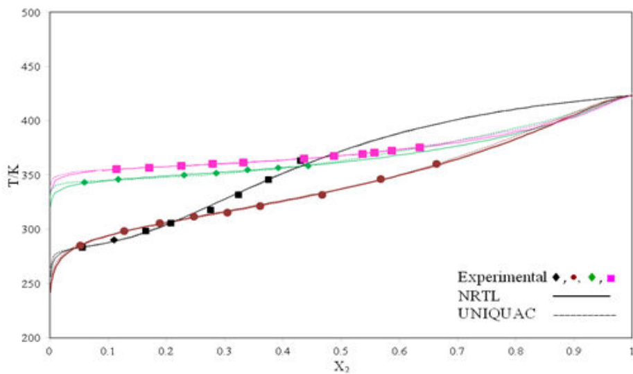
(a) Glucose
