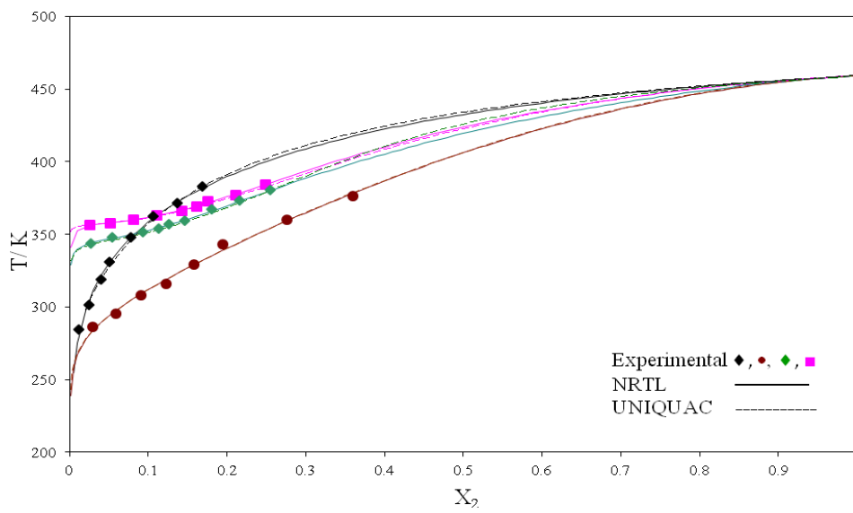
(c) Sucrose
