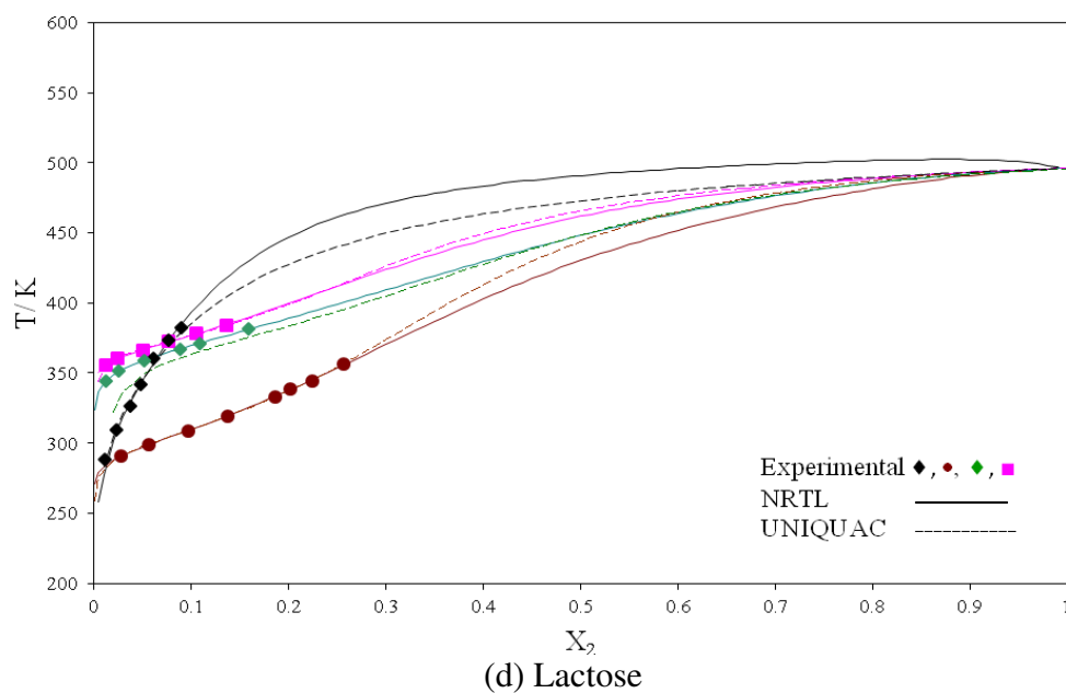
Figure II.1. Plot of the experimental and calculated SLE of {IL + sugar} binary systems: \blacklozenge EMIMSCN; \bullet DMIMMPh; \blacklozenge BMIMCl; \blacksquare EtOHMIMCl. The solid lines have been calculated using NRTL and UNIQUAC models with (a) Glucose, (b) Fructose, (c) Sucrose and (d) Lactose, where X_2 is the sugar mole fraction.
