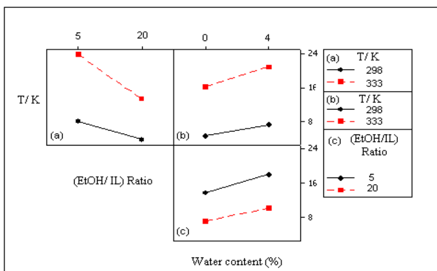
Figure II.7. The interaction between different variables on the solubility of glucose in a binary mixture of (BMIMCl + EtOH) at time 300 min.: a) at water content =2%, b) at EtOH/IL ratio by weight =12.5, c) at temperature =315.5 K.
