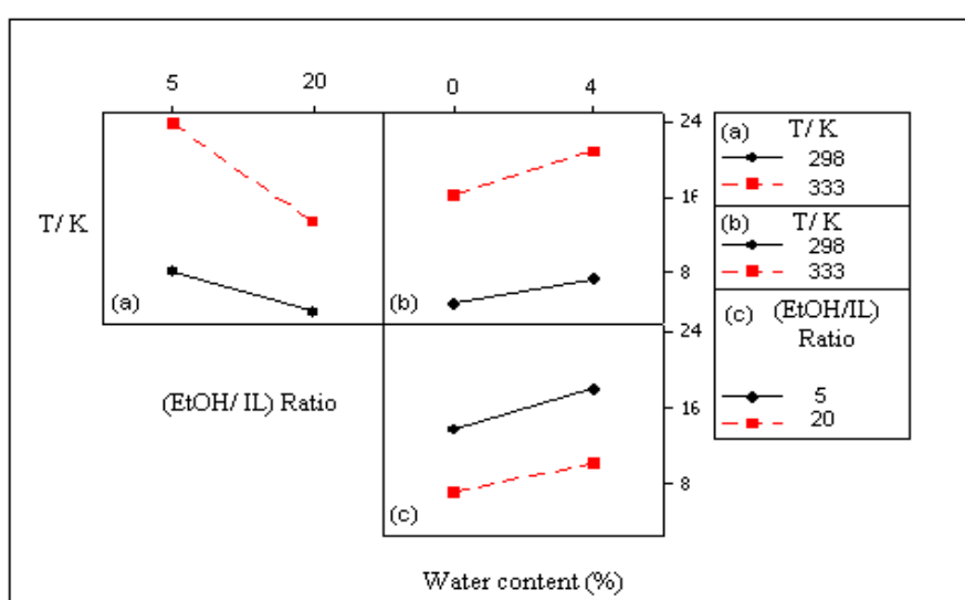
Figure II.7. The interaction between different variables on the solubility of glucose in a binary mixture of (BMIMCl + EtOH) at time 300 min.: a) at water content = 2%, b) at EtOH/IL ratio by weight = 12.5, c) at temperature = 315.5 K.
