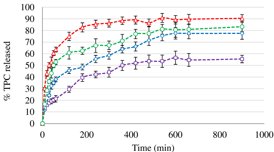
Fig. 3. TPC release from HPMC films enriched with 2% (v/v) B ( \Delta ), AC ( \diamond ), AC+B ( \circ ) and NRC ( \square ) compounds at 20°C.
