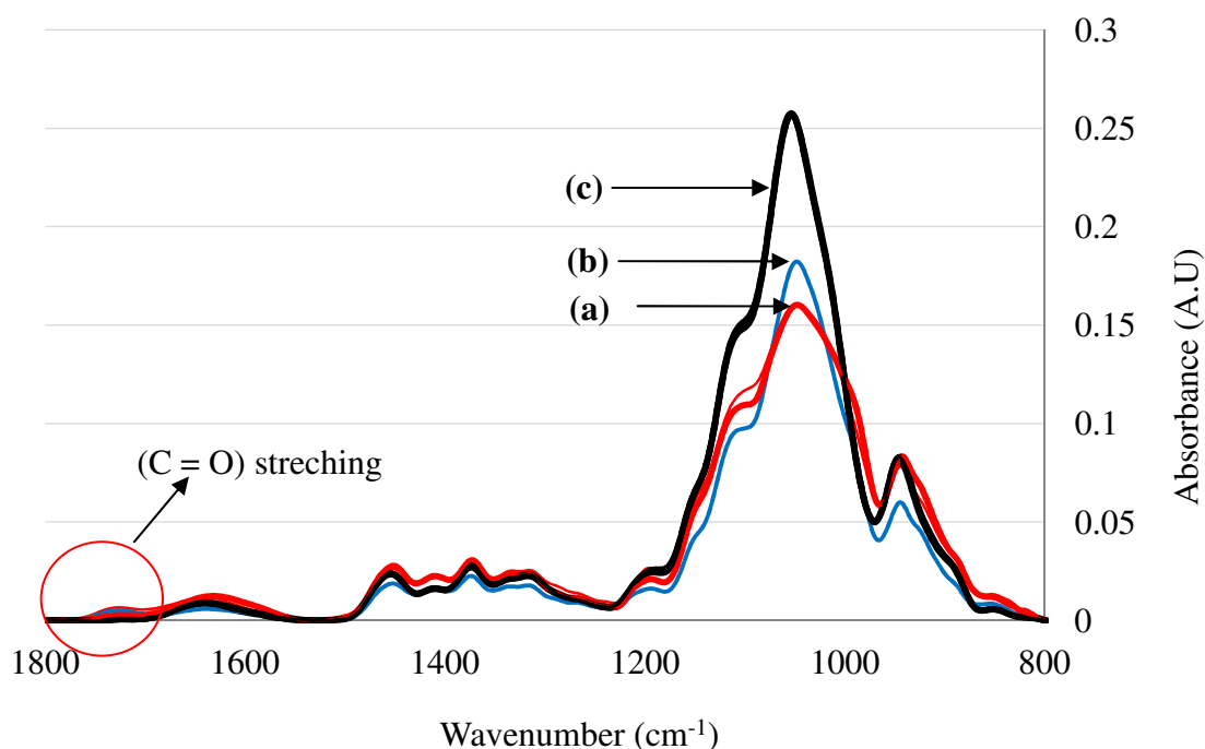
Fig. 6. FTIR spectra of HPMC films with 2% of each phenolic compound: (a) before release AC, B and (AC+B) films (b) before release NRC films (c) all film samples after release study.
