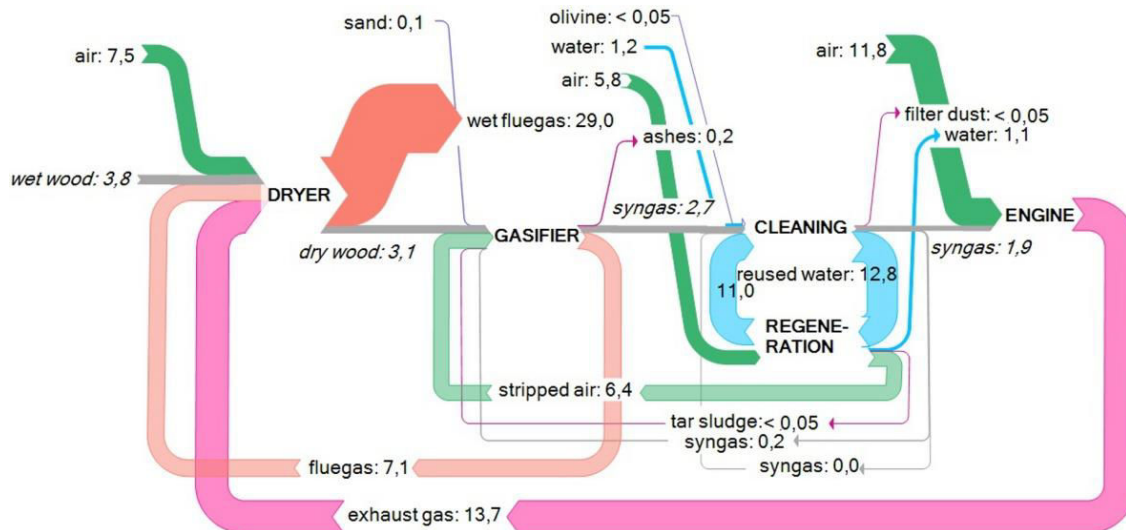
Figure A2- 3. Mass balance of the nominal wood gasification CHP system (mass flow streams in \text{kg s}^{-1} ).
