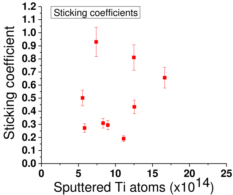
Fig. IV-7: Variation of the sticking coefficient as a function of Ti atoms sputtered during the deposition process.
