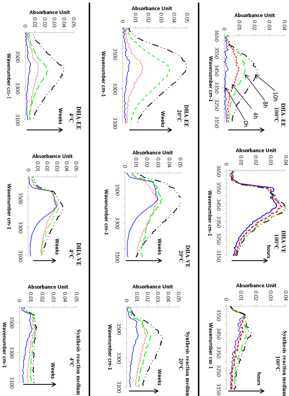
Fig. 4 Changes produced in the region between 3650 – 3100 \text{cm}^{-1} of the infrared spectrum of samples stored during 3 months. t=0 month —, t=1 month ·····, t=2 months — — and t=3 months — · · at 4°C & 20°C and of samples stored at 100°C t=0\text{h} —, t=4\text{h} ·····, t=8\text{h} — — and t=10\text{h} — · ·
