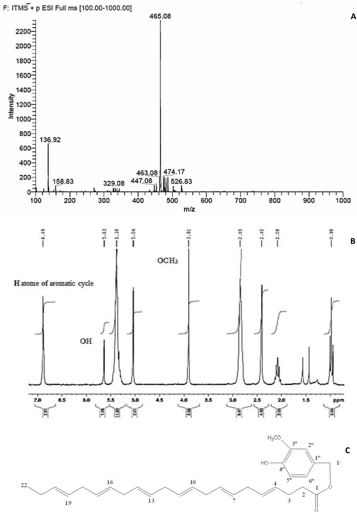
Figure 1: Structural characterization of DHA-VE. (A) MS analysis. (B) 1 H NMR analysis. (C) Deduced chemical structure.
