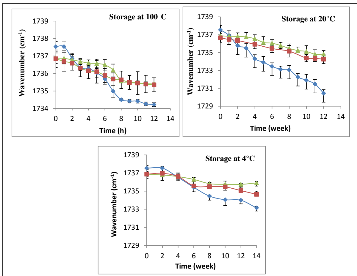
Fig.6. Evolution of wavenumber values of C=O band of DHA-EE \blacklozenge , Synthesis reaction medium \blacksquare and DHA-VE \blacktriangle under different oxidative conditions.
