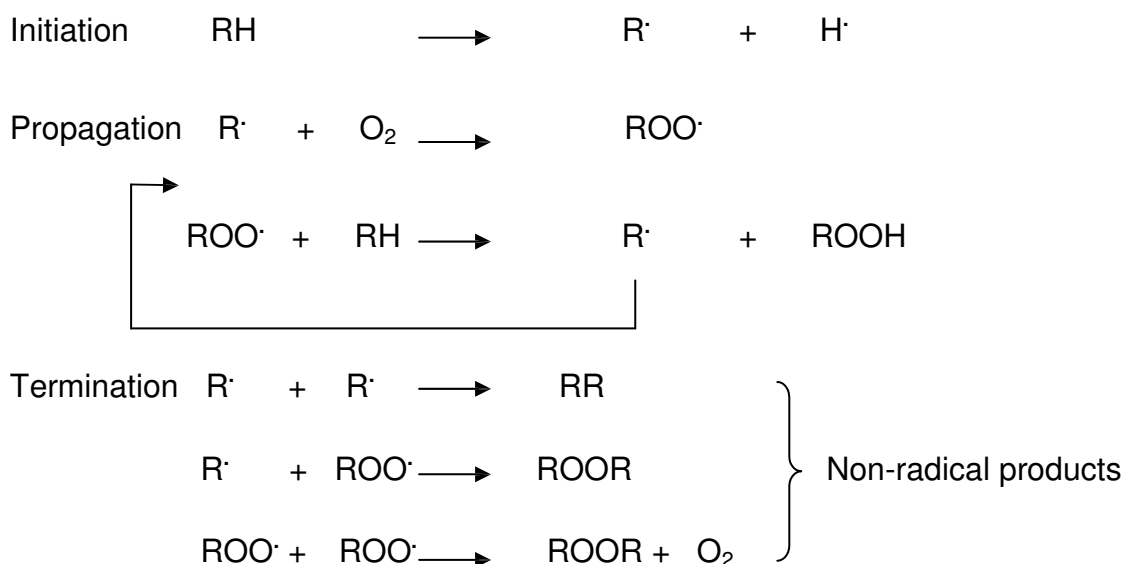
Figure 3. Autoxidation reaction, species identification is as follows: lipid (RH), Oxygen (O 2 ), free radicals, (R· and H·), peroxy radical (ROO·) and non-radical products (RR, ROOR), including hydroperoxides (ROOH).
