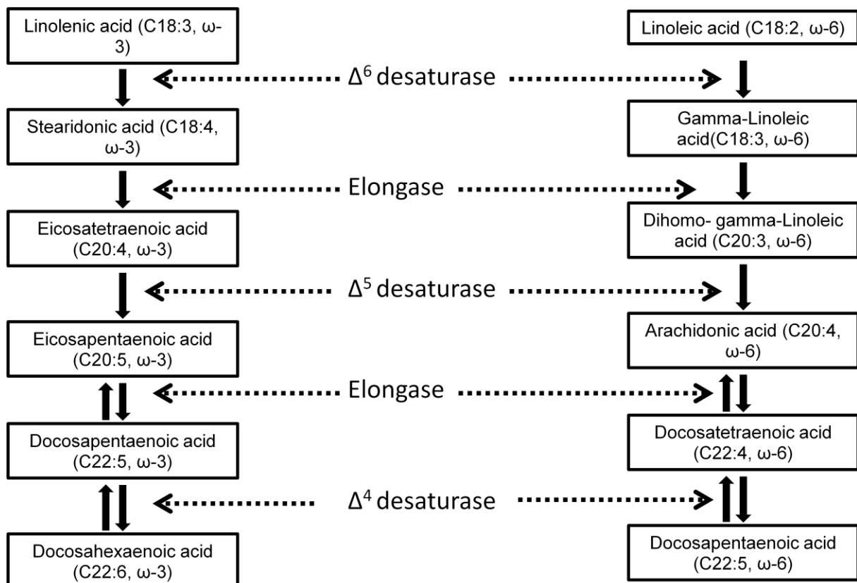
Figure 2. Desaturation and elongation pathway of \omega -3 and \omega -6 fatty acids.
