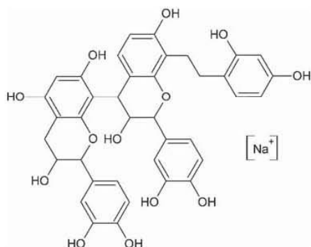
Figure 13 TRG1 polymer of 721Da (peak read at 721Da).
