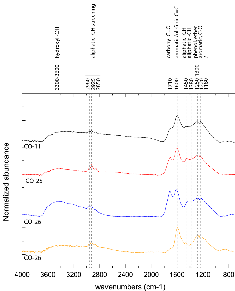
Figure 3.23: IR microspectroscopy spectra (Grenoble measurements) of Nebulotron CO samples (starting gas mixture CO only).
