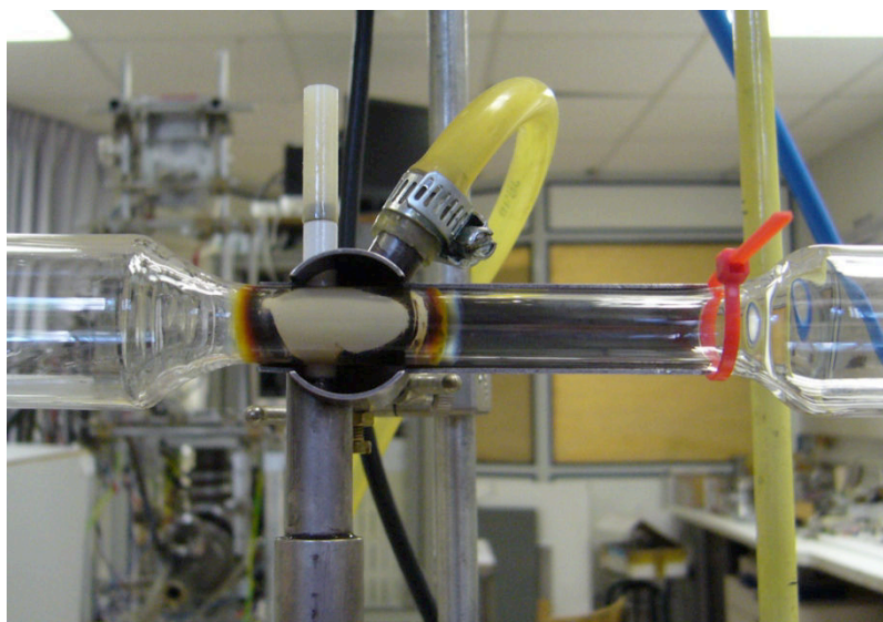
Figure 2.13. Picture of the Nebulotron reactor (new one) with the synthesized solids after a CO-N 2 experiment of 360 min, at 30W. The cavity length is 10 cm.
