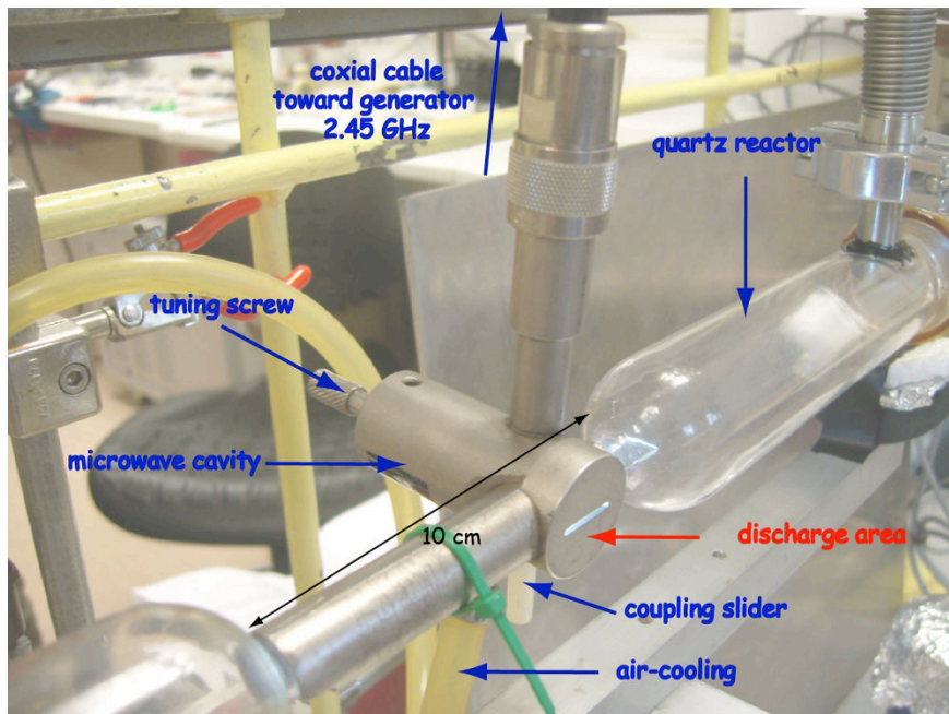
Figure 2.12. Microwave cavity onto the Nebulotron reactor.
