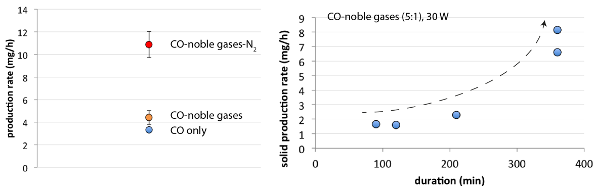
Figure 2.15. Solid production rate (mg/h) in the Nebulotron. Left: averages of samples produced in the same experimental conditions (360 min, 30 W) as a function of the initial gas mixture composition, for the new reactor. Right: for the CO-noble gases mixture (5:1, 30W) as a function of the experiment duration, on the old reactor.
