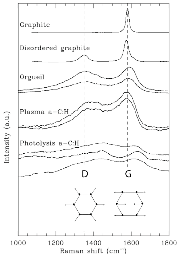
Figure 3.4. Raman spectra of (from top to bottom): (i) graphite; (ii) disordered graphite (G. Montagnac, data base of the ENS Lyon); (iii) carbonaceous fraction of the Orgueil meteorite; (iv) a-C:H produced in a hydrogen-dominated RF plasma; (v) UV photoproducted a-C:H from hexane and trans-2-butene precursors. The position of the G (for “graphitic”) and D (for “defect”) in (disordered) graphite are given by vertical dashed lines along with their vibration modes (adapted from Dartois et al., 2005 and Ferrari and Robertson, 2000).
