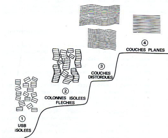
Figure 3.18: Progressive organization of carbon microtexture during heating treatment. When temperature rises, the BSU organization evolves toward a layered structure with less and less distortions. From Oberlin et al. 1984.
