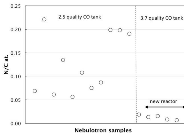
Figure 3.29. Evolution of the N/C ratio in Nebulotron samples as a function of production time. The CO gas tank change is marked on the graphic.
