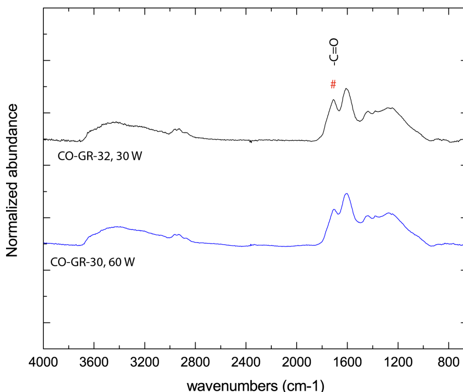
Figure 3.28. FTIR spectra of samples CO-GR-32 and CO-GR-30, produced at 30 W and 60 W respectively. The # symbol marks where the visible difference between the two spectra occurs at 1700\text{ cm}^{-1} .
