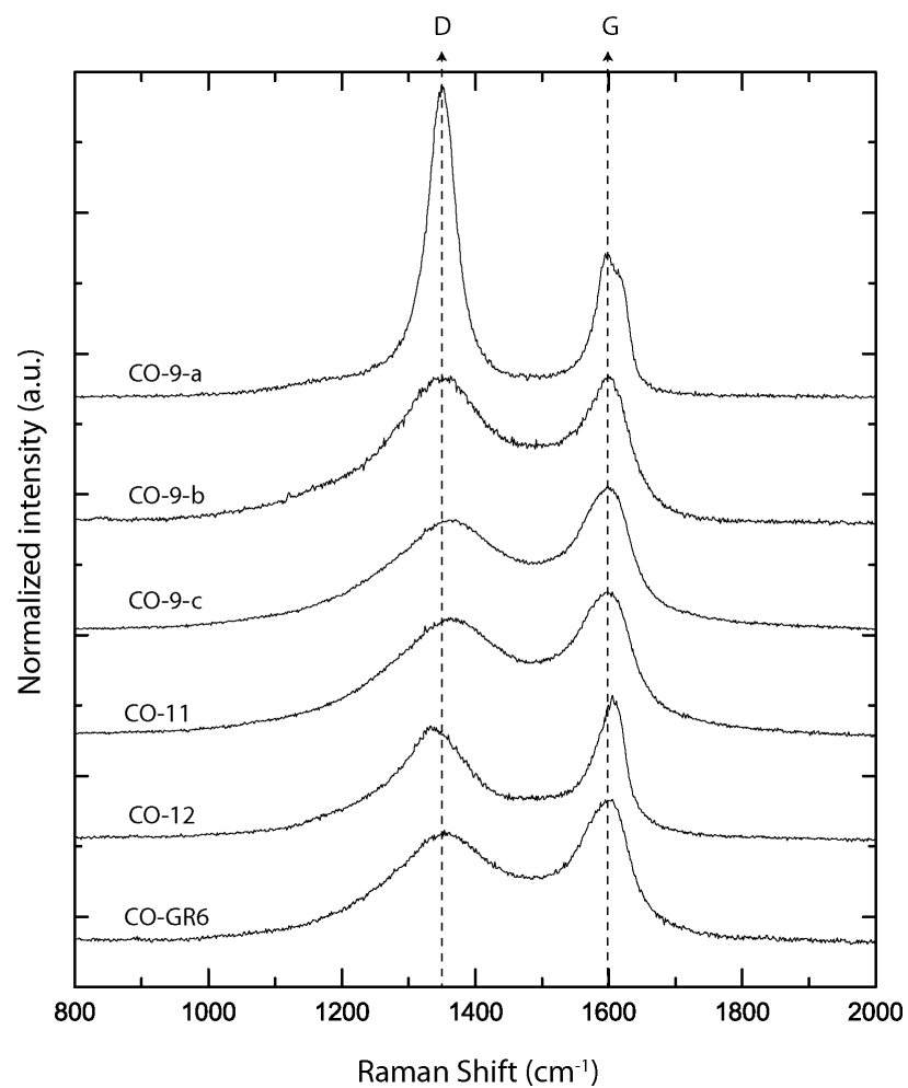
Figure 3.16. Representative Raman spectra of the Nebulotron samples analyzed at 514 nm. The baseline is subtracted and the intensity is normalized to the intensity of the G peak. The D and the G peak are materialized by the dote lines.
