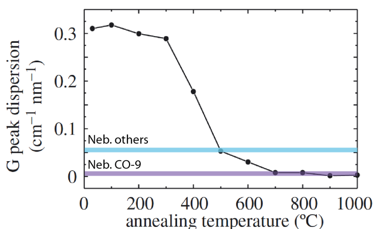
Figure 3.19: Empirical law between the G peak dispersion between 244 and 514 nm and the annealing temperature of hydrogenated amorphous tetrahedral carbons (ta-C:H, adapted from Ferrari and Robertson, 2001) along with the G peak dispersion between 244 and 514 nm for the Nebulotron samples.
