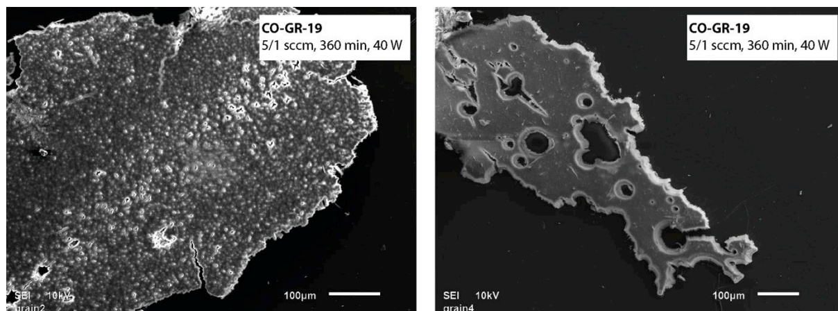
Figure 3.10. SEM pictures of red films synthesized in the Nebulotron.
