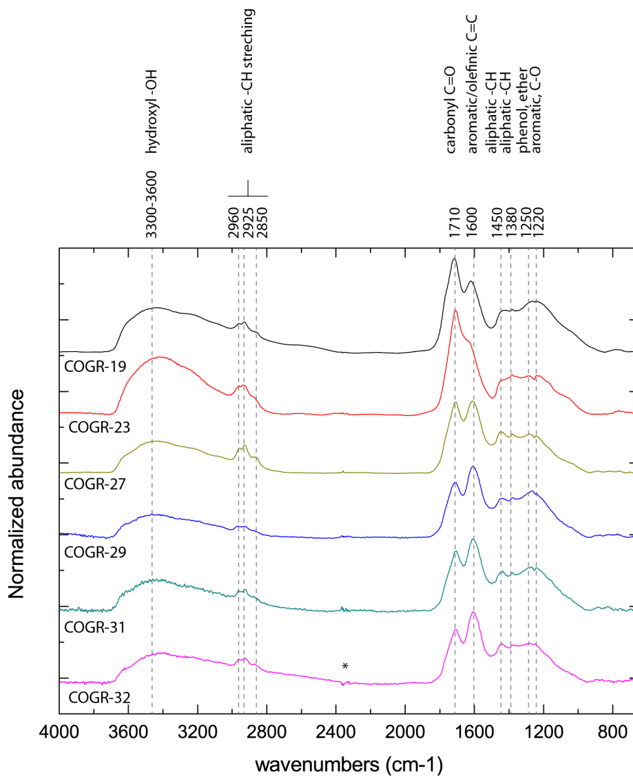
Figure 3.24. IR microspectroscopy spectra (Grenoble measurements) of Nebulotron CO-GR samples (starting gas mixture CO+Noble gases).
