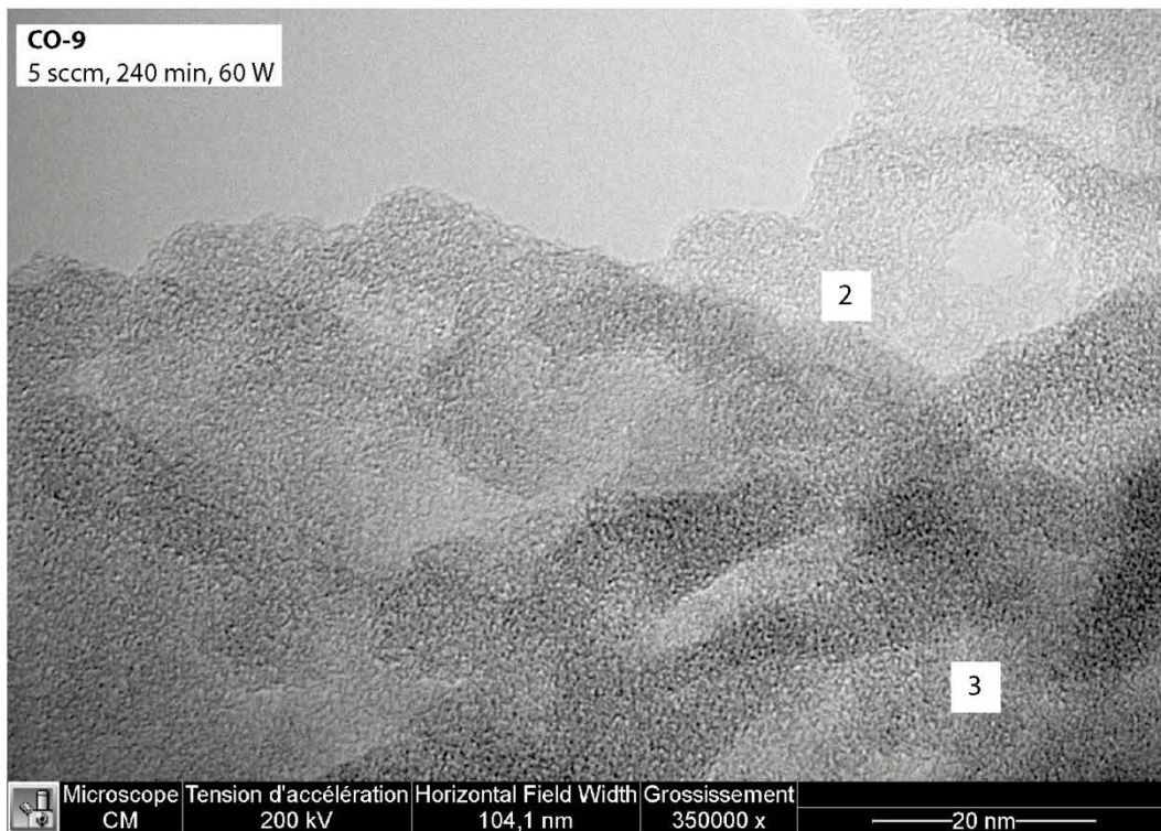
Figure 3.12. TEM pictures of Nebulon samples with 3 identified carbon microtextures: (1) microporous, (2) concentric and (3) amorphous.
