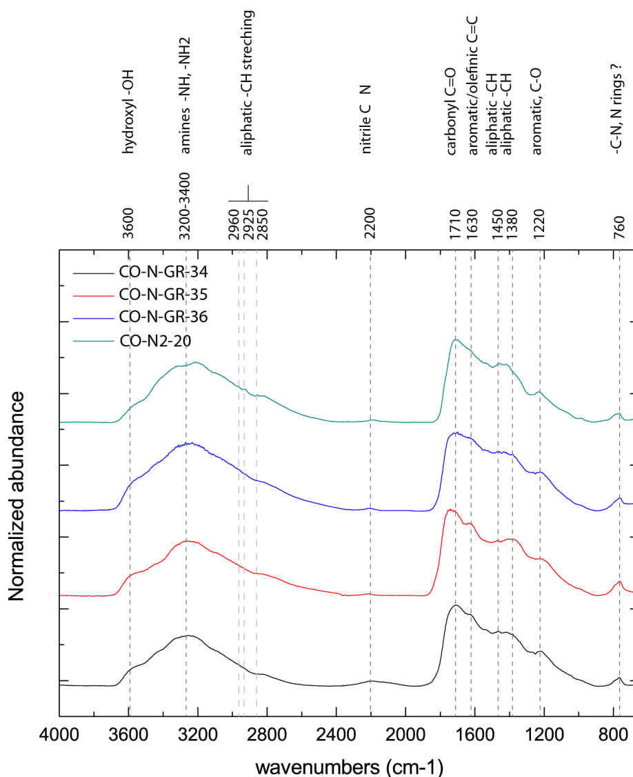
Figure 3.25. IR microspectroscopy spectra (Grenoble measurements) of Nebulotron CO-N-GR samples (starting gas mixture CO+N 2 +Noble gases, except for the CO-N 2 -20 sample, which was produced with a CO+N 2 gas mixture).
