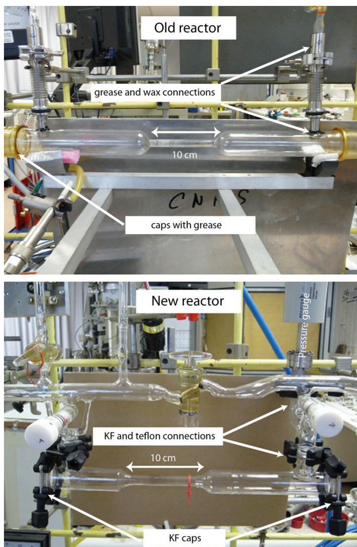
Figure 2.11. The Nebulotron old reactor vs. the new reactor.
