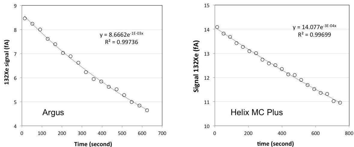
Figure 5.1. Signal of ^{132}\text{Xe} vs. time in an Argus (left) and in an Helix MC Plus (right) spectrometer (300 \mu\text{A} trap current). The signals are extrapolated to t=0 in order to account for gas consumption by ionization of the gas during measurement. One can note that the decrease of the signal is much more important in the Argus than in the Helix mass spectrometer, due to the low volume of the Argus one.
