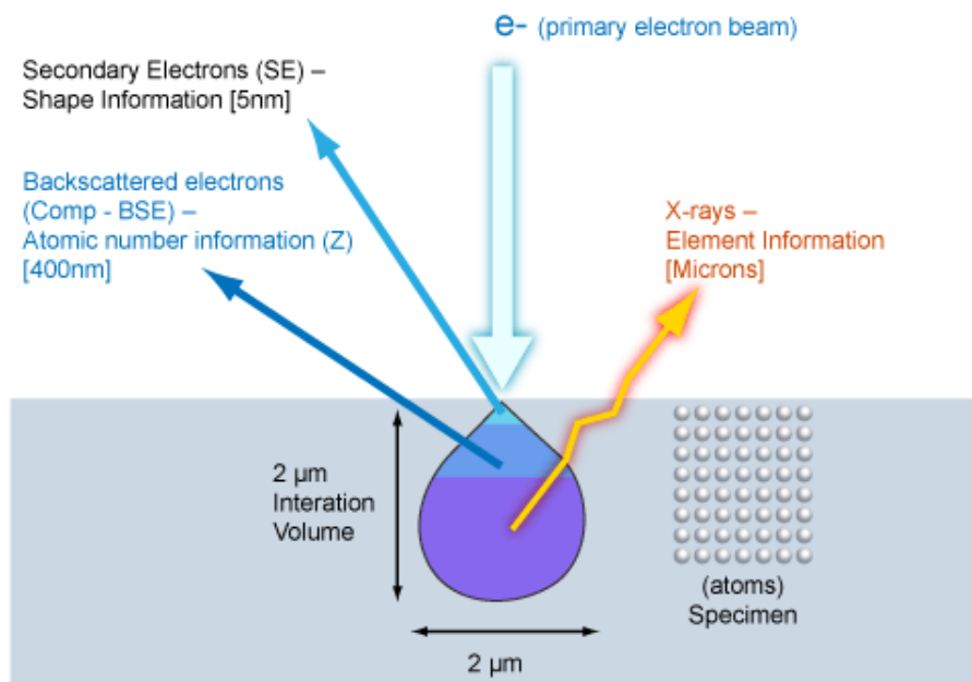
Figure 3.1. Electron-sample interaction volume, resulting in the emission of secondary and backscattered electrons and X-ray photons, used by SEM technique.
