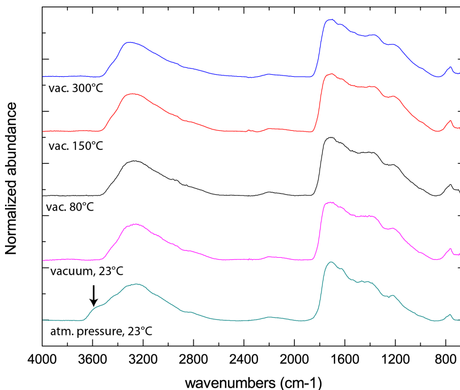
Figure 3.26: Spectral evolution of the sample CO-N-GR34, from atmospheric pressure to vacuum, and then from room temperature to 300°C under vacuum. The black arrow shows the disappearing of the absorption at \sim 3600\text{ cm}^{-1} when the sample is put under vacuum, likely due to \text{H}_2\text{O} desorption.
