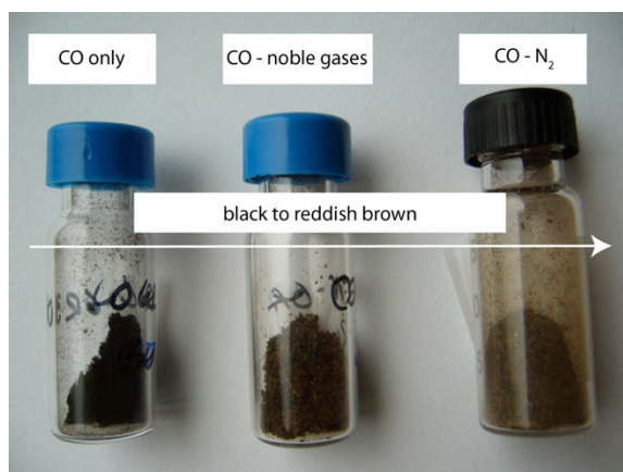
Figure 2.14. Different synthesized samples depending on the initial gas mixture composition.
