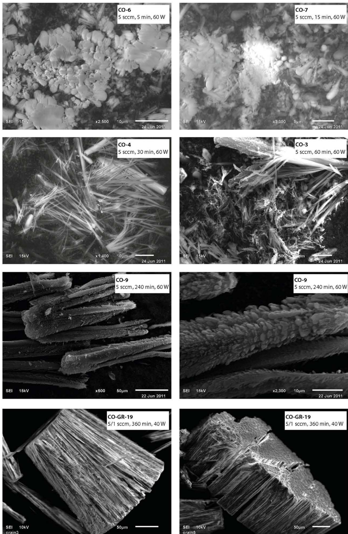
Figure 3.9. Various morphologies of dark grains (SEM pictures).
