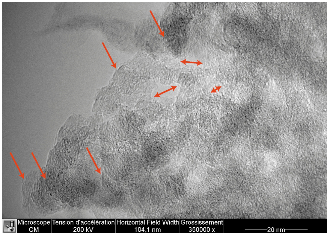
Figure 3.14. TEM picture showing a concentric carbon microtexture observed in Nebulotron sample CO-Ar-1.
