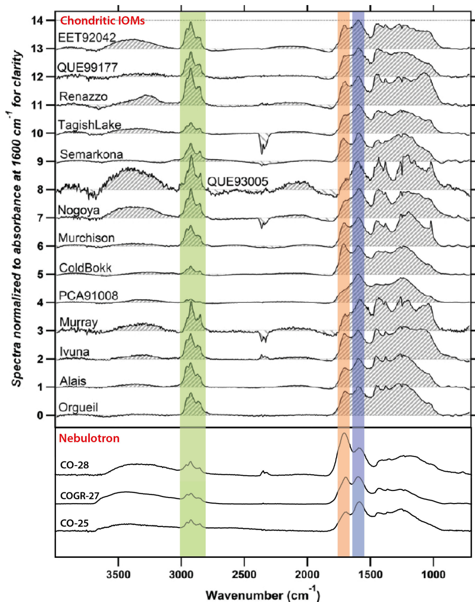
Figure 3.31. FTIR spectra of chondritic IOMs (adapted from Orthous-Daunay et al., 2013) and of three Nebulotron samples (CO25, COGR27 and CO28). Those Nebulotron samples display spectra qualitatively closer to spectra of IOMs than the other samples. The spectral domains that are highlighted are: alkyl ( \text{CH}_3 , \text{CH}_2 , green ), carbonyl ( \text{C}=\text{O} , orange ) and aromatic (aromatic \text{C}=\text{C} , blue ) functional groups.
