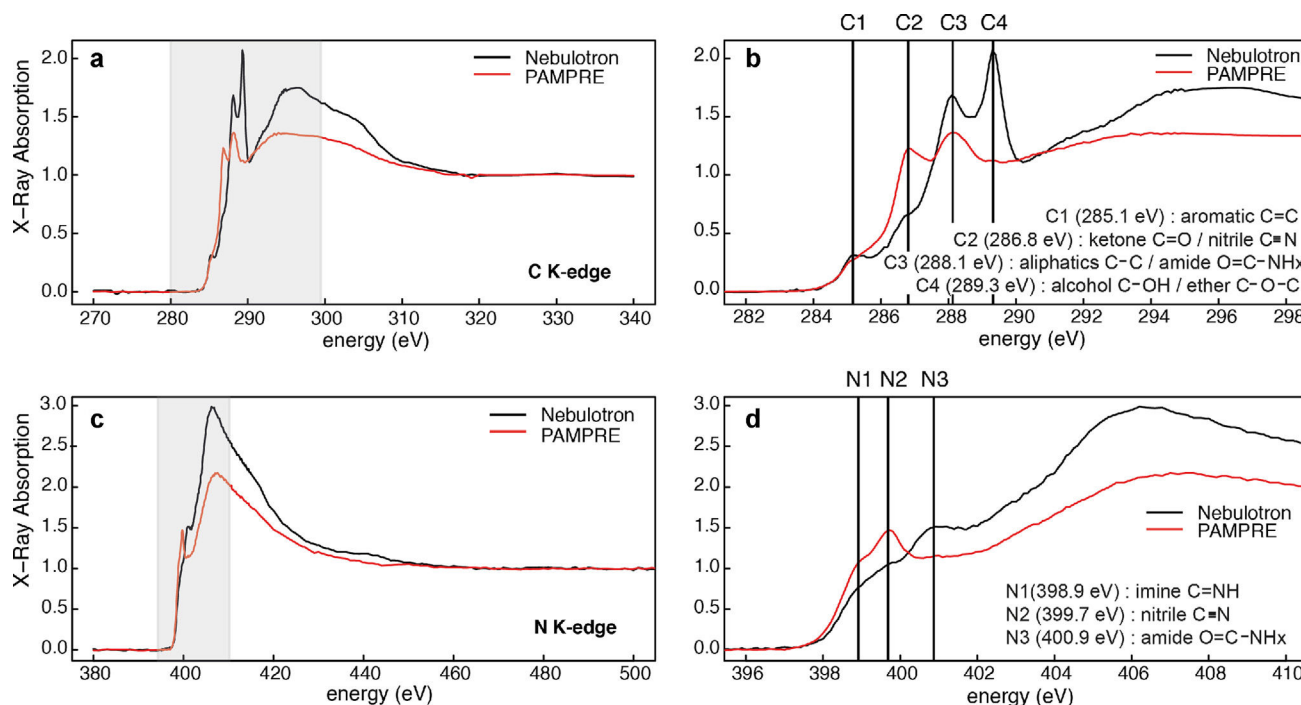
Fig. 3. XANES spectra and band assignment in the C and N K-edges ((a) and (c) respectively) of the PAMPRE (5% initial \text{CH}_4 ) and Nebulotron aerosols. (b) and (d) are a zoom of the shaded area in the (a) and (c) plots respectively.
