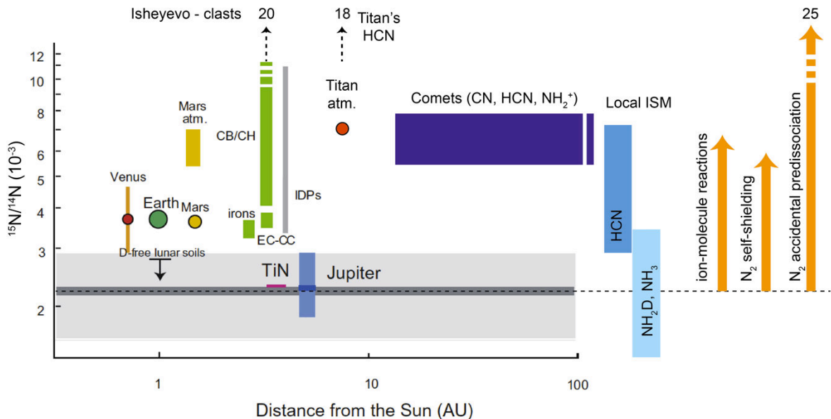
Figure 1.11. Nitrogen isotope variations in solar system reservoirs as a function of the distance from the Sun. The dark gray line (“Solar”) is the ^{15}\text{N}/^{14}\text{N} ratio determined in the Genesis targets (Marty et al., 2011, Marty et al., 2010), and the light gray area represents its 2\sigma uncertainty. The magnitude of nitrogen isotopic fractionation resulting from ion-molecule reactions, \text{N}_2 self-shielding and \text{N}_2 accidental predissociation are shown for comparison. The figure is adapted from Marty et al., 2010. Data come from Marty et al., 2010 and references therein, Rousselot et al., 2014, Niemann et al., 2010, Vinatier et al., 2007, Hily-Blant et al., 2013, and references therein. Fractionation models: Terzieva and Herbst, 2000, Lyons et al., 2009, Chakraborty et al., 2013.
