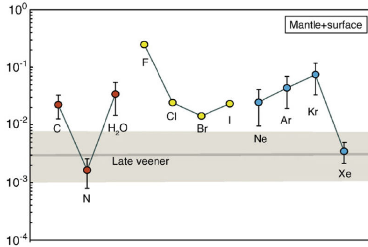
Figure 1.13. Terrestrial composition of volatile elements in Earth for the mantle and atmospheric reservoirs (from Marty, 2012). Abundances are normalized to the mass of the Earth and to the abundances in chondrites.
