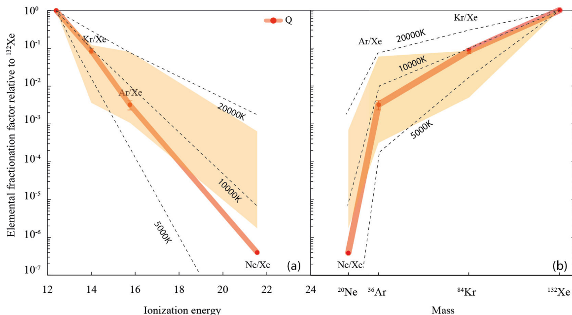
Figure 5.21. Calculated ionic abundance pattern of noble gases at three electron temperatures (5000, 10000 and 20000 K). The red line indicates the average for Q (Busemann et al., 2000) and the shaded orange area indicates the range obtained from plasma experiments (see Fig. 5.18). (a) plotted vs. ionization energy, and (b) plotted vs. mass.
