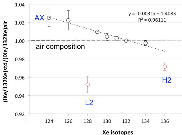
Figure 5.3. Example of the instrumental mass fractionation in the Helix MC Plus for Xe standards of atmospheric isotopic composition (average and standard deviation of 60 standard aliquots). The black circles represent the Xe isotopes measured on the Ax SEM. The red circles ( ^{128}\text{Xe} and ^{136}\text{Xe} ) represent the isotopes measured on the other SEM, L2 and H2 detectors, respectively. The regression line through the “Ax isotopes” illustrates the mass fractionation from the true value (i.e. air) relative to the measured one, which is of the order of -3\text{‰}/\text{amu} . The isotopes measured on other SEM collectors fall off this mass fractionation line.
