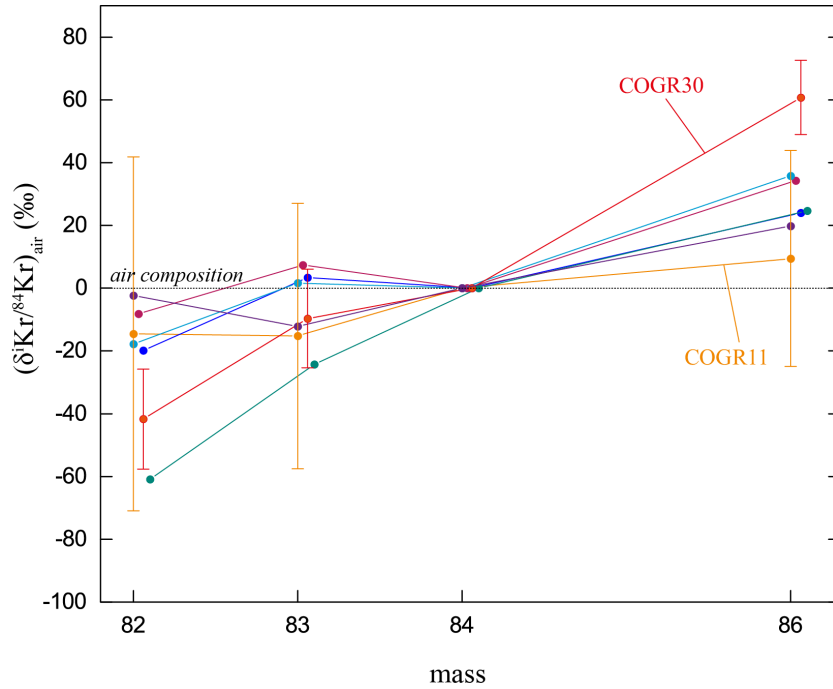
Figure 5.10. Krypton isotopic compositions in the Nebulotron samples. The points are slightly shifted along the mass axis for visibility. Error bars ( 1\sigma ) are shown for two samples only for clarity.
