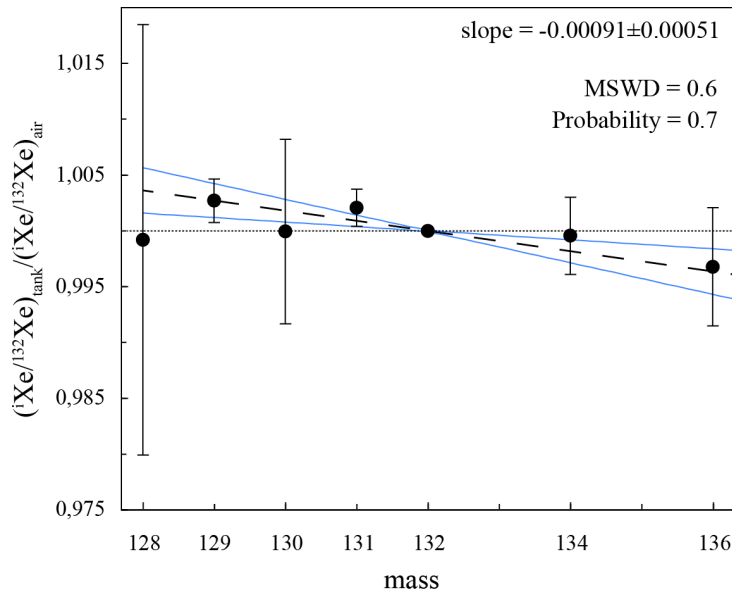
Figure 5.7. Xe isotopic composition of the gas tank (black dots) relative to the Xe standard ( ^{132}\text{Xe}=1 ) as a function of mass. Error bars are 2\sigma . The regression line and its 2\sigma envelope are shown. The dotted line represents the air composition ( \equiv 1 , unfractionated).
