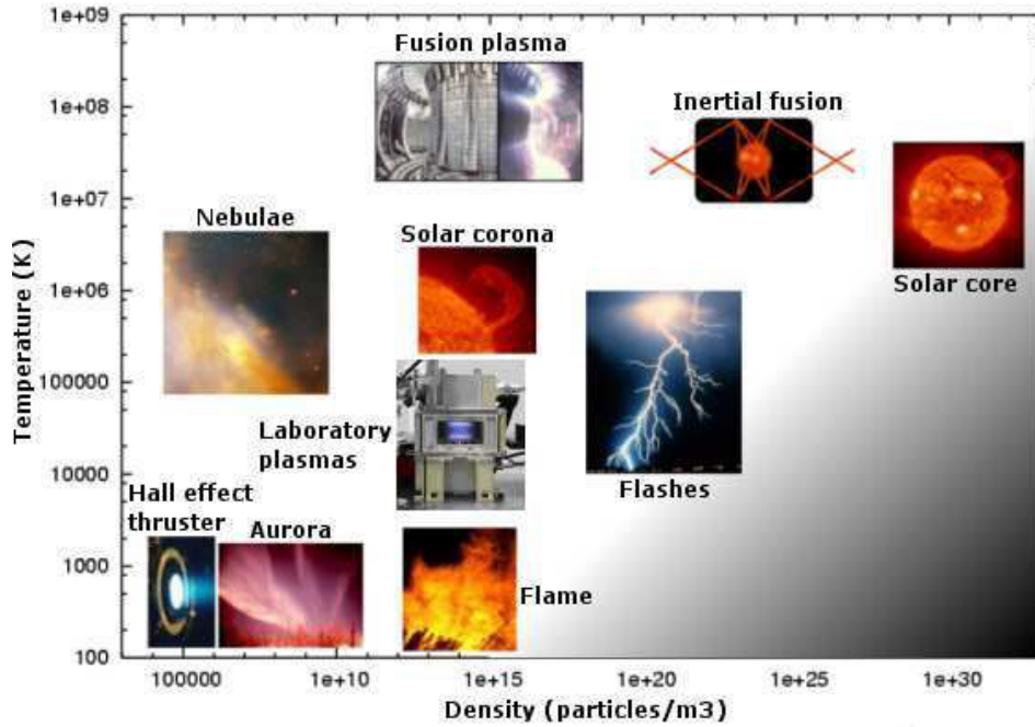
Figure 2.1. Space, natural and laboratory plasma electron temperature and densities.
