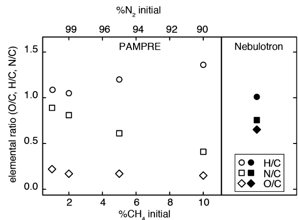
Fig. 2. Elemental composition of the PAMPRE (open symbols) and Nebulotron (filled symbols) experiments. Elemental ratios of the PAMPRE aerosols are presented as a function of the initial CH 4 concentration in the gas mixture (data from Sciamma-O'Brien et al., 2010). Error bars are smaller than the symbol sizes.
