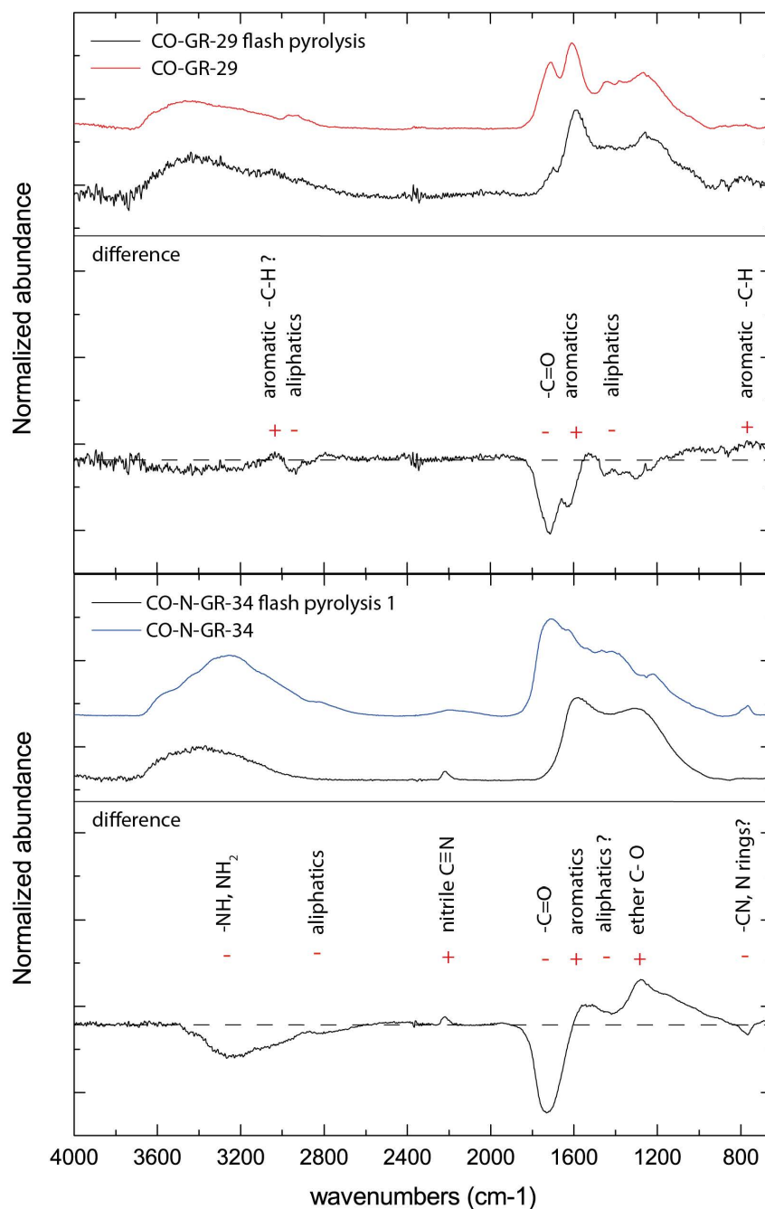
Figure 3.27. FTIR spectra of the CO-GR29 (top) and CO-N-GR34 (bottom) samples before and after the 1200^{\circ}\text{C} flash heating, and the calculated difference between the two. Minus signs mark the disappearance/intensity decrease of some bands, whereas the plus signs mark the appearance/intensity increase of other bands.
