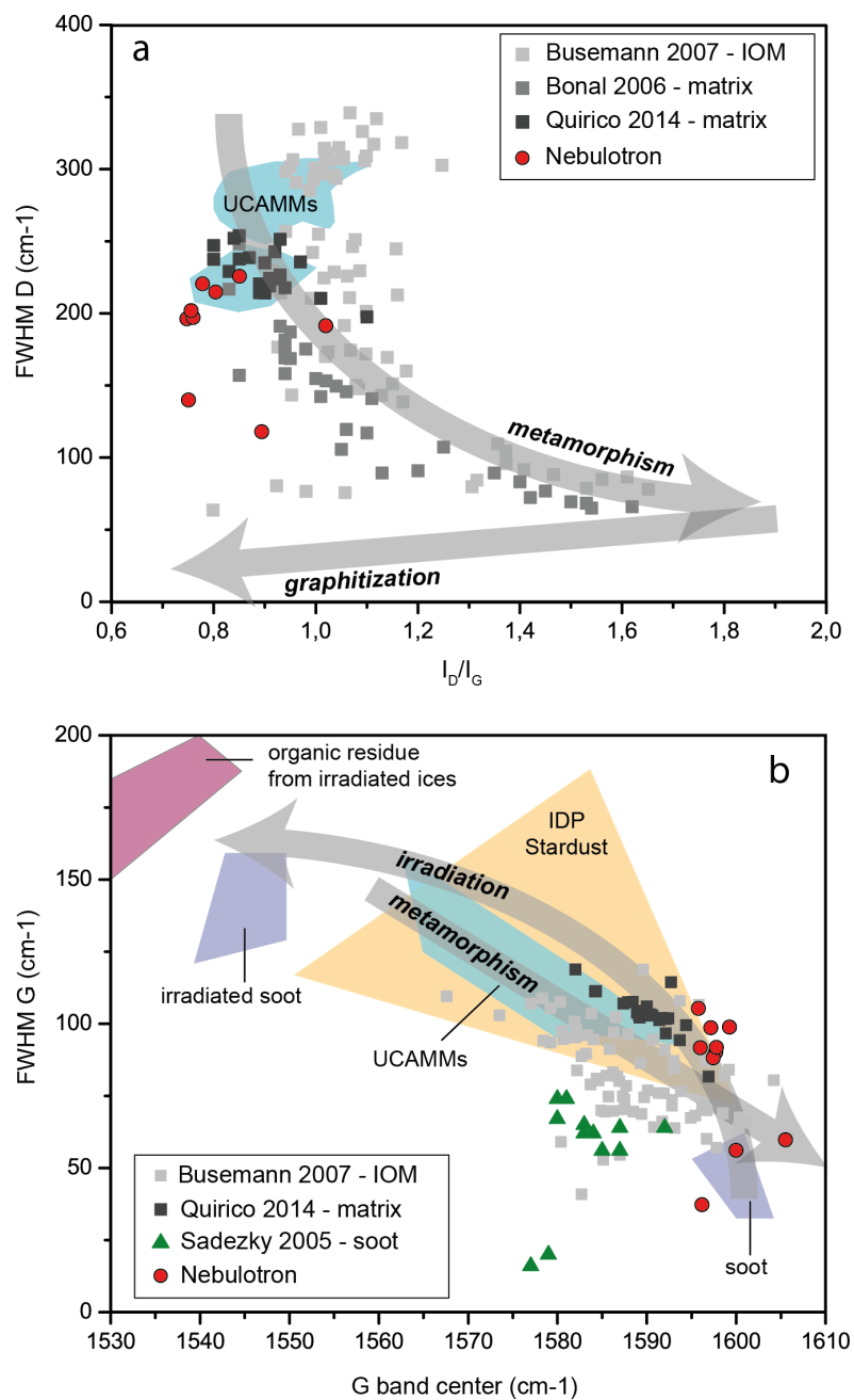
Figure 3.33. Comparison of 514 nm Raman spectral parameters of Nebulotron samples with those of organics from cosmomaterials. Chondrites: matrix (Bonal, 2006, Quirico et al., 2014), and extracted IOMs (Busemann et al., 2007). Antarctic micrometeorites (UCAMMs, blue area: Dartois et al., 2013, Dobrică et al., 2011). IDPs and Stardust grains (orange area: Quirico et al., 2005, Rotundi et al., 2008, Sandford et al., 2006). Laboratory soot (green triangles: Sadezky et al., 2005, purple area: Brunetto et al., 2009). Irradiated organic materials (soot: Brunetto et al., 2009, organic residue from irradiated ices: Baratta et al., 2004). (a) FWHM-D vs. I_D/I_G and (b) FWHM-G vs. w_G . The grey arrows illustrate the evolution of the Raman spectral parameters with metamorphism and irradiation with high energy ions (keV) (Bonal et al., 2006, Brunetto et al., 2009, Busemann et al., 2007).
