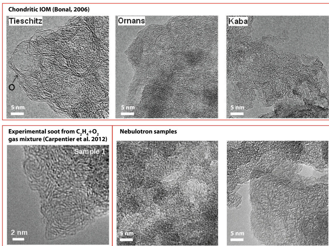
Figure 3.32. TEM observations of carbon textures in chondritic IOMs (Bonai, 2006), in an experimental soot formed in a flame composed of C_2H_4 and O_2 (Carpentier et al., 2012) and in Nebulotron samples.
