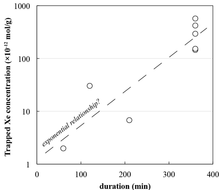
Figure 5.14. Trapped Xe concentrations in the Nebulotron samples as a function of the duration of the experiments.
