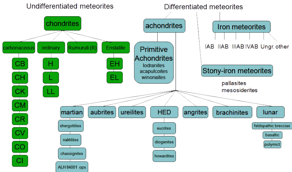
Figure 1.7. Classification of meteorites (credits: NASA).
