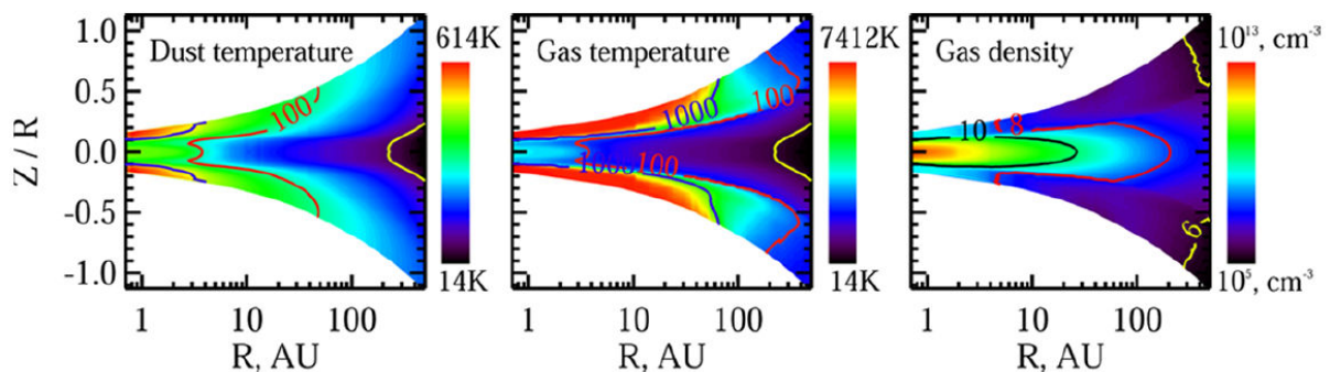
Figure 1.2. Calculated radial and vertical profiles of the dust temperature (left), the gas temperature (middle) and the gas density (right). The high values are marked by red color whereas the low values are marked by dark blue/black colors (from Henning and Semenov, 2013).
