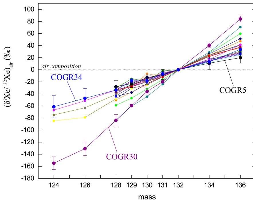
Figure 5.9. Xenon isotopic composition in Nebulotron samples (in \delta notation). Uncertainties ( 1\sigma ) are listed for samples COGR5, COGR34 and COGR30. Uncertainties for other samples are similar but not shown for visibility.
