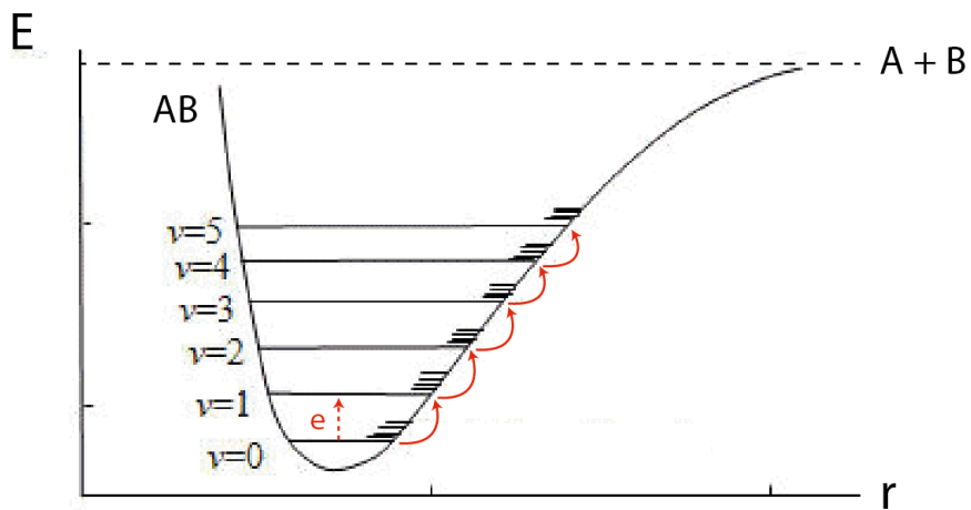
Figure 2.4. Dissociation by resonant V-V energy transfer.
