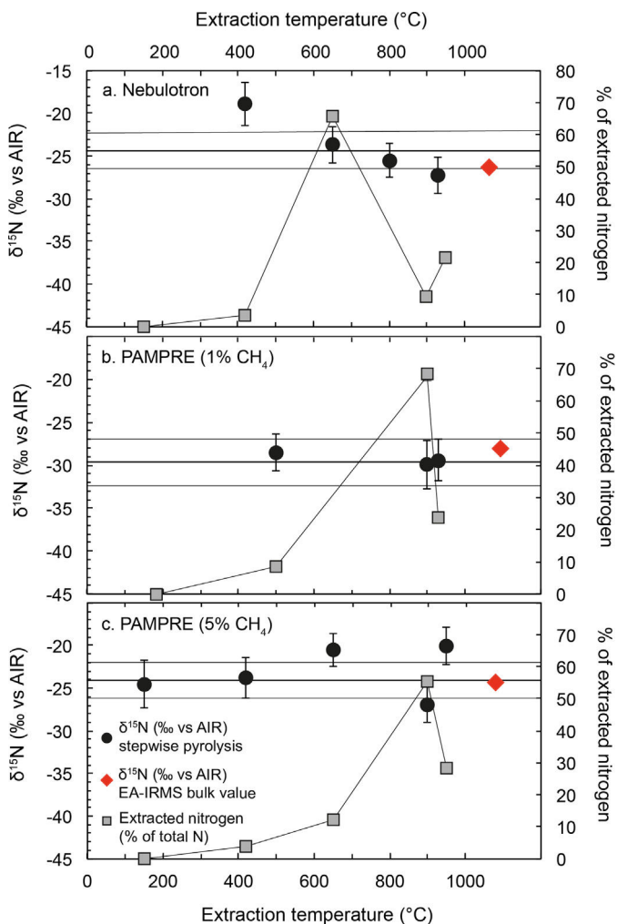
Fig. 5. Nitrogen isotopic composition (δ 15 N in ‰, left axis, dark circles) and quantity of released nitrogen (in % of total nitrogen extracted, right axis, gray squares) as a function of pyrolysis temperature of the Nebulotron and the PAMPRE aerosols. Solid lines: weighted average and standard deviation of the nitrogen isotopic ratios over all extraction steps. Red diamonds: EA-IRMS bulk δ 15 N measurements (error bars (1σ) are smaller than the symbol size).
