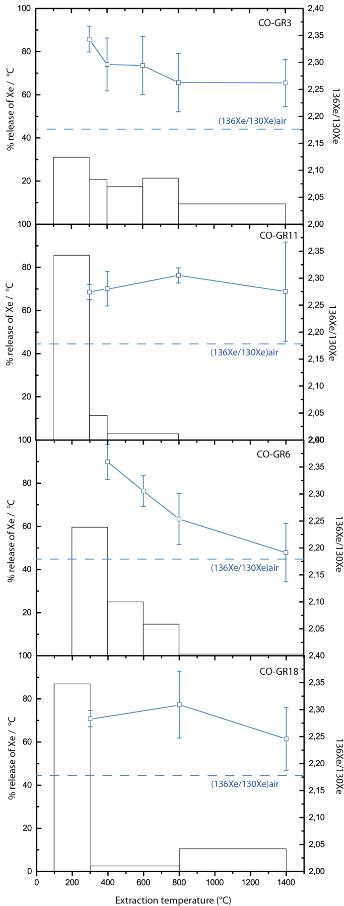
Figure 5.16. Thermal release patterns for ^{130}\text{Xe} in four Nebulotron samples, expressed in % of released gas normalized to °C. ^{136}\text{Xe}/^{130}\text{Xe} ratios and their 1 sigma uncertainties are shown for each step.
