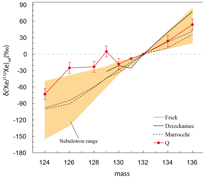
Figure 5.18. Xe isotopic composition in Q (average of all chondrites measured by Busemann et al., 2000) as well as in different plasma experiments: this study, Frick et al., 1979, Dzizckanec et al., 1981 and Marrocchi et al., 2011. The delta notation is used and the ratios are normalized to ^{132}\text{Xe} and to the solar wind composition for Q (Meshik et al., 2014) and to air for the plasma experiments. The orange shaded area represents the range of Xe isotopic compositions obtained in the Nebulotron experiment. Typical errors ( 1\sigma ) on deltas are shown for Q only for visibility.
