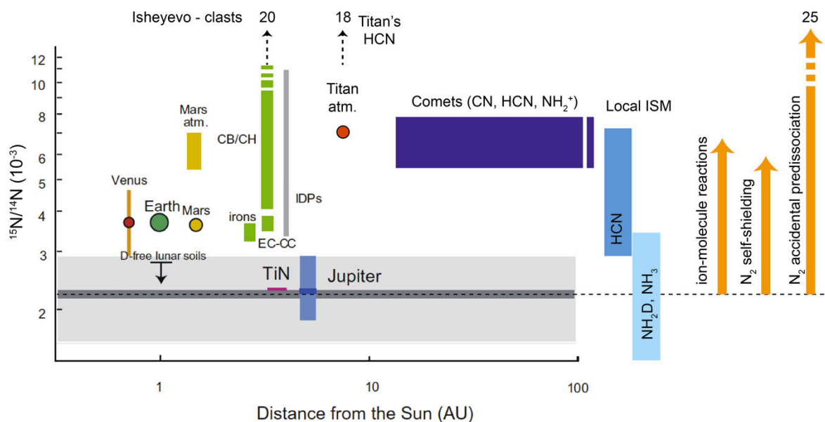
Figure 1.11. Nitrogen isotope variations in solar system reservoirs as a function of the distance from the Sun. The dark gray line (“Solar”) is the ^{15}\text{N}/^{14}\text{N} ratio determined in the Genesis targets (Marty et al., 2011, Marty et al., 2010), and the light gray area represents its 2\sigma uncertainty. The magnitude of nitrogen isotopic fractionation resulting from ion-molecule reactions, \text{N}_2 self-shielding and \text{N}_2 accidental predissociation are shown for comparison. The figure is adapted from Marty et al., 2010. Data come from Marty et al., 2010 and references therein, Rousselot et al., 2014, Niemann et al., 2010, Vinatier et al., 2007, Hily-Blant et al., 2013, and references therein. Fractionation models: Terzieva and Herbst, 2000, Lyons et al., 2009, Chakraborty et al., 2013.
