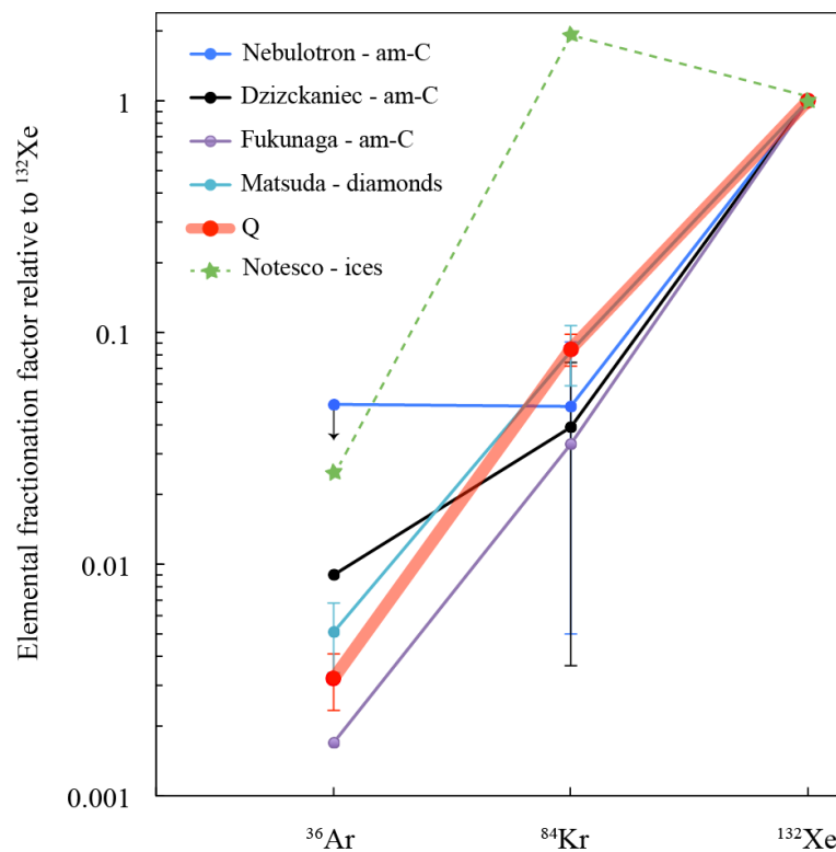
Figure 5.17. Elemental abundances patterns for Xe, Kr and Ar in Q (average of chondrites measured by Busemann et al., 2000) and in ion-implantation experiments (this study, Dzizckaniec et al., 1981, Fukunaga and Matsuda, 1997, Matsuda et al., 1991). The fractionation factor is defined in the text. The solar composition is taken as the reference for the Q-gases. The upper limit for ^{36}\text{Ar}/^{132}\text{Xe} in the Nebulotron samples is shown by the arrow. For comparison, data from noble gas trapping in water ices are shown (Notesco et al., 2003). am-C stands for amorphous carbon.
