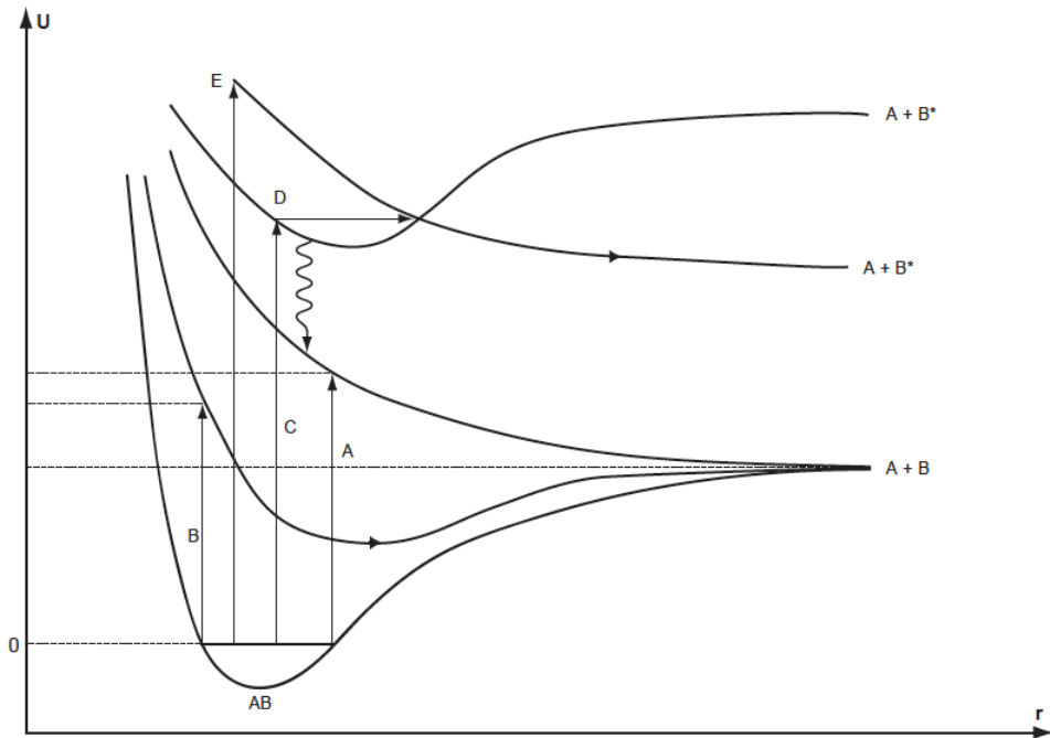
Figure 2.3. Different mechanisms of molecular dissociation through electronic excitation (from Fridman, 2008).
