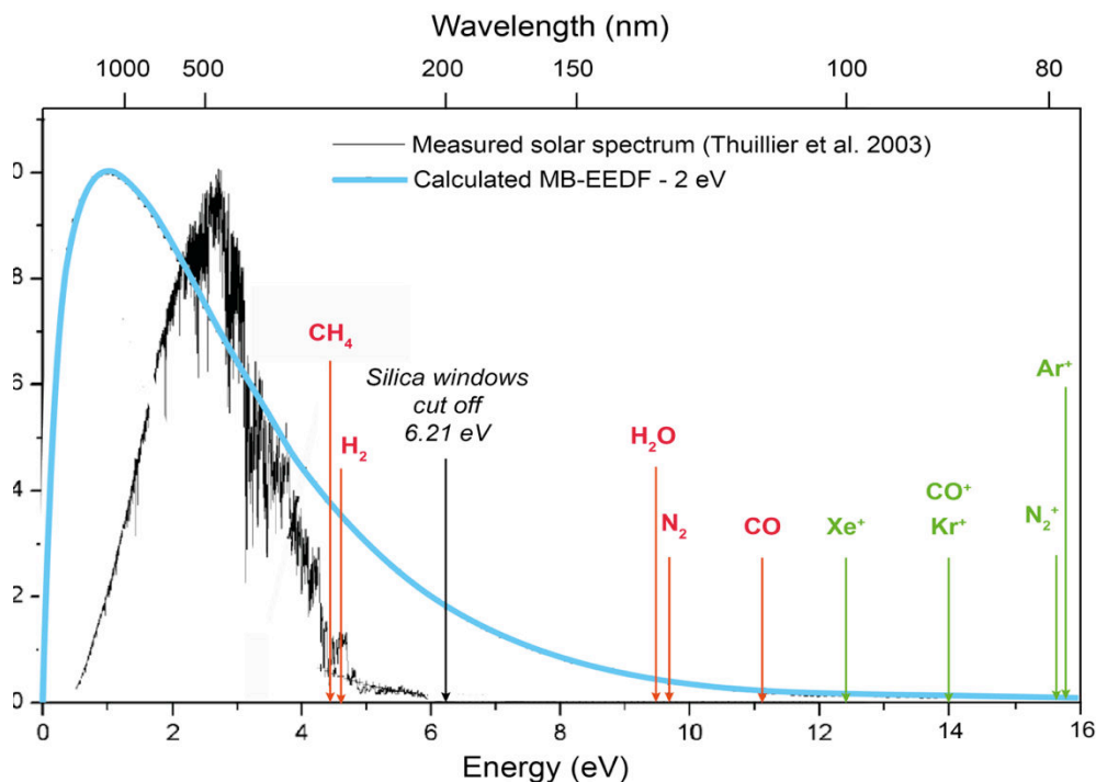
Figure 2.7. Example of a Maxwellian EEDF (blue curve) along with the dissociation (red) and ionization (green) energies of atoms and molecules of interest for this study. For a comparison of shapes and relative intensities as a function of energies, the solar spectrum is given. Adapted from Szopa et al., 2006.
