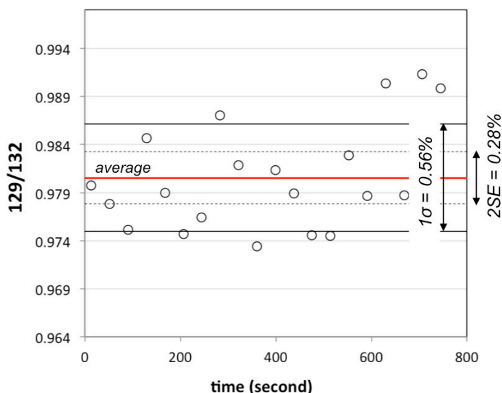
Figure 5.2. Example of the determination of the raw ^{129}\text{Xe}/^{132}\text{Xe} ratio by calculating the isotope ratios averaged over all cycles. \sigma = standard deviation = \sqrt{\frac{1}{N-1} \sum_1^n (x_i - \bar{x})^2} ; SE = standard error = \frac{s}{\sqrt{n}} (where n is the number of measurements, here the number of cycles). In this case, the 95% confidence interval on the average value is 0.28% (2 SE). Each point represents the isotopic ratio determined for one cycle.
