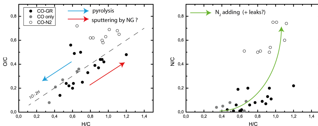
Figure 3.22. Atomic ratios O/C (left) and N/C (right) ratios as a function of H/C ratio for the Nebulotron samples. The arrows illustrate the evolution of the elemental composition with pyrolysis in the plasma (blue), increase of N 2 (green) and of noble gases (red) contents in the gas mixture, probably favoring surface sputtering.
