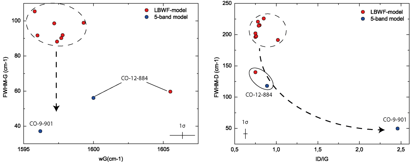
Figure 3.17. Raman parameters determined from the 2-band and 5-band fits. Left: FWHM-G vs. \omega_G . Right: FWHM-D vs. I_D/I_G . Typical error bar ( 1\sigma ) is given for each plot. CO-9-901 and CO-12-884 spectra plot outside the sample domain, probably because they have experienced higher temperatures. The arrows illustrate the growth of graphitic domains, with an increase of the I_D/I_G ratio and a decrease of the FWHM of the G and the D bands (Ferrari and Robertson, 2000, Busemann et al., 2007).
