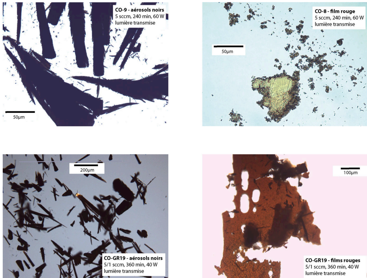
Figure 3.8: Microscopy images of dark and red-brown grains from the Nebulotron discharge. Scale bars are shown on the pictures.
