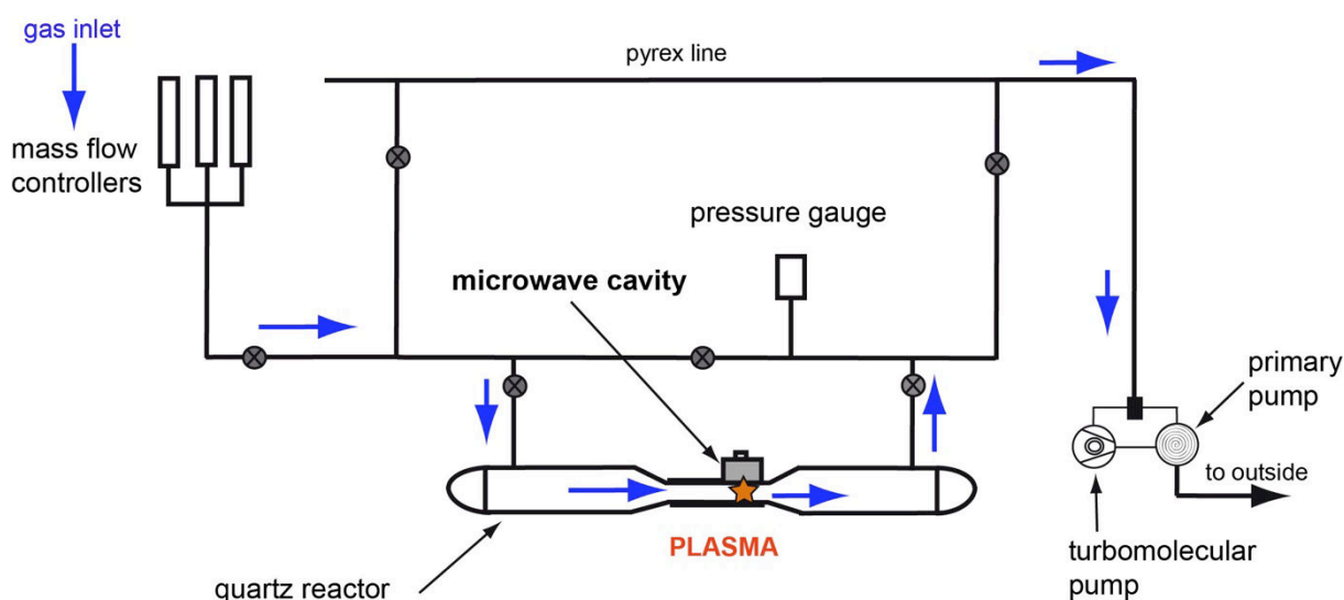
Figure 2.10. Schematics of the Nebulotron glass line.
