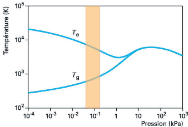
Figure 2.2. Electron temperature T_e and neutral temperature T_g as a function of pressure in an Ar plasma. The orange area represents the pressure conditions used during this thesis and give approximated T_e and T_g values of 10^4 and 800 \text{ K} , respectively.
