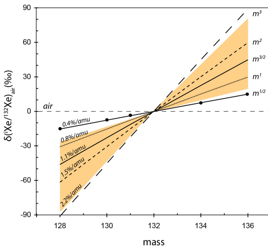
Figure 5.12. Xe isotopic fractionations for all the Nebulotron samples (orange area) assuming a mass-dependent fractionation laws with isotopic fractionation depending on m^{1/2} , m^1 , m^{3/2} , m^2 and m^3 . Isotopic fractionation factors in \%/amu are given for each law.
