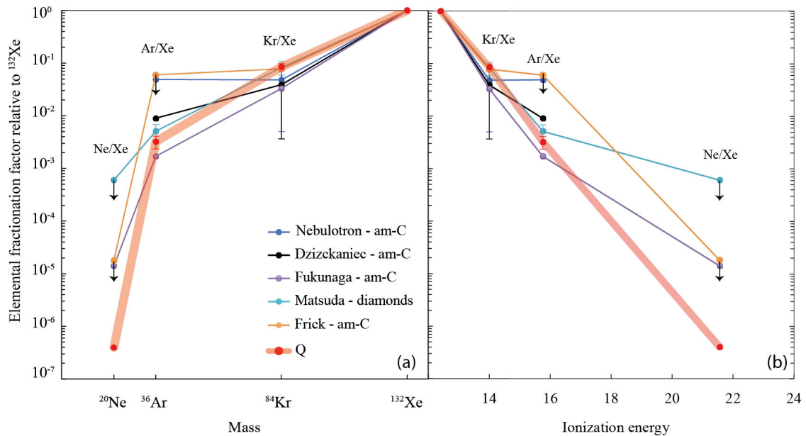
Figure 5.19. Elemental ratios of Q (average from Busemann et al., 2000) and of trapped noble gases in synthetic carbon compounds from plasma experiments (this study and Dzizckanec et al., 1981, Frick et al., 1979, Fukunaga and Matsuda, 1997, Marrocchi et al., 2011, Matsuda et al., 1991). Ratios are normalized to ^{132}\text{Xe} and to the solar abundance for Q and to the elemental composition of the starting gases for the experiments. (a) plotted vs. mass and (b) plotted vs. ionization energy. Arrows show the upper limits for some experimental ratios.
