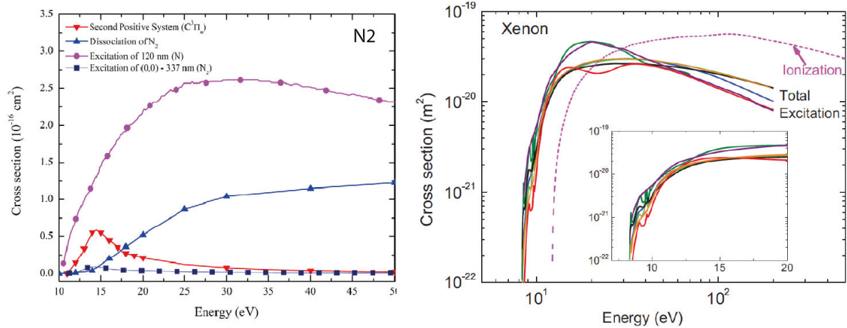
Figure 2.5: Electron-impact excitation and ionization cross section for N_2 and xenon as a function of electron energy. Left : electron-impact cross section for the excitation of different N_2 excited states and the dissociation of N_2 (from Fierro et al., 2012). Right : total excitation and ionization cross section of xenon (from Bordage et al., 2013).
