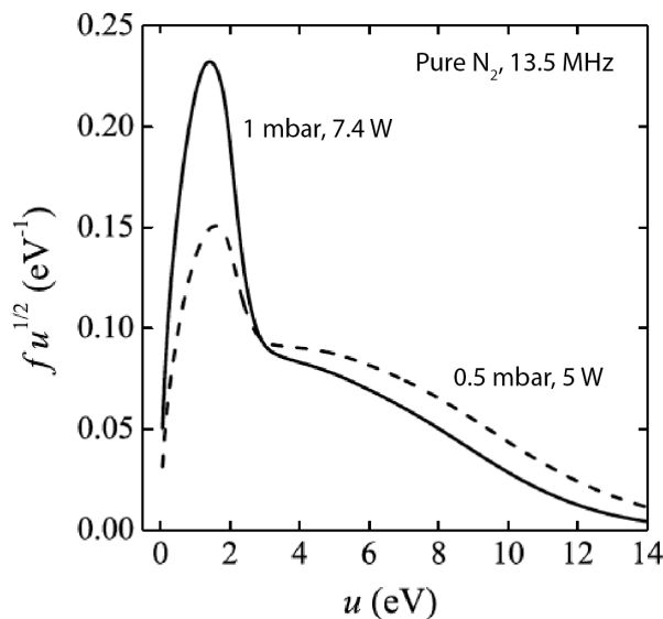
Figure 2.6. Example of EEDF in a N _2 plasma (PAMPRE, from Alves et al., 2012).
