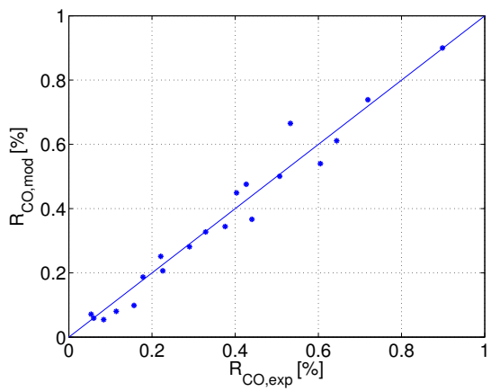
(c) CO
