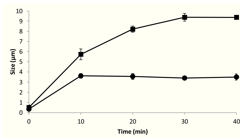
Figure 1: Size evolution measurements in the Moselle water of 100 mg/L of TiO 2 -NP (black square) and 10 mg/L of TiO 2 -NP (black circle).
