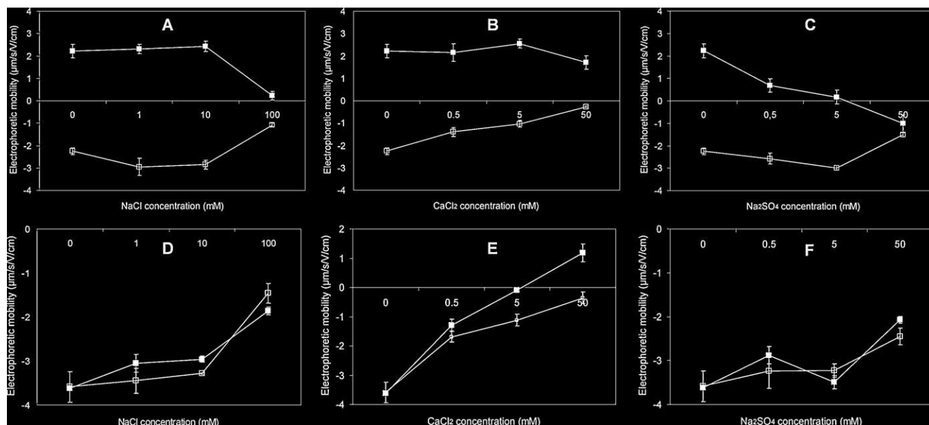
Fig. 5. The electrophoretic mobility of both NP-TiO 2 (black squares) and Escherichia coli cells (open squares) as a function of (A) NaCl, (B) CaCl 2 , (C) Na 2 SO 4 at pH 5.5 and (D) NaCl, (E) CaCl 2 , (F) Na 2 SO 4 at pH 9.5.
