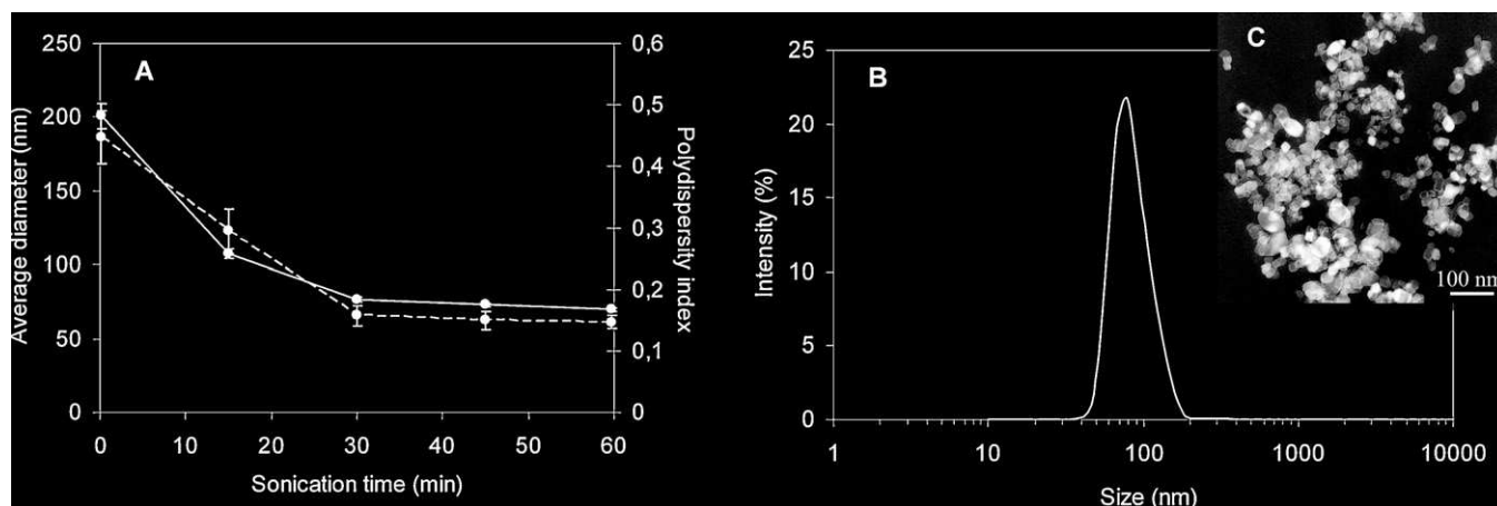
Fig. 1. Physical characterization of the NP-TiO 2 stock suspension. (A) Hydrodynamic diameter and polydispersity index of the NP-TiO 2 after various sonication times in mQ water. (B) Particle size distribution (B) and transmission electron microscopy image (C) of the NP-TiO 2 after 30 min of sonication in mQ water.
