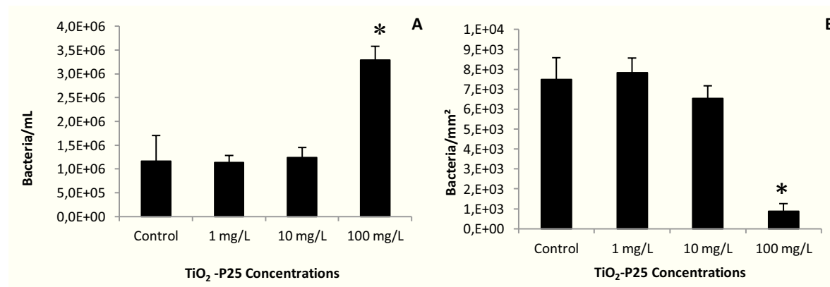
Figure 2: Evaluation of planktonic (A) and sessile (B) bacterial biomass with DAPI staining after 2 weeks of exposure to TiO 2 -NP. Significant statistical differences between samples are indicated with a level of significance of p < 0.05 with Kruskal-Wallis test.
