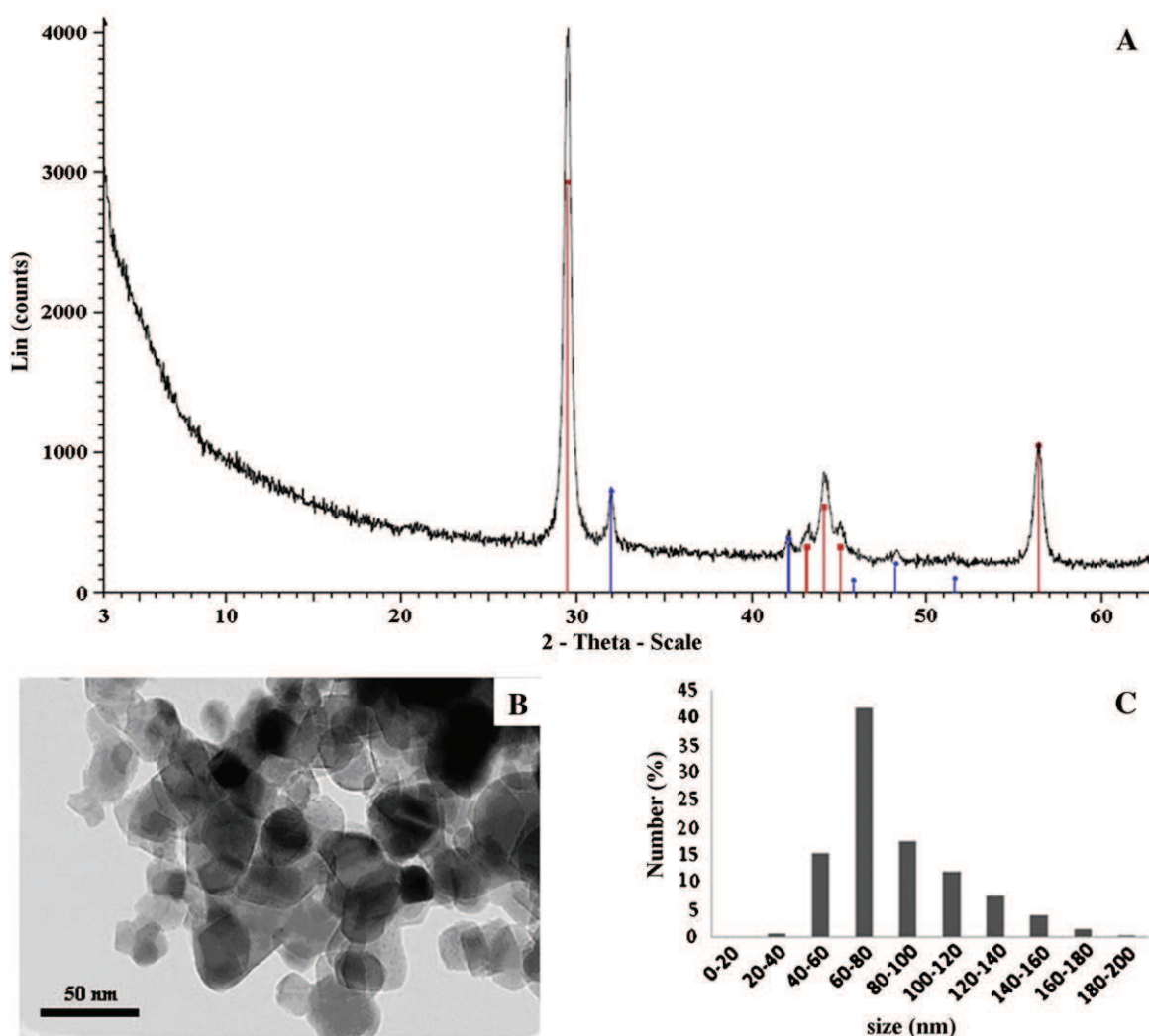
Fig. 1. Characterization of the TiO 2 -P25 nanoparticles. (A) X-ray diffraction pattern of the initial TiO 2 -P25 nanoparticles. Red peaks were assigned to the anatase form and blue peaks to the rutile form; (B) TEM micrograph and (C) hydrodynamic diameter of the TiO 2 -P25 nanoparticle stock suspension after 30 min of dispersion by sonication in ultrapure water.
