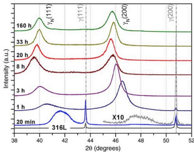
Fig. I. 28: XRD patterns for different nitriding durations. The peaks 316L ( \gamma ) and expanded austenite ( \gamma_N ) are indicated for the 111 and the 200 reflections (The low intensity 200 \gamma_N peak for 20 min of nitriding has been multiplied by 10) (Stinville et al., 2010).
