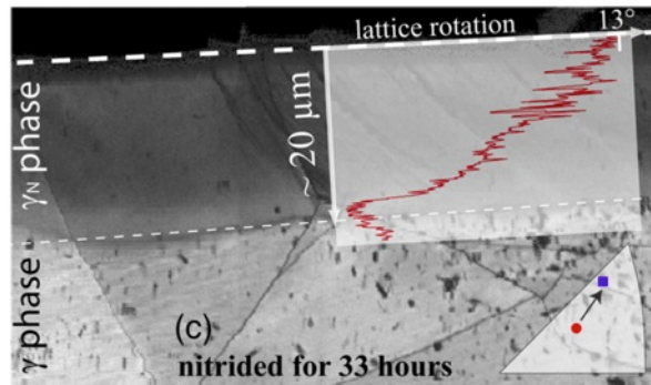
Fig. I. 36: The gradient of the misorientation across then nitrided zone of an AISI 316L after 33 h of nitriding, where the bold white dashed line indicates the surface (the red circle and the blue square in the insert ND inverse pole figure indicate the orientation of the non-nitrided and nitrided region of the grain, respectively)(Templier et al., 2010).
