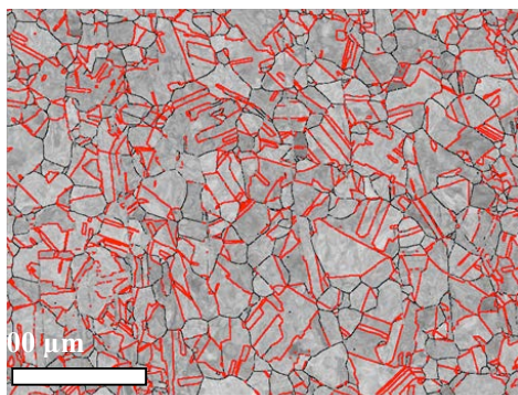
Fig. II. 1: SEM image of the AISI 316L initial microstructure and the distribution of the Sigma-3 boundaries (thermal twins).
