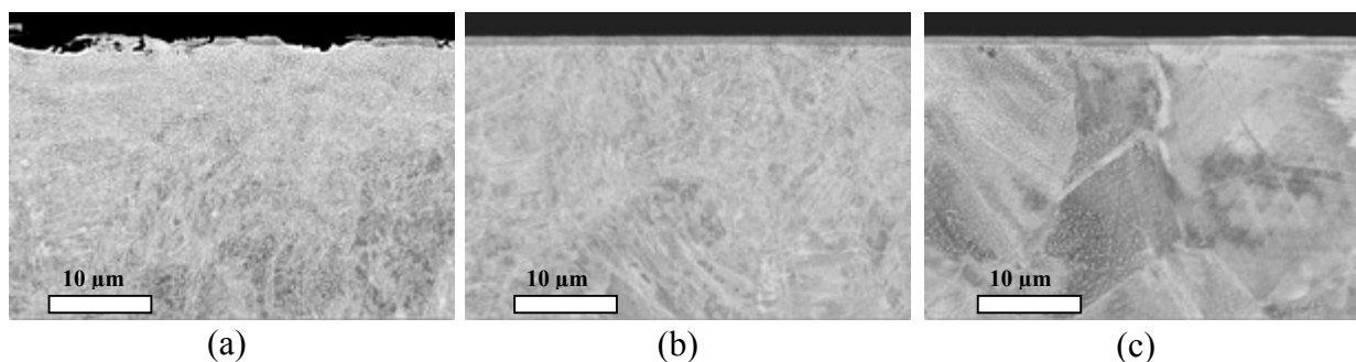
Fig. IV. 12: SEM cross section images showing the nitrided layer in the case of (a) the raw SMAT-ed surface nitrided, (b) SMAT-ed + electropolishing for 20s + nitrided and (c) SMAT-ed + electropolishing for 60s + nitrided. The sample was treated with 100Cr6 balls for 17 min.
