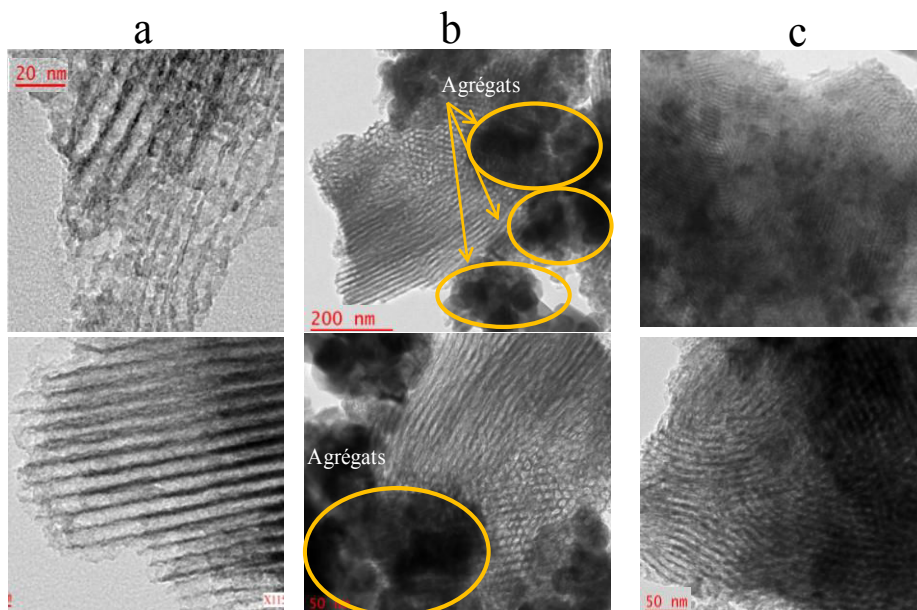
Figure IV-30 – Clichés MET de \text{TiO}_2 four (a), \text{Zn}(\text{OAc})_2[\text{Ti} - \text{Zn}] four (b) et \text{Zn}(\text{OAc})_2[\text{Ti} - \text{Zn}] IF (c).
