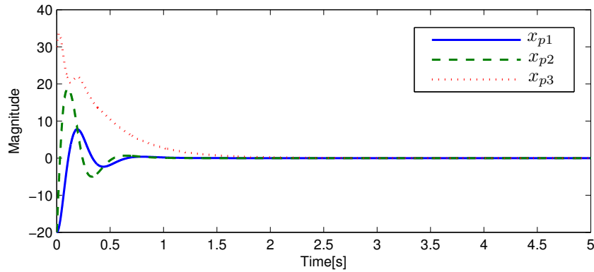
FIGURE 2.2: States of the plant
