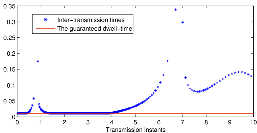
FIGURE 3.2: Inter-transmission times.
