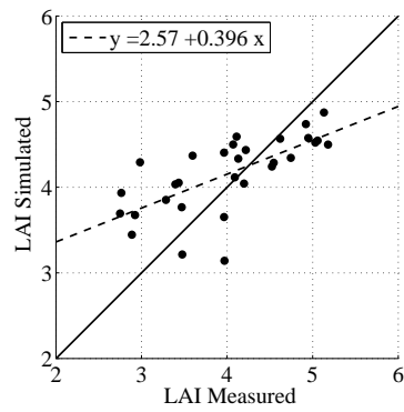
Figure 6: Comparison of the measured and simulated data in the E137 plantation (site 1): first-order linear regression for litterfall ( LF ) (above) and leaf area index ( LAI ) (below).
