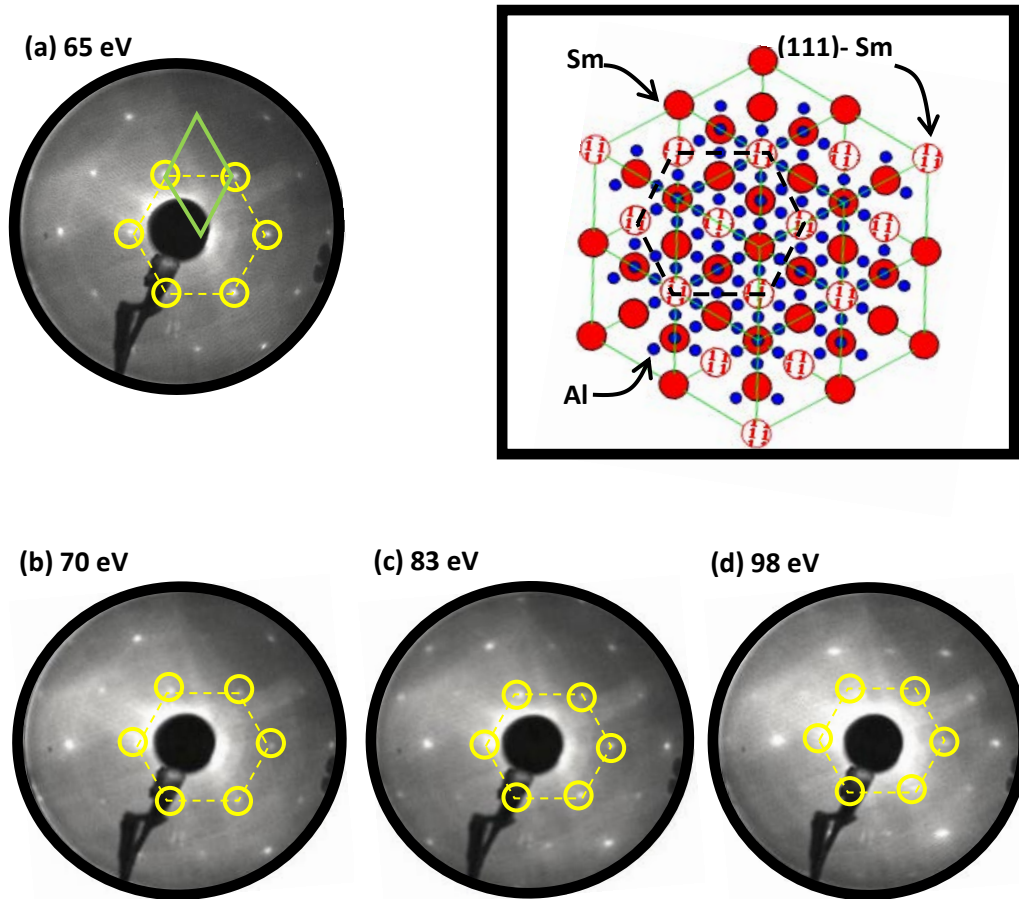
Figure 5: LEED patterns collected at 65 eV (a), 70 eV (b), 83 eV (c) and 98 eV (d) on (111)SGA surface. The elementary mesh of SGA is sketched by the green diamond. Upper right: (111) \text{SmAl}_2 plane, as obtained from the software CaRIne.
