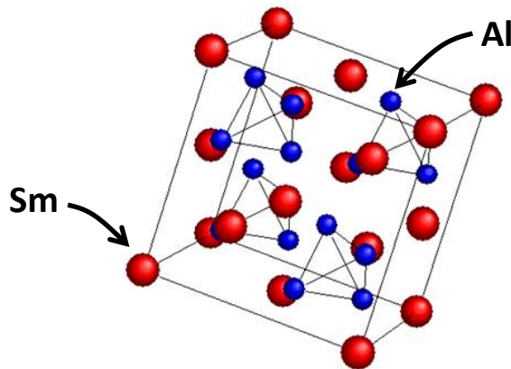
Figure 2: Sketch of the cubic Laves phase structure in the case of \text{SmAl}_2 .
