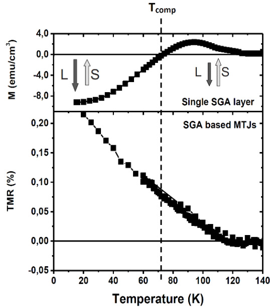
Figure 14: Top: Magnetization of a SGA single layer versus temperature, in increasing temperature under zero-applied field after field-cooling under +7 T. The magnetic L and S configurations in the SGA epitaxial layer are sketched with the dark and light grey arrows respectively. Bottom: TMR of a SGA/ \text{AlO}_x /[Co/Pt] 5 MTJ versus temperature.
