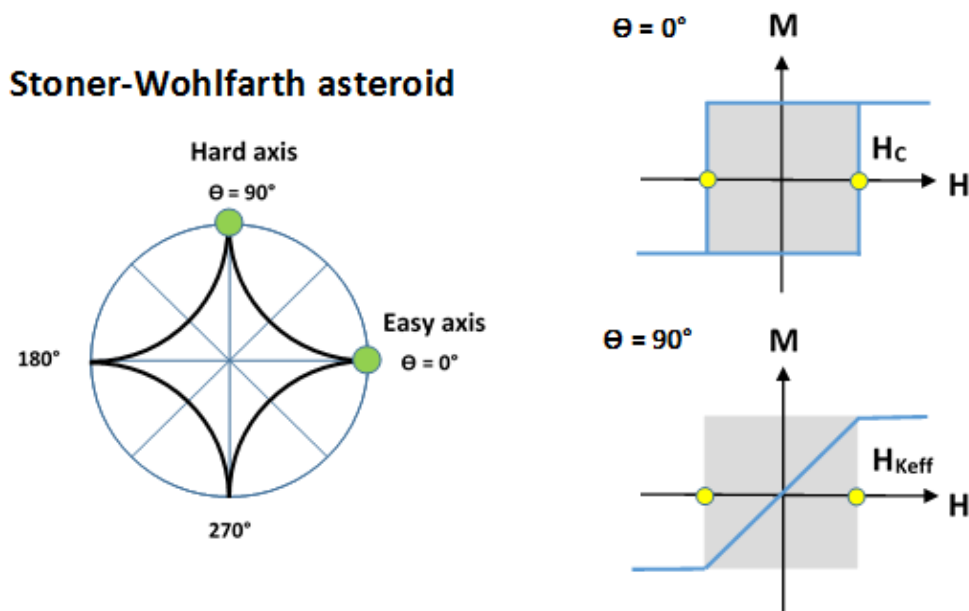
Figure 3: Left: Stoner-Wohlfarth asteroïd. Right: M(H) loops for particular \Theta angles of the Stoner-Wohlfarth asteroïd.
