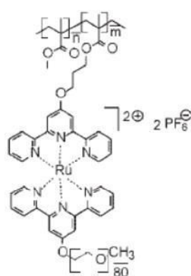
Figure 9. Structure of the graft copolymer used by Schubert et. al. [36]
