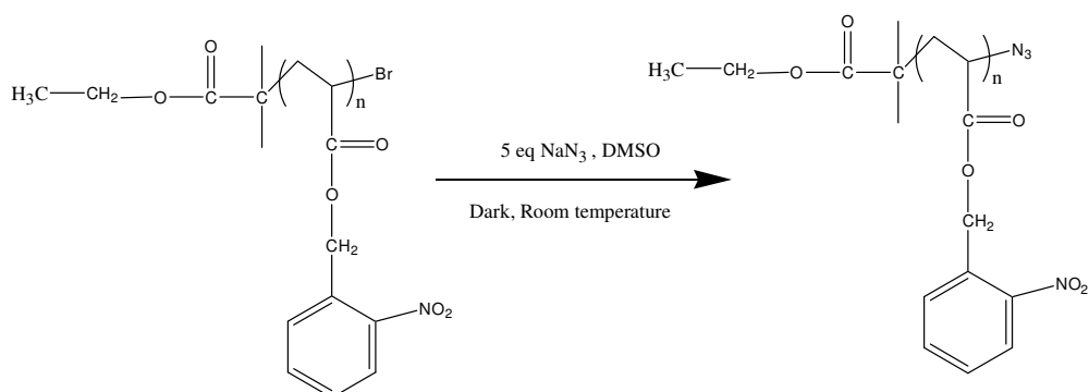
Scheme 1. Modification of PNBA-Br by using NaN 3
