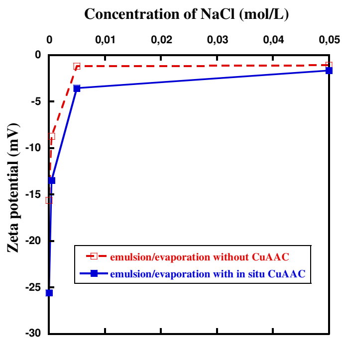
Figure 75. Evolution of zeta potential of nanoparticles preped via emulsion/evaporation method versus NaCl concentration.
