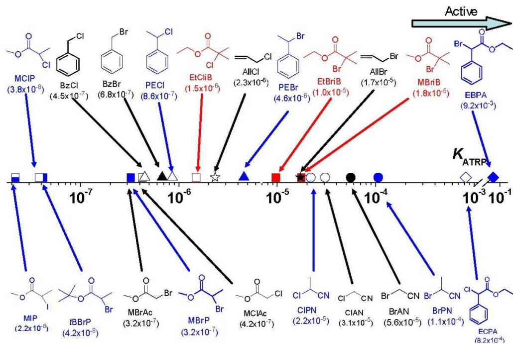
Figure 47. ATRP equilibrium constants for various initiators with Cu^I X/TPMA ( X= Br or Cl ) in MeCN at 22 °C [144].
