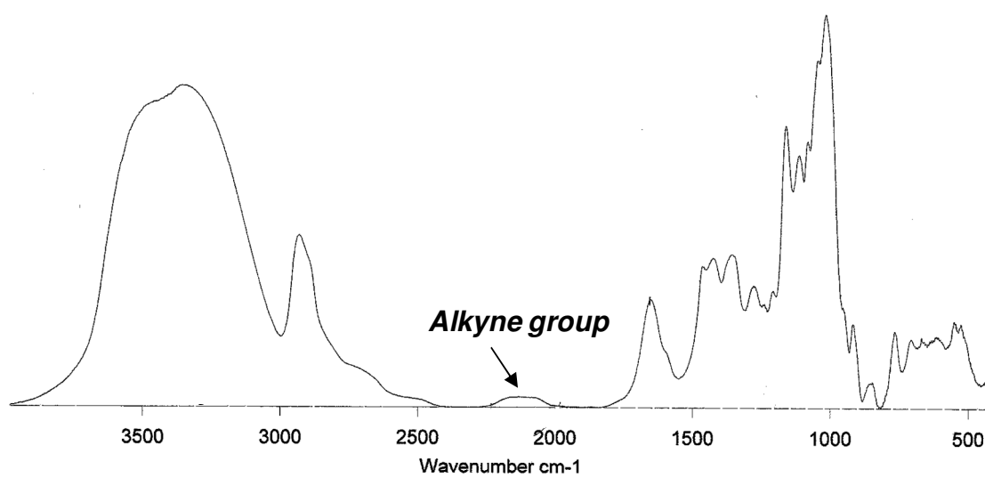
Figure 112. FT-IR chart of \text{-alkyne} dextran
