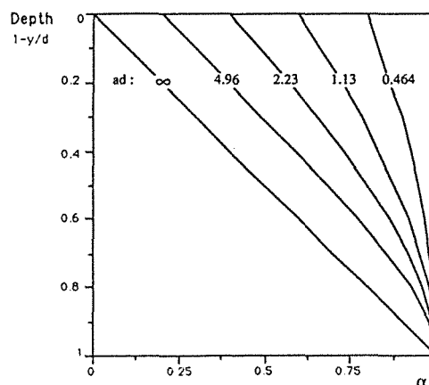
FIG. 2. Dependence of the dimensionless temperature \alpha on the dimensionless depth d for several values of the parameter a \cdot d .
