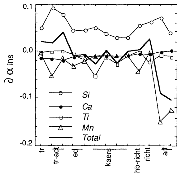
Figure 8 : Contribution of Si, Ca, Ti and Mn beam intensities to the variation of the D/H instrumental fractionation factor \alpha_{\text{ins}} , as calculated from Eqn. 1, on each of the standard amphiboles.
