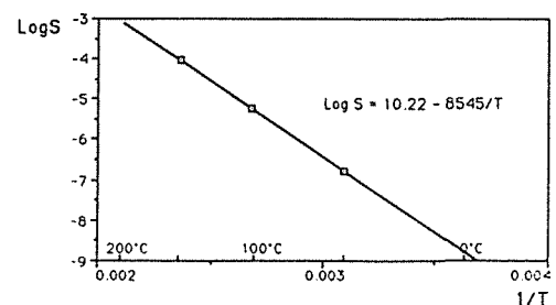
FIG. 4. Solubility of PbS in brines as a function of temperature, T . Brines are 2.8 molal in NaCl, 0.64 molal in CaCl_2 , and 1 pH unit below neutral.
