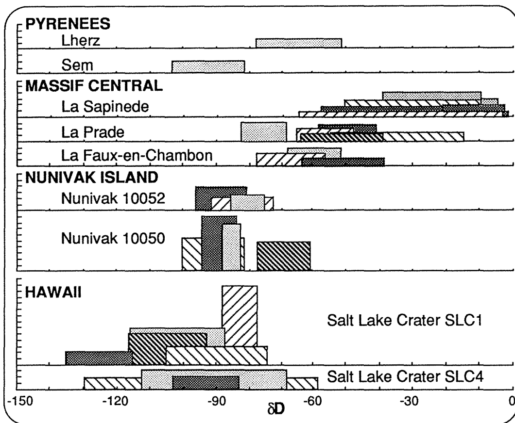
Figure 5 : Distribution of ion probe probe measured \delta D_{\text{smow}} in mantellic kaersutite and pargasite.
