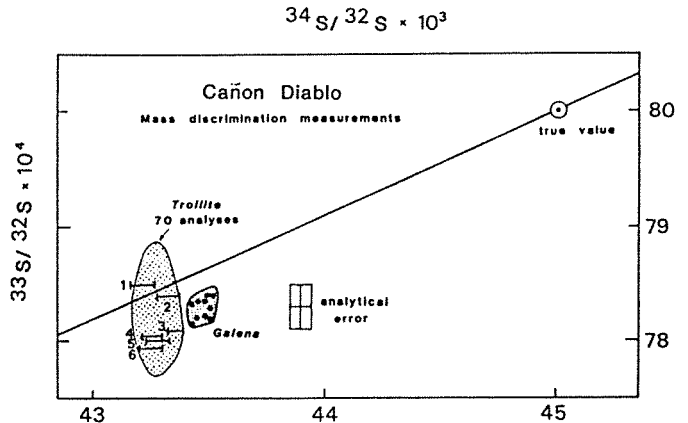
FIG. 2. Reproducibility and calibration of sulfur isotope analyses. The dotted area encloses 70 measurements of Canyon Diablo troilite, measured on six days in a one-month period. The mean value of ^{33}\text{S}/^{32}\text{S} and the total variation of ^{34}\text{S}/^{32}\text{S} are reported for each day. True values for Canyon Diablo are 45 \cdot 10^{-3} and 8 \cdot 10^{-3} . The line is the theoretical fractionation line. We also reported measurements of Manitowadge galena, which has the same isotopic composition as Canyon Diablo troilite. The change in the mass discrimination effect is due to matrix effects.
