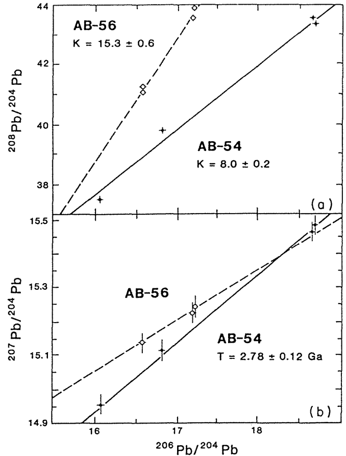
FIG. 4. Pb-isotopic results on pyrites from the Lamaque gold mine.
