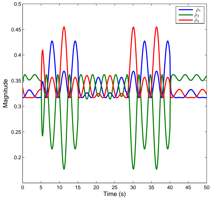
Figure 3.2 – Estimated scheduling functions \rho_i(\hat{x}(t)) .
