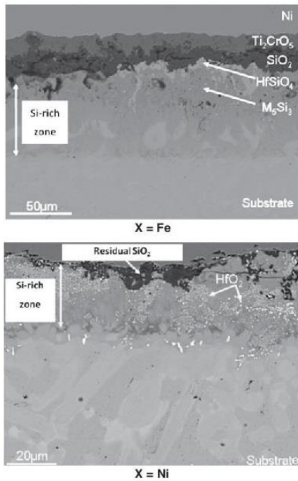
Fig. 5. Cross sections of the MASC samples with Fe- and Ni-containing coatings after 50 h isothermal oxidation at 1300 °C.
