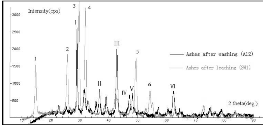
Figure 3. 17: XRD pattern of the ashes ( A_{12} & SW_1 )
