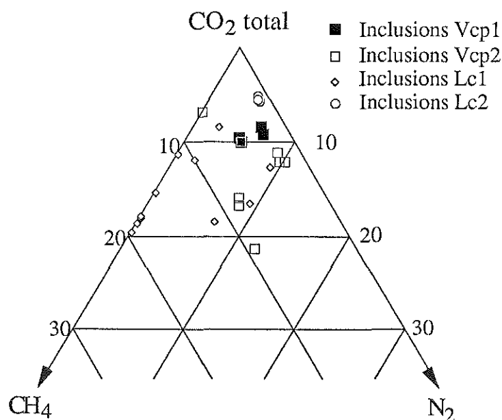
Figure 5.25 : composition de la phase volatile
