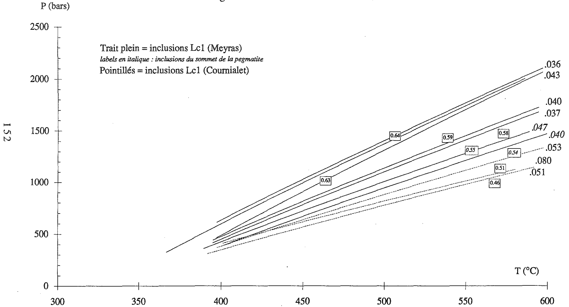
Figure 5.14 : isochres des inclusions Lc1
