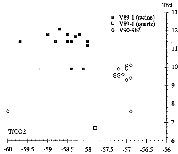
A - Diagramme TfCO2-Tfcl des inclusions Lc1
