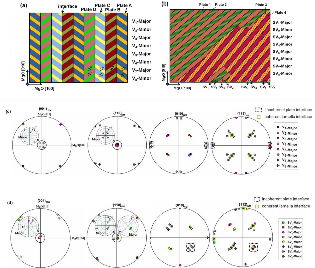
Fig. 5.5. (a-b) Schematic illustration of the geometrical configuration of NM plates. V 1 , V 2 , ..., V 8 and SV 1 , SV 2 , ..., SV 8 denote eight orientation variants in the low relative contrast zones ( Z_1 ) and in the high relative contrast zones ( Z_2 ), respectively. (c-d) Representation of measured orientations of in-plate lamellar variants in the form of \{001\}_{Tetr} , \{110\}_{Tetr} , \{010\}_{Tetr} and \{112\}_{Tetr} pole figures. The orientations of the intra- and inter-plate interface planes are respectively indicated by light green solid squares and black dotted rectangles in the \{010\}_{Tetr} and \{112\}_{Tetr} pole figures.
