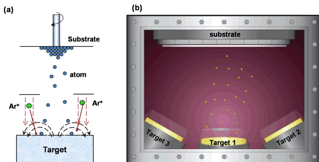
Fig.2.2 illustration of direct current magnetron sputtering process (a) and the confocal magnetron sputtering system (b).
