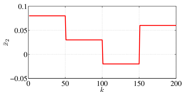
Figure 3.3: Reference \bar{x}_2(k) .
