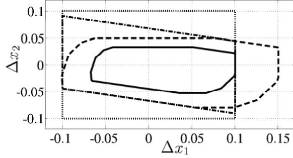
Figure 4.7: Homothetic transformation for 30 \leq k < 90 or k \geq 140 . Dotted line: constraint X_\Delta(k) . Dash-dotted line: constraint \mathcal{X}_\Delta(k) . Dashed line: nominal invariant set \hat{\Omega} . Solid line: \alpha(k)\hat{\Omega} with \alpha(k) = 0.67 .
