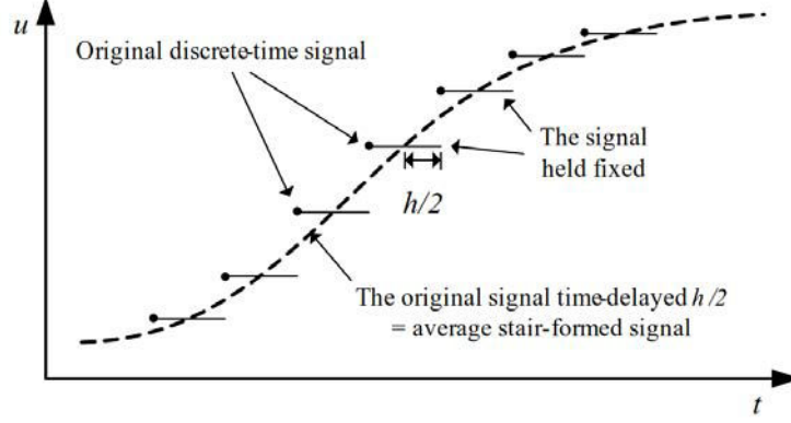
Figure 2.9: Time delay of the discretization process [33]. h = T_s is the time step.
