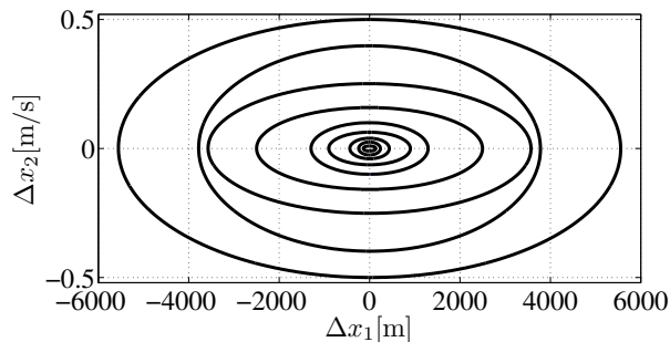
Figure 5.9: Invariant ellipsoids.
