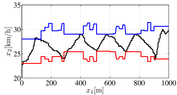
Figure 6.7: Real-time response of the embedded robust adaptive control according to the position. Black line: x_2(t) . Red line: V_{min}(t) . Blue line: V_{max}(t) .
