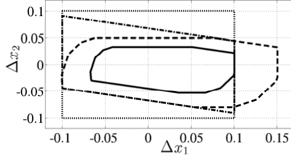
Figure 4.7: Homothetic transformation for 30 \leq k < 90 or k \geq 140 . Dotted line: constraint X_{\Delta}(k) . Dash-dotted line: constraint \mathcal{X}_{\Delta}(k) . Dashed line: nominal invariant set \hat{\Omega} . Solid line: \alpha(k)\hat{\Omega} with \alpha(k) = 0.67 .
