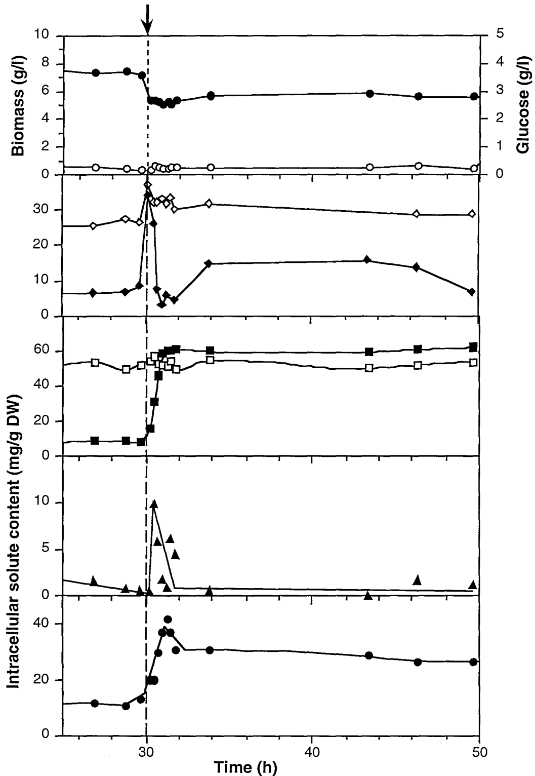
Fig. 1 : Effect of a saline upshock on the intracellular solute content of C. glutamicum on a defined medium. ● Biomass, ○ glucose concentration ; ◇ Potassium, ◆ sodium, ■ proline, □ glutamate, ▲ glutamine, ● trehalose intracellular concentration when the fermentation was started at a medium osmolality of 0.4 \text{ osmol.kg}^{-1} and when NaCl was added (arrow) to rise the osmotic pressure to 1.2 \text{ osmol.kg}^{-1} .
