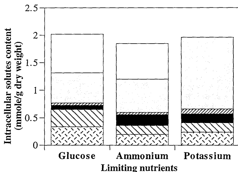
Fig . 6 : Comparison between the steady-state intracellular content of C. glutamicum grown in continuous culture under the different nutrient limitation at an osmolality of 1.2 osmol.kg -1 and a dilution rate of 0.1 h -1 :
