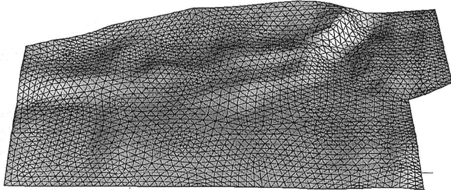
FIGURE 3-21 : maillage quelconque, maillage initial
