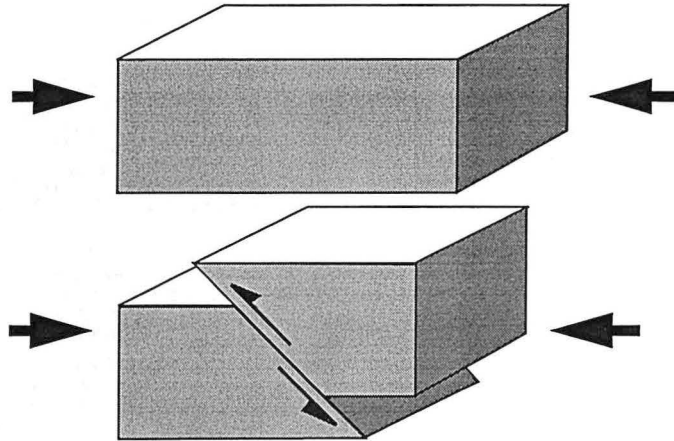
FIGURE 6-3 : Faille inverse
