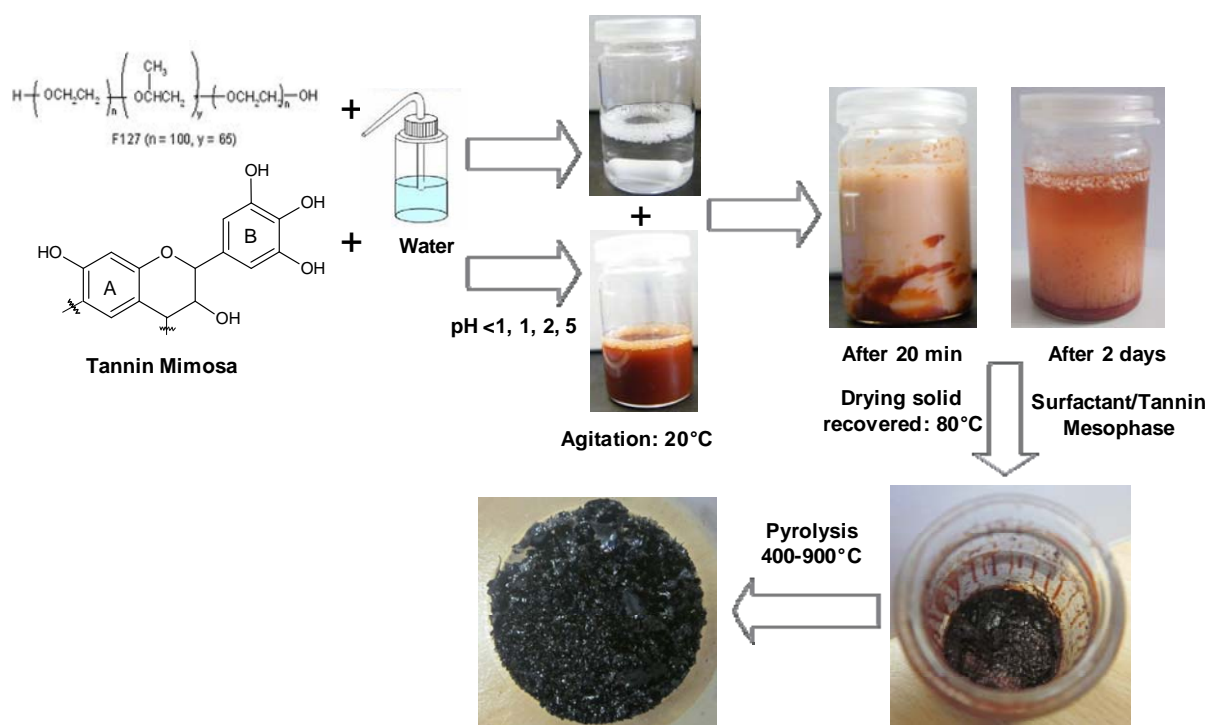
Fig. 91: Schematic approach of OMC's synthesis using tannin and F127.
