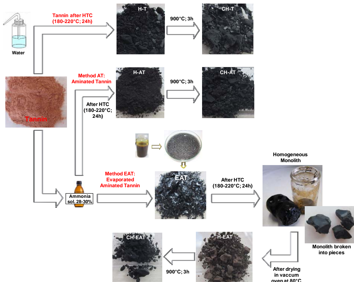
Fig. 60: The methods used for preparing N-doped carbon materials and their respective final products.
