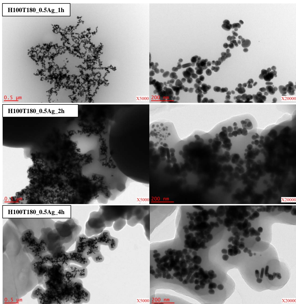
Fig. 55: TEM images of three filtrates obtained after HTC of tannin at 180°C in presence of AgNO_3 solution during 1, 2 and 4h respectively.
