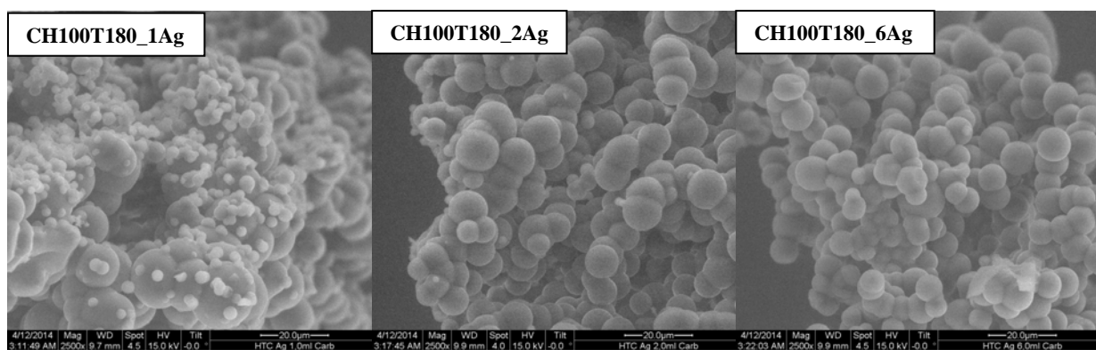
Fig. 56: SEM images of three filtrates obtained after HTC of tannin with 1, 2 or 6 mL of 0.1M AgNO_3 solution at 180°C for 24h and posterior carbonization at 900°C.
