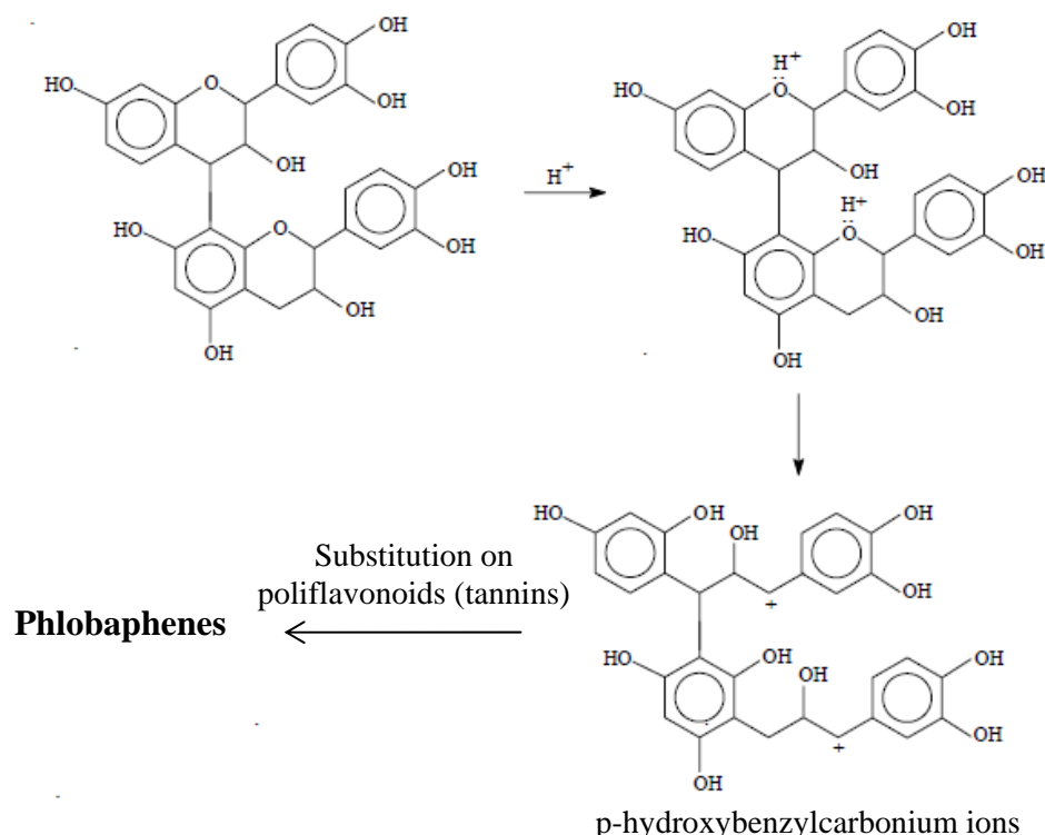
Fig. 19: Tannin autocondensation by acid hydrolysis of heterocyclic rings [Pizzi 1983].
