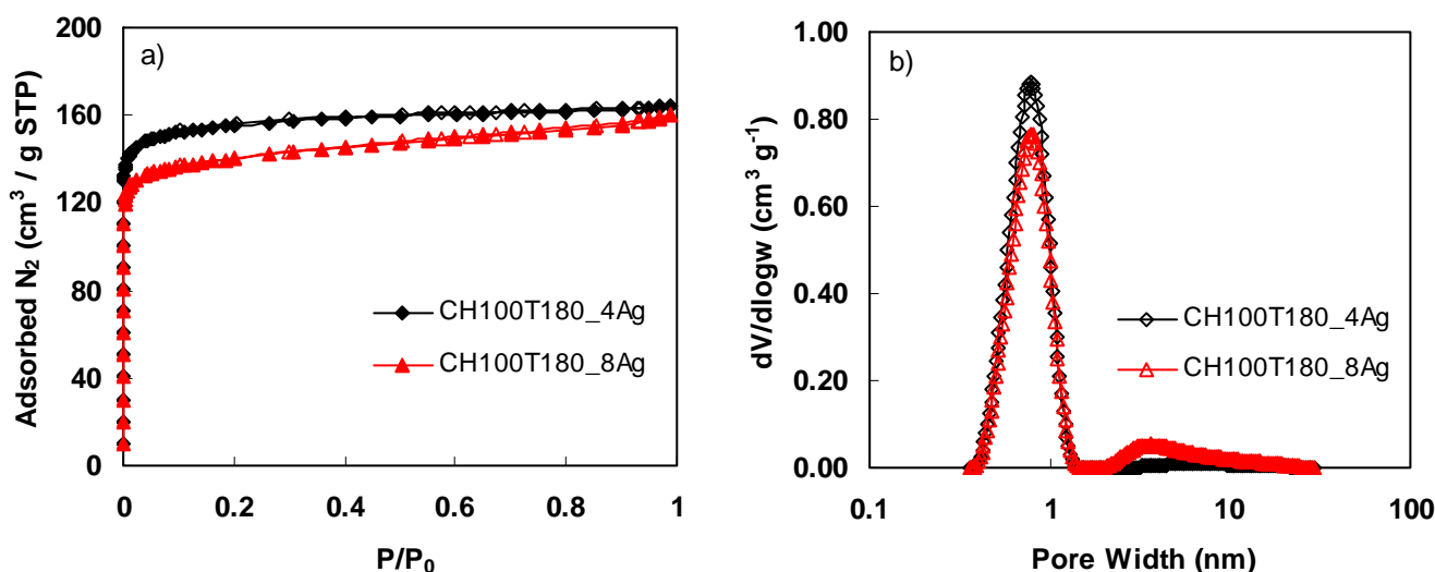
Fig. 58: a) Nitrogen adsorption-desorption isotherms (full and open symbols, respectively) at -196^\circ\text{C} for pristin two materials made after HTC at 180^\circ\text{C} having 4 and 8g of an aqueous solution of AgNO_3 after posterior pyrolysis at 900^\circ\text{C} ; and b) their correspondent pore size distribution obtained by PSD.
