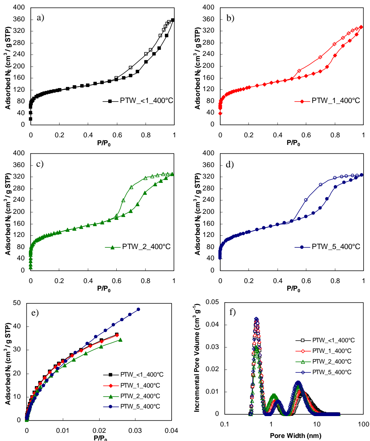
Fig. 93: a) to d) Nitrogen adsorption-desorption isotherms (full and open symbols, respectively) at -196°C for different pHs; e) CO 2 adsorption isotherms at 0°C for PTW carbon materials at different pHs after pyrolysis at 400°C; and f) pore size distribution calculated by DFT model for all samples prepared at different pHs and calcined at 400°C.
