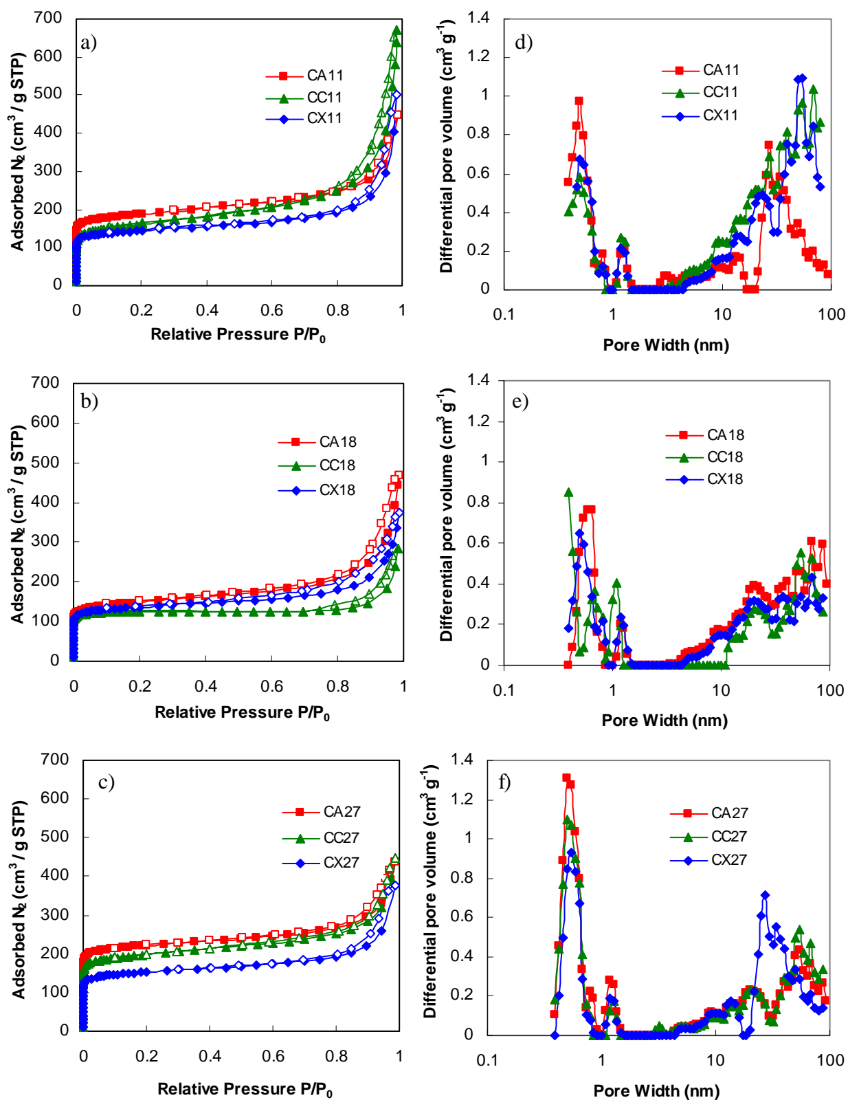
Fig. 83: (a), (b) and (c) Nitrogen adsorption-desorption isotherms at -196\text{ }^{\circ}\text{C} of CA, CC and CX carbon gels at different percentages 11, 18 and 27%, and (d), (e) and (f) their corresponding pore size distributions.
