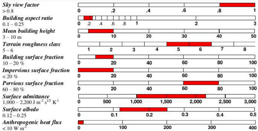
Figure A.9 : Type de LCZ 9 Sparsely built.
