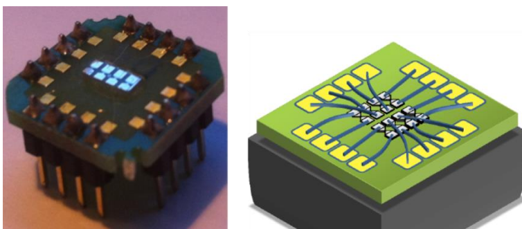
Figure 2 - 12: The pictures of magnetic tunnel junctions mounted on a chip.
