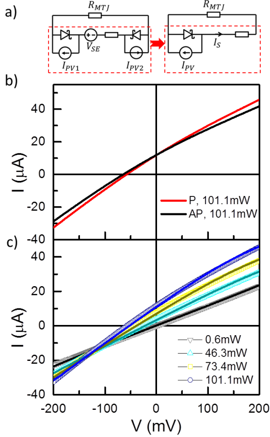
Figure 4 - 18: Measurement and simulation of I(V) curves under different power. a) Sketch of the electric circuit used to model the I(V) curves, in which I_{PV} , V_{SE} stand for the photovoltaic current and Seebeck voltage. The two sources are equivalent to an effective Schottky barrier, of which the photo generated current is given by I_{PV'} . b) I(V) curves for P and AP magnetic configuration obtained on a Contact geometry device. c) I(V) for the P magnetic configuration for different laser power.
