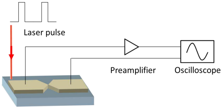
Figure 2 - 15: Sketch of setup for time resolved measurement. Periodical laser pulse shines at the sample and the voltage signal is amplified using a preamplifier before recorded by an oscilloscope.
