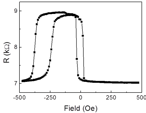
Figure 2 - 13: Typical resistance versus field loop of an \text{Al}_2\text{O}_3 MTJ. The multilayer structure consists: Ta (5nm)/Co (10nm)/IrMn (7.5nm)/Co (5nm)/ \text{Al}_2\text{O}_3 (2nm)/Co (10nm)/Pt (5nm). The reversal of the 10nm thick free Co and 5nm thick Co pinned layer are clearly separated.
