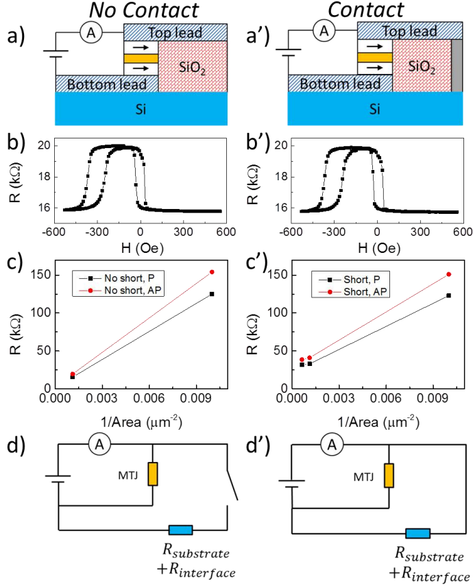
Figure 4 - 1: Resistance study of two magnetic tunnel junctions. The multilayer stack, namely Ta(5nm) /Co(10nm)/ IrMn(7.5nm)/ Co(5nm)/ Al 2 O 3 (2nm)/ Co(10nm)/ Pt(5nm)), is grown on a Si substrate: in a No Contact (left panel) and Contact (right panel) geometry. a) Schematic of the devices in a resistance measurement configuration, b) Resistance of the MTJ as a function of the in-plane applied field c) Resistance of MTJ versus the inverse of the junction area, d) Schematic of the equivalent circuits that corresponds to the two geometries.
