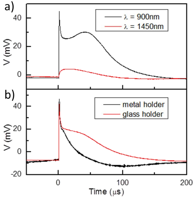
Figure 4 - 7: Time resolved measurement on a simplified sample.
