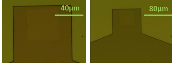
Figure 2 - 8: Optical microscope photo of resist in the shape of bottom electrode. Resist on top of the multilayer stack to define the lateral shape of the bottom electrode.
