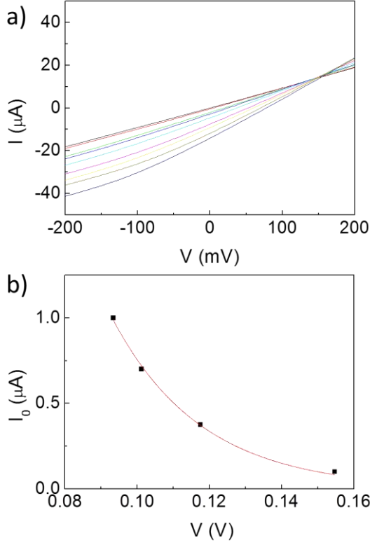
Figure 4 - 19: Simulation of IV curves with different Schottky barrier height. a) Simulated IV curves when the I_0 is set to 100nA. b) Four black dots are the converging points in four IV curve simulation. The red line is fitting using: I_0 \propto \exp(-\Phi_B/kT) .
