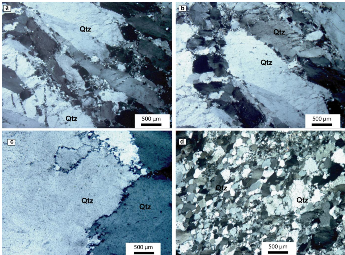
Figure 65: Microphotographies du quartz.
