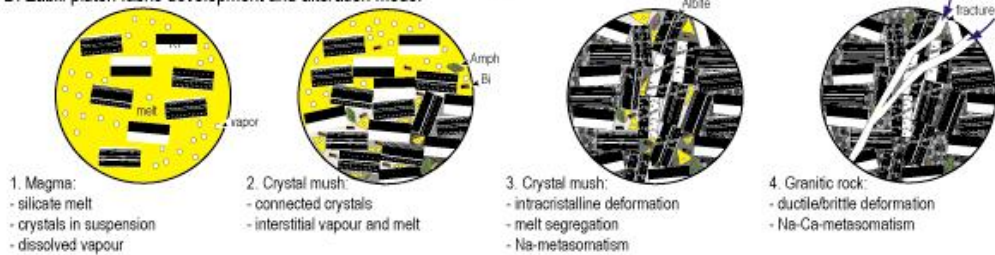
Figure 16. A model for the emplacement of the Zabili pluton and for associated fluids circulation and mineralization. A. Syntectonic emplacement of the Zabili pluton in a dilational jog related to a regional-scale sinistral shear zone. B. Late-magmatic ductile to brittle deformation of the Zabili pluton marked by the development of R' mylonitic to cataclastic shear zones. C. A model for fluid circulations around the crystallizing and cooling Zabili pluton. The circulation of surface-derived fluids is limited to the brittle upper crust whereas the ductile crust is marked by the circulation of magmatic and metamorphic fluids. During
