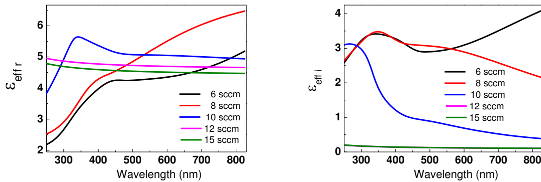
FIG. 4.19. (Left) Real and (right) imaginary parts of the effective dielectric function of as-deposited ZnO-Au nanocomposite thin films grown in the OFR interval from 6 to 15 sccm. The Au content is higher than 15 % in all the films.
