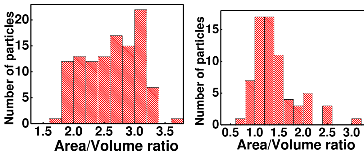
FIG. 4.11. Ratio of surface area to volume of Au NPs in nanocomposite films grown at 8 sccm. (left) As-deposited and (right) annealed at 300 °c, 1h in air.
