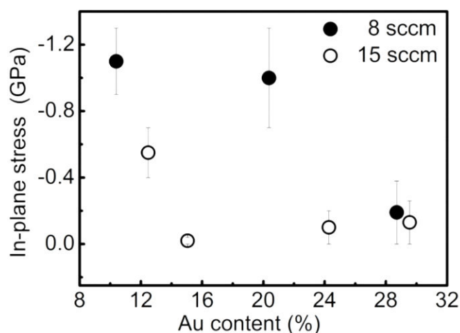
FIG. 4.9. Stress measurements using the curvature method for ZnO-Au nanocomposite films as a function of the Au content and grown with OFrs of 8 sccm (filled circles) and 15 sccm (empty circles).
