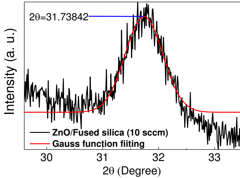
FIG. A.1. In-plane X-ray diffractogram of a ZnO film grown at an OF R of 10 sccm on fused silica. The peak corresponds to the diffraction by {1000} planes of wurtzite ZnO. The red line corresponds to a Gauss function in order to determine with precision the peak position.
