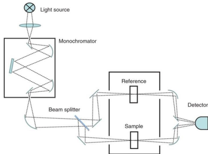
FIG. 2.16. Schematic of a double-beam absorption spectrometer 125 .
