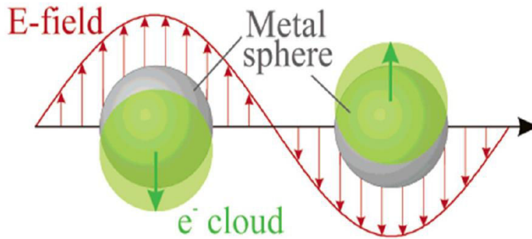
FIG. 1.10. Schematic depiction of the coherent motion of the free electrons in a spherical metallic nanoparticle when excited by an external time dependent electric field fitting the plasmon frequency.
