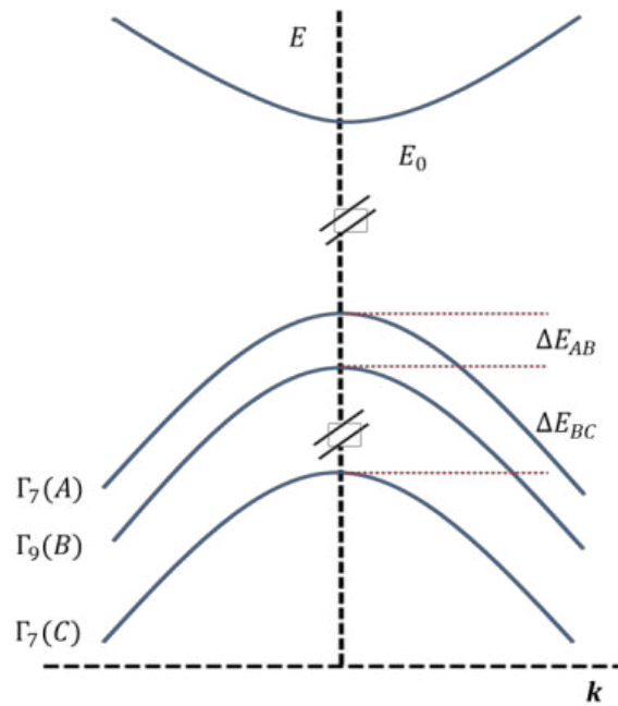
FIG. 1.4. Representation of the conduction and valence band states for ZnO with a direct transition. The valence band is split by into three subbands due to crystal field and spin-orbit interactions. Each subband has a specific symmetry.
