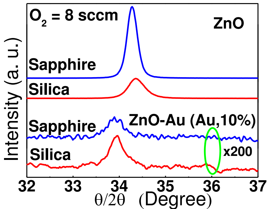
FIG. 4.2. X-ray diffractograms of ZnO and of ZnO-Au (10 % Au) films grown on sapphire (blue lines) and on fused silica (red lines). The ZnO-Au diffracted intensity is magnified by 200 times. All the films were grown with an OF R of 8 sccm. Diffractograms are offset on the y-axis for clarity.
