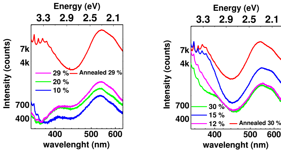
FIG. 4.25. Photoluminescence spectra of as-deposited and annealed ZnO-Au nanocomposite thin films grown with an OFR of 8 sccm with different Au contents (left) and an OFR of 15 sccm with different Au contents (right). For both graphs: red line is for the highest Au content ZnO-Au nanocomposite film after an annealing process for 1h in air at 300 °C.
