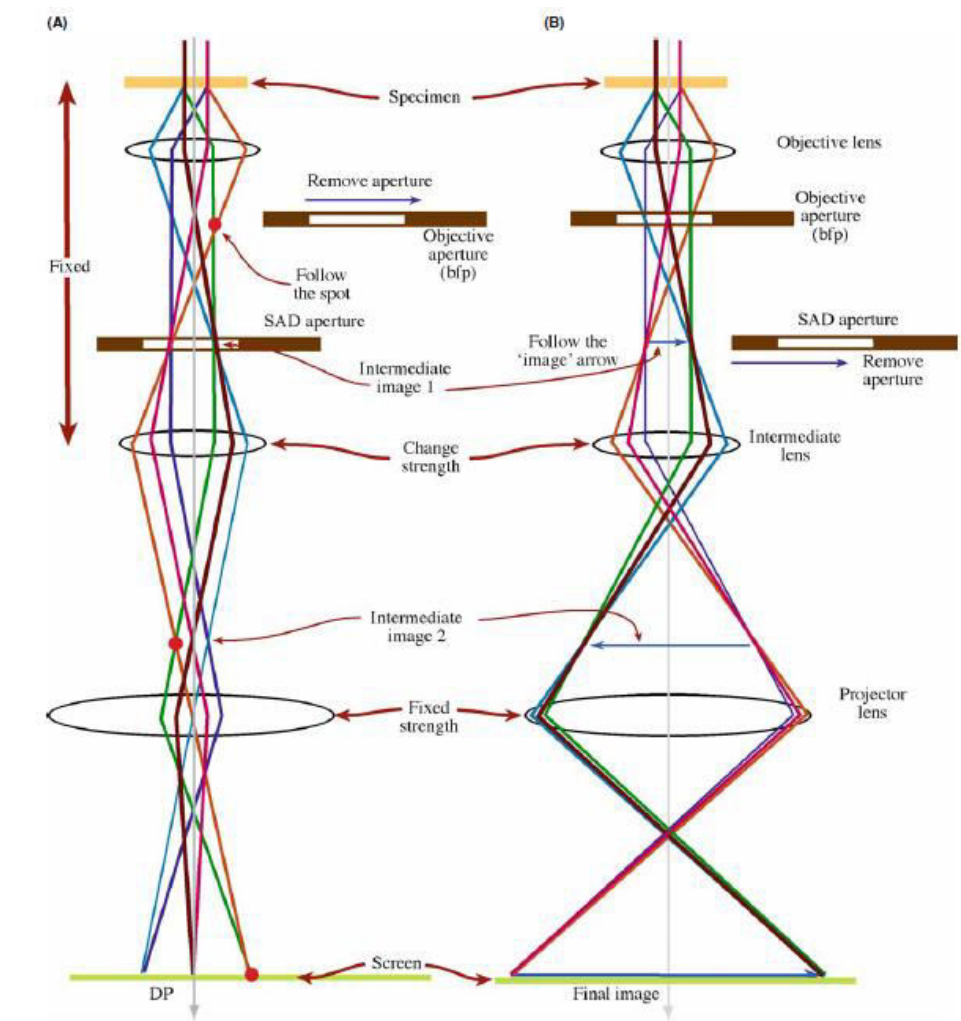
FIG. 2. 12. Diagram of Three lens TEM operating in (A) a diffraction mode and (B) an imaging mode. The figure shows the position of the objective and the SAED apertures 123 .
