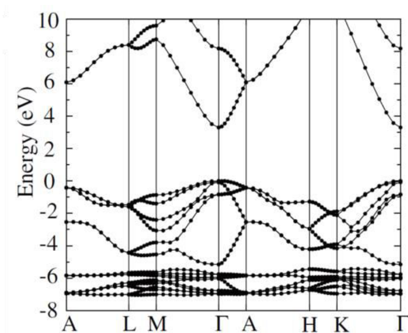
FIG. 1.3 Calculated band structure of ZnO using the HSE hybrid functional in density functional theory. The energy of the valence-band maximum (VBM) was set to zero. From 16 .
