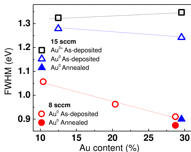
FIG. 4.15. Evolution of the XPS FWHM signal of the Au 0 and Au 3+ peaks of films grown at an OF R s of 8 sccm and 15 sccm as a function of the gold content and influence of the annealing treatment at 300°C. The dotted lines are shown as a visual guide.
