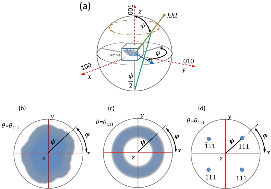
FIG. 2.11. Representation of a (a) pole figure geometry and the 2D stereographic representations of a 4-fold crystal structure material with (b) random orientation, (c) fiber texture and (d) epitaxial alignment.
