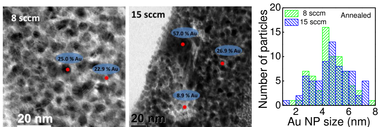
FIG. 4.6. TEM images of 300°C annealed (1h) ZnO-Au nanocomposite thin films with Au contents close to 30% grown with OF Rs of 8 sccm (left) and 15 sccm (center) Corresponding size distribution of the Au NPs (right).
