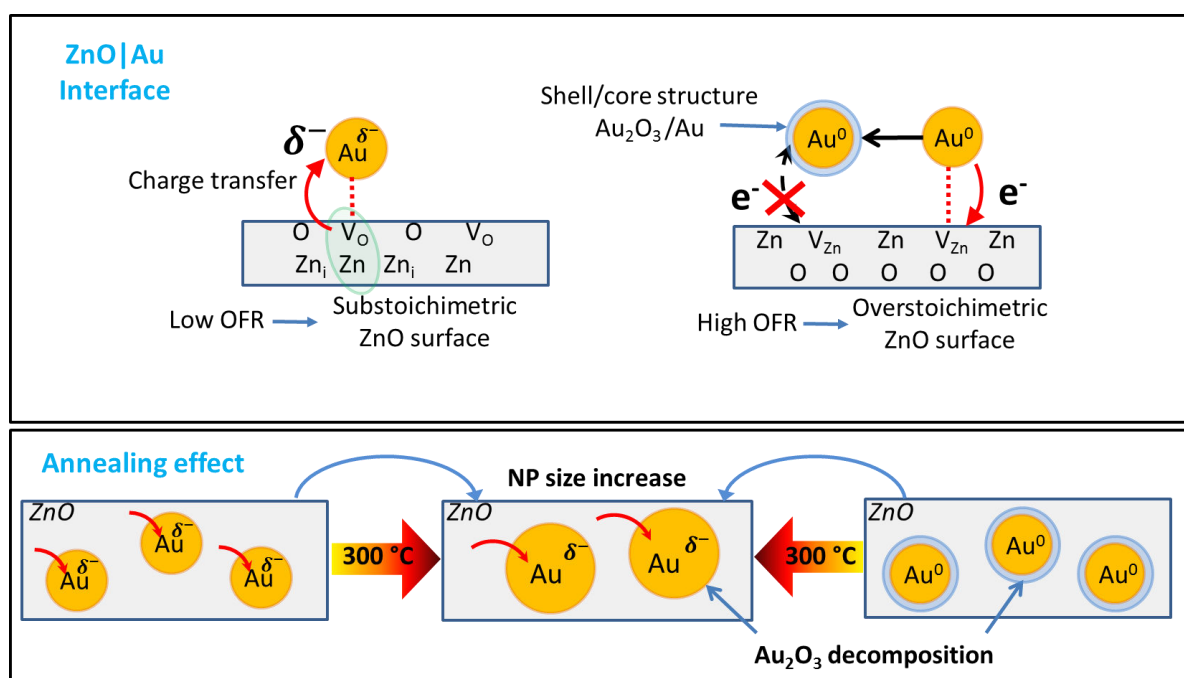
FIG. 4.14. Top. ZnO|Au interface showing the Au NPs-ZnO matrix interaction for nanocomposites grown with an OFR of 10 sccm and below (left) and films grown at OFRs of 12 and 15 sccm (right). Bottom: Interaction of the Au NPs with the ZnO matrix after annealing at 300 °C, 1h in air.
