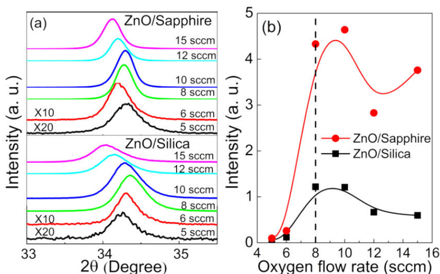
FIG. 3.3. Region of interest of the X-ray diffractograms of ZnO films deposited on fused silica and c -oriented sapphire for different OFRs (a). Evolution of the diffracted intensity with the OFR for films deposited on fused silica and (0001)-sapphire (b). The vertical dashed line indicates the critical oxygen flow rate ( c-OFR ).
