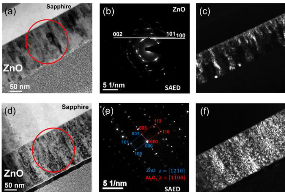
FIG. 3.7. Bright field, dark field images and selected area electron diffraction pattern of ZnO films deposited on (0001)-oriented sapphire at oxygen flow rates of 5 sccm (a-c) and 15 sccm (d-f).
