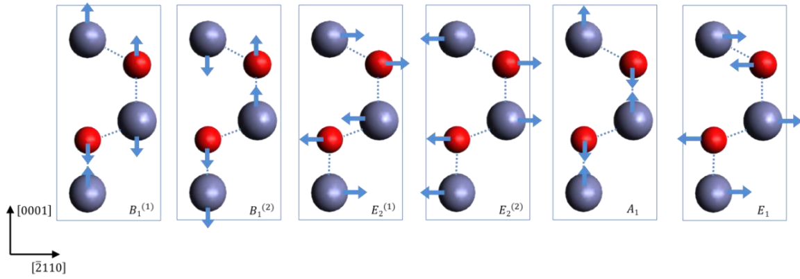
FIG. 1.2. Wurtzite ZnO optical phonon modes. Atoms displacement are indicated by the blue line. Blue and red balls represent Zn and O atoms, respectively.
