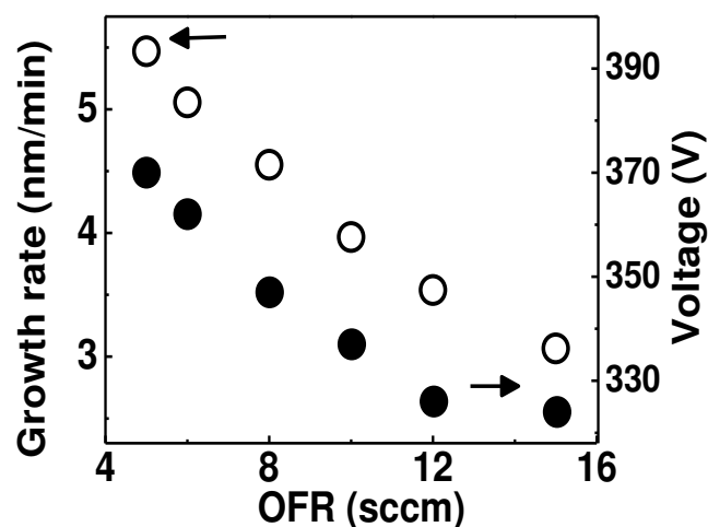
FIG. 3.1 Growth rate (white dots) and discharge voltage (black dots) as a function of the OFR .
