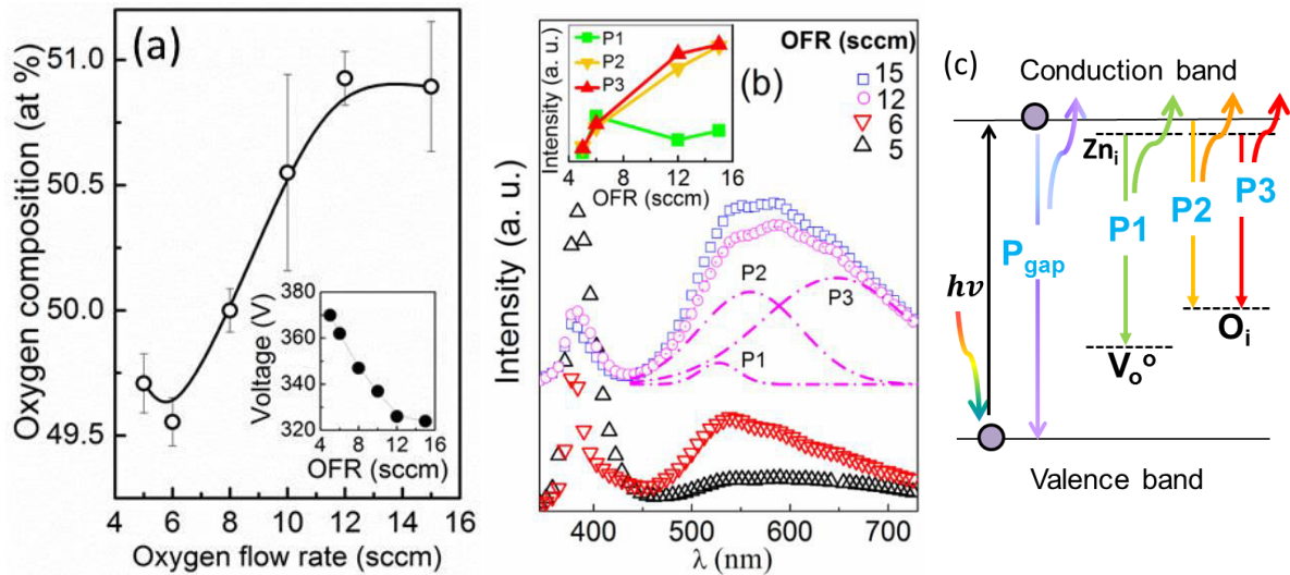
FIG. 3.8. Evolution of the oxygen content and discharge voltage V_d (insert) with the oxygen flow rate for all synthesized films (a). The vertical dashed line indicates the critical oxygen flow rate ( c -OFR). Photoluminescence spectra of ZnO films deposited at different oxygen flow rates (b). An example for the deconvolution of the visible signal in three contributions is shown for the oxygen flow rate of 12 sccm. The insert shows the evolution of the maximal intensity of each contribution with the oxygen flow rate. (c) Schematic diagram showing the interband and intraband transitions in the ZnO films.
