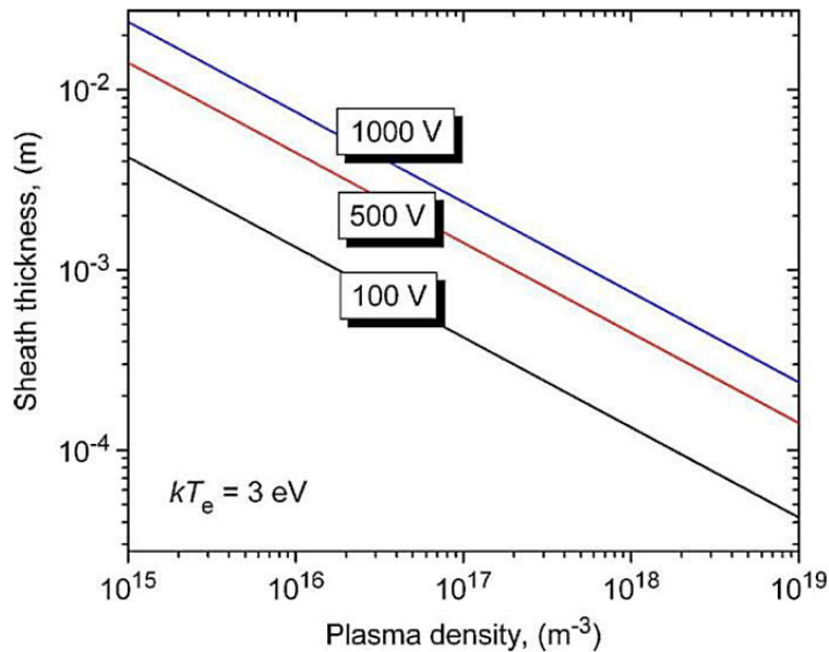
FIG. 2. 3. Child sheath thickness as a function of plasma density, with electron temperature and sheath voltage as parameters 98 .
