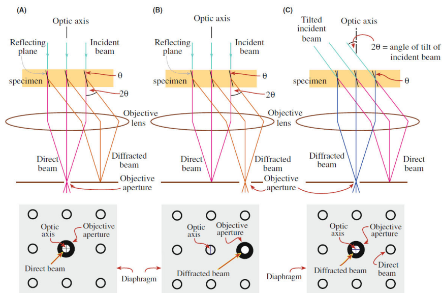
FIG. 2.13. TEM imaging operation modes of (a) bright field and dark field by (b) displacement of the objective aperture and (c) tilting of the incident beam 123 .
