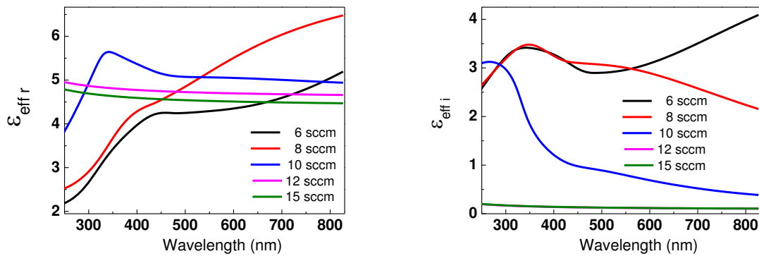
FIG. 4.19. (Left) Real and (right) imaginary parts of the effective dielectric function of as-deposited ZnO-Au nanocomposite thin films grown in the OF R interval from 6 to 15 sccm. The Au content is higher than 15 % in all the films.
