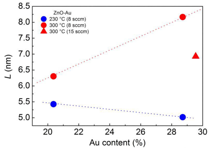
FIG. 4. 10. Length of coherence domains of crystalline gold estimated from X-ray diffractograms of annealed ZnO-Au films for two gold contents and two OFR_s .
