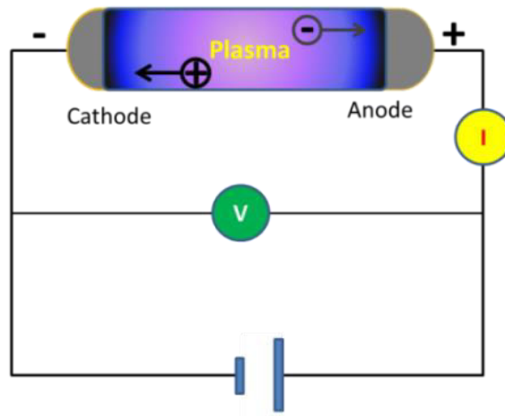
Fig. 2.1. Schematic of a vacuum tube and formation of a glow discharge.
