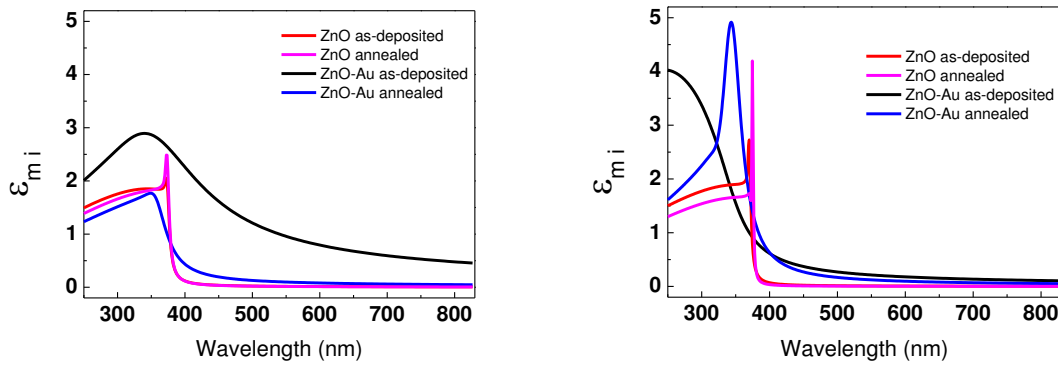
FIG. 4.20. Imaginary part of the ZnO dielectric function in as-deposited and annealed ZnO and ZnO-Au nanocomposite thin films grown at low (left) and high (right) OFRs .
