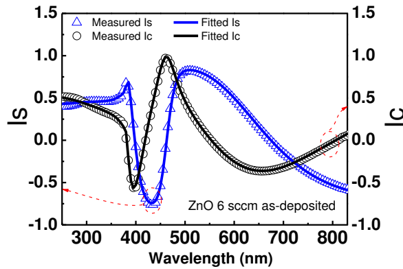
Fig. B.3. Experimental (symbols) and calculated (lines) |S| and |C| ellipsometric parameters measured at 70^\circ for as-deposited ZnO thin films grown at an OFR of 6 sccm.
