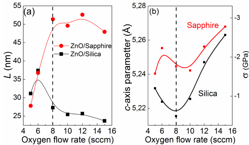
FIG. 3.4. Evolution of the length of coherence domains (a) and of the c -axis parameter of the wurtzite cell structure (b) with the oxygen flow rate of ZnO films deposited on fused silica and (0001)-sapphire. The vertical dashed line indicates the critical oxygen flow rate ( c - OFR ).
