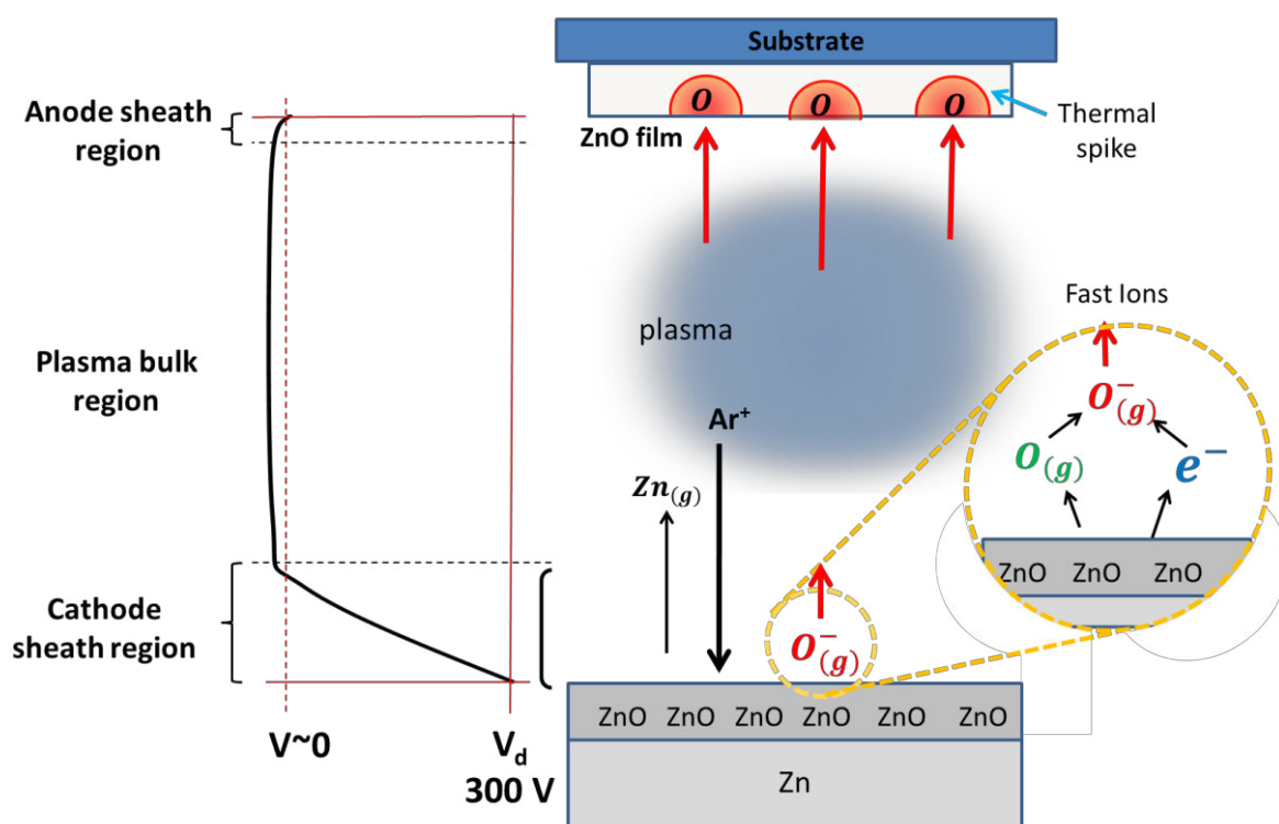
FIG. 3.10. Scheme of the oxygen ion bombardment mechanism after the critical- OFR .
