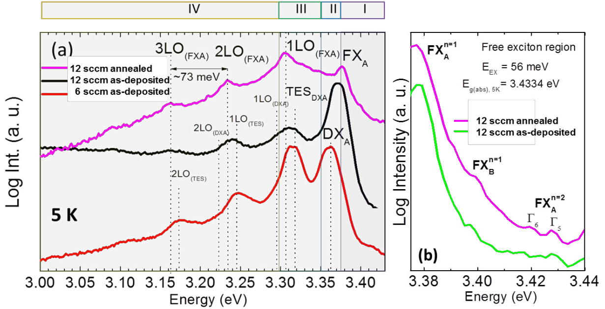
FIG. 3.9. (a) Photoluminescence spectrum at 5 K of ZnO grown at OFRs of 6 and 12 sccm. (b) Zoom of the photoluminescence spectrum at 5 K in the free exciton region for an annealed and an as-deposited ZnO films.
