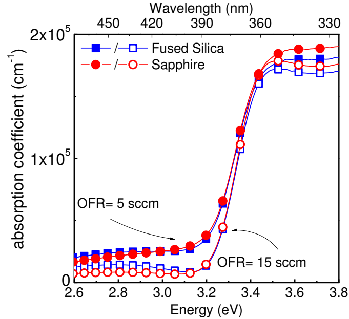
FIG. 3.12. Evolution of the absorption coefficient of ZnO films deposited on fused silica (blue squares) and (0001)-sapphire (red circles) at OFRs of 5 sccm (filled symbol) and 15 sccm (open symbol).
