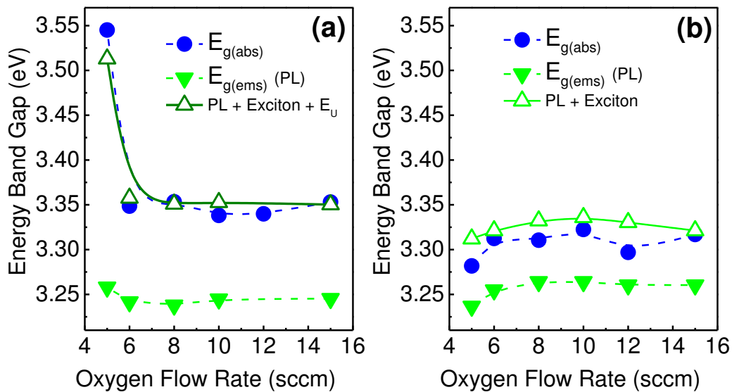
FIG. 3.14. Evolution of the bandgap energy of ZnO thin films with the OFR determined by photoluminescence (emission) (-▼-), ellipsometry (absorption) (-●-) and fit to the data with expressions 3.13 and 3.14 (-Δ-) for (left) as deposited films in the exciton-defects regime and (right) annealed films in the exciton-phonon regime.
