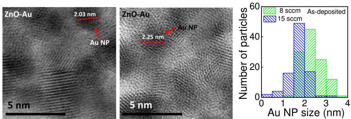
FIG. 4.5. HR-TEM bright field images of ZnO-Au thin nanocomposite films with an Au content of 20 % grown with OFRs of (left) 8 sccm and (center) 15 sccm. (Right) size distribution of Au NPs in as-deposited films (extracted from several images collected in different regions of the TEM lamellae).
