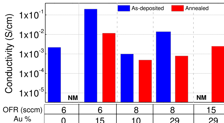
FIG. 4.22. Electrical conductivity of as-deposited and annealed ZnO and ZnO-Au nanocomposite films grown at 6, 8 and 15 sccm with different Au content NM stands for samples non-measurable ( \rho > 10^7 ohm-cm)
