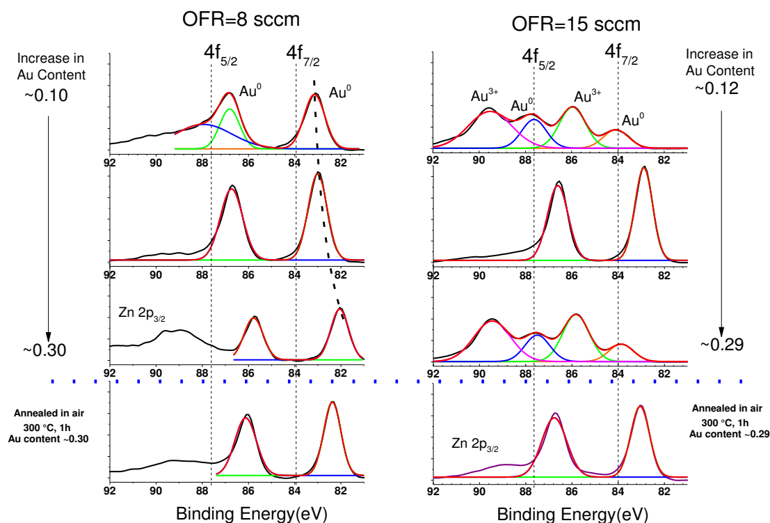
FIG. 4.13. Au-4f core level spectra obtained by XPS measurements of ZnO-Au thin films grown at an OFR of 8 sccm and 15 sccm with different Au contents. The vertical dashed lines represent the 4f level of bulk Au 0 . Below the dotted blue line are shown the spectra of annealed ZnO-Au nanocomposite thin films at the highest Au content of the each series.
