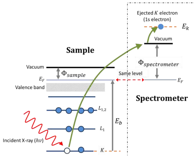
FIG. 2.15. Representation of the mechanism of photoelectron emission by a photon with energy h\nu in X-ray photoelectron spectroscopy (XPS) 124 .
