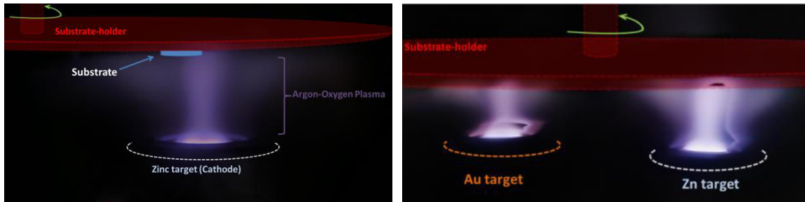
FIG. 2.8. (Above) schematic of the reactive sputtering chamber used for the growth of ZnO and ZnO-Au nanocomposite thin films. The Au target is added for the deposition of ZnO-Au films. (below) Photographs of ZnO and ZnO-Au sputtering process showing the off-axis position of the targets and of the substrate.
