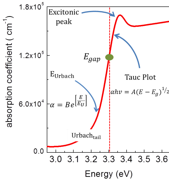
FIG. 1.5. Typical absorption spectrum of a ZnO film. In the near absorption edge, at energies higher than the E_{g(abs)} the absorption coefficient follows the Tauc relation, below the E_{g(abs)} it follows an exponential behavior.
