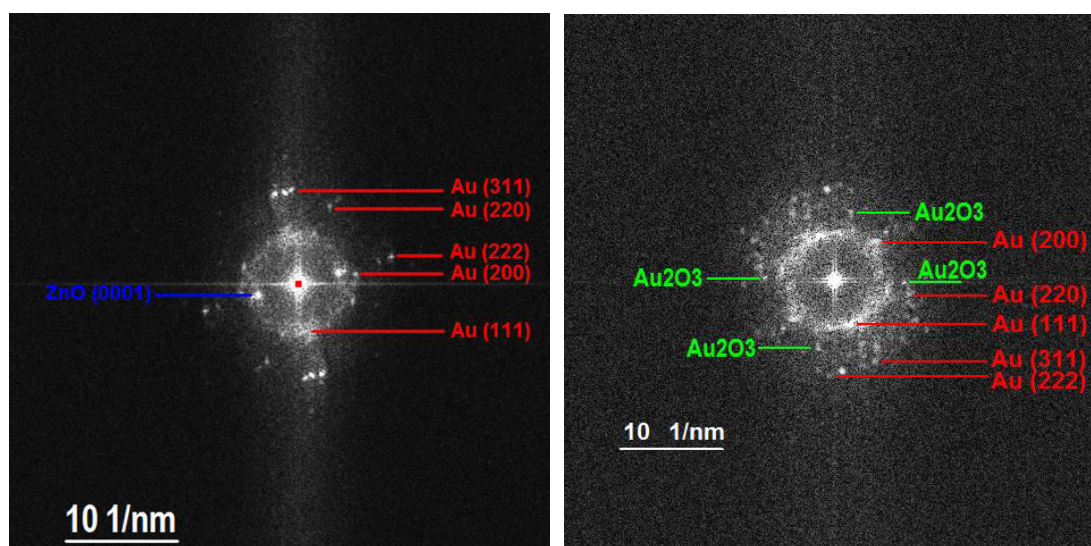
Fig. 4.12. Indexation of the electron diffraction pattern obtained using FFT of HRTEM images of ZnO-Au nanocomposite films grown at low (left) and high (right).
