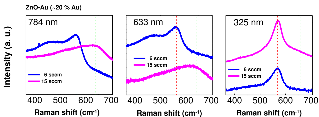
FIG. 4.24. Raman shift spectra measured with three different laser excitations (784, 633 and 325 nm) of as-deposited ZnO-Au nanocomposite films grown with an OFR of 6 sccm (blue) and 15 sccm (violet). The red and green dashed lines represent the position of the ZnO and Au_2O_3 vibration modes respectively.
