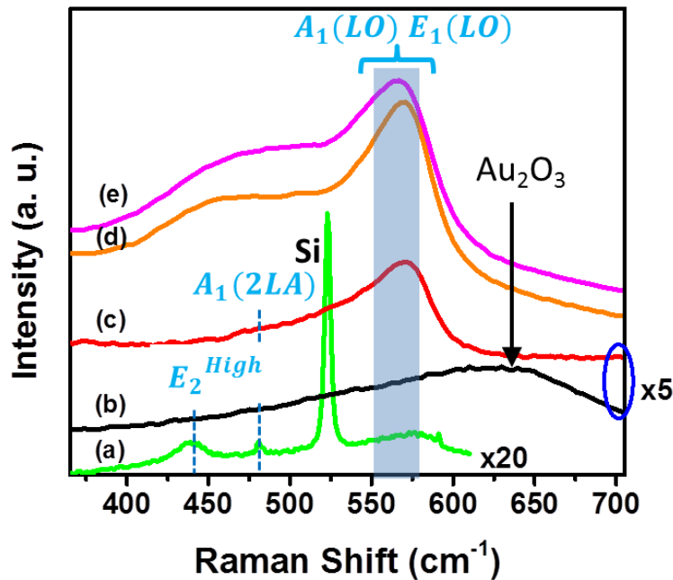
FIG. 4. 23. Raman shift spectra obtained with a 633 nm laser excitation of (a) as-deposited ZnO film grown at 6 sccm, (b) as-deposited ZnO-Au film grown at 15 sccm, (c) ZnO-Au film grown at 15 sccm after an annealing at 300 °C, 1h in air, (d) annealed ZnO-Au film grown at 6 sccm and (e) as-deposited ZnO-Au film grown at 6 sccm. All the ZnO-Au nanocomposite films have an Au content of nearly 20 %. (a) is amplified by a factor of 20 and (b) and (c) are amplified by a factor of 5.
