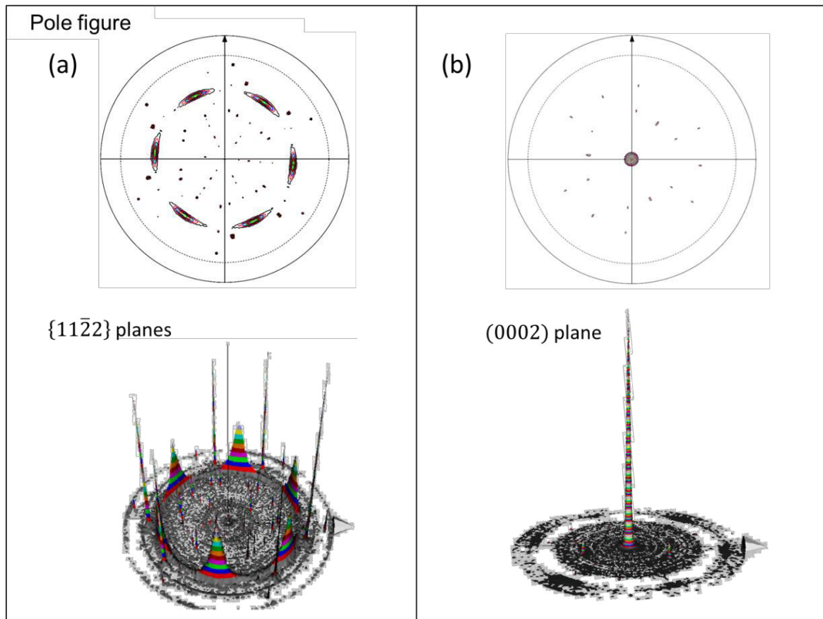
FIG. 3.6. Pole figure and 3D representation of the (a) \{11\bar{2}2\} and (b) (0002) diffraction planes of a ZnO film grown at an OF R of 15 sccm.
