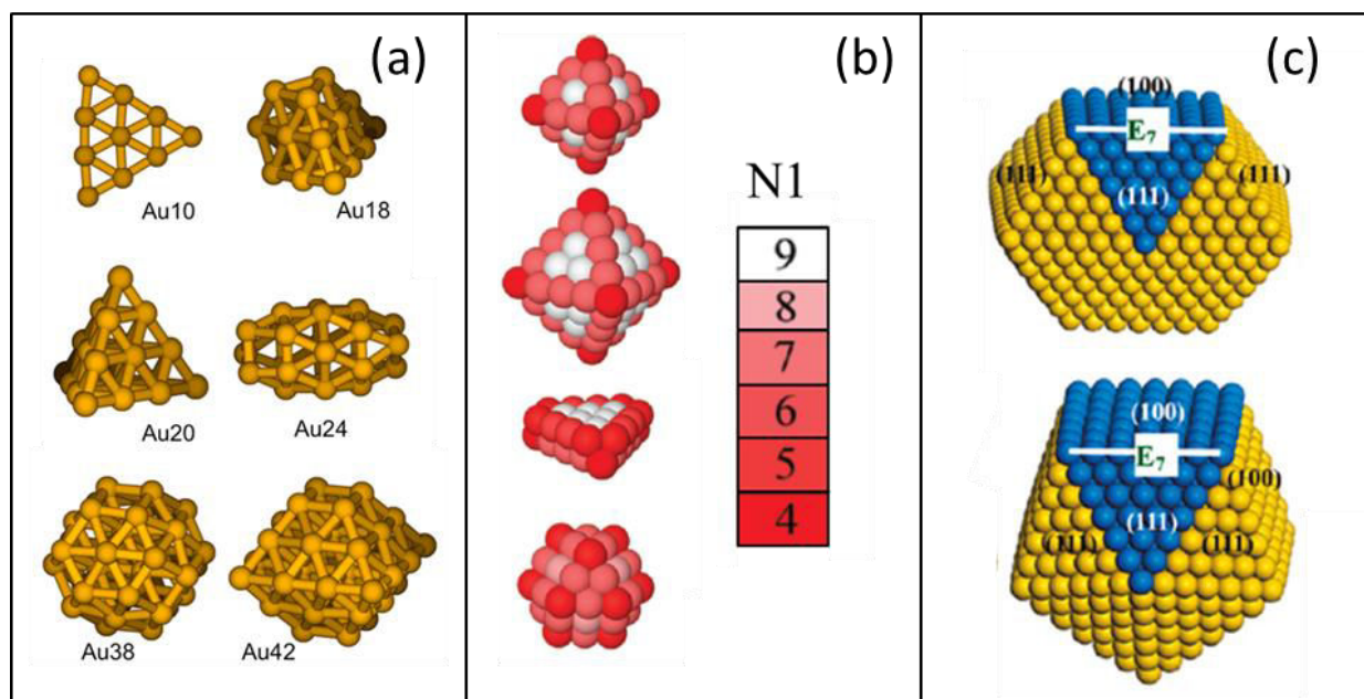
FIG. 1.8. Representation of metallic NPs for (a) 10 to 42 Au Atoms and their corresponding geometrical configurations 57 . (b) Pt NPs with different number of atoms and shapes, N1 present a color-table indicating the coordination number for each geometrical configuration 55 . (c) Dodecahedral Au781 and Penta-star Au932 NPs close to 4 nm in diameter 58 .
