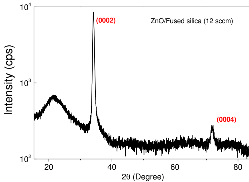
FIG. A.2. X-ray diffractogram (full range) of a ZnO thin film grown at an OF R of 12 sccm on fused silica. Only the (0002) and (0004) planes are detectable in the diffractogram.
