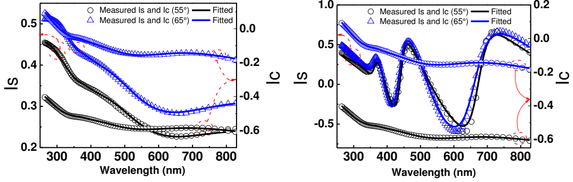
Fig. B.5. Experimental (symbols) and calculated (lines) |S| and |C| ellipsometric parameters measured at 55^\circ and 65^\circ for ZnO-Au nanocomposite films grown at low (left) and high (right) OFR .
