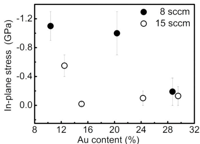
FIG. 4.9. Stress measurements using the curvature method for ZnO-Au nanocomposite films as a function of the Au content and grown with OFrs of 8 sccm (filled circles) and 15 sccm (empty circles).
