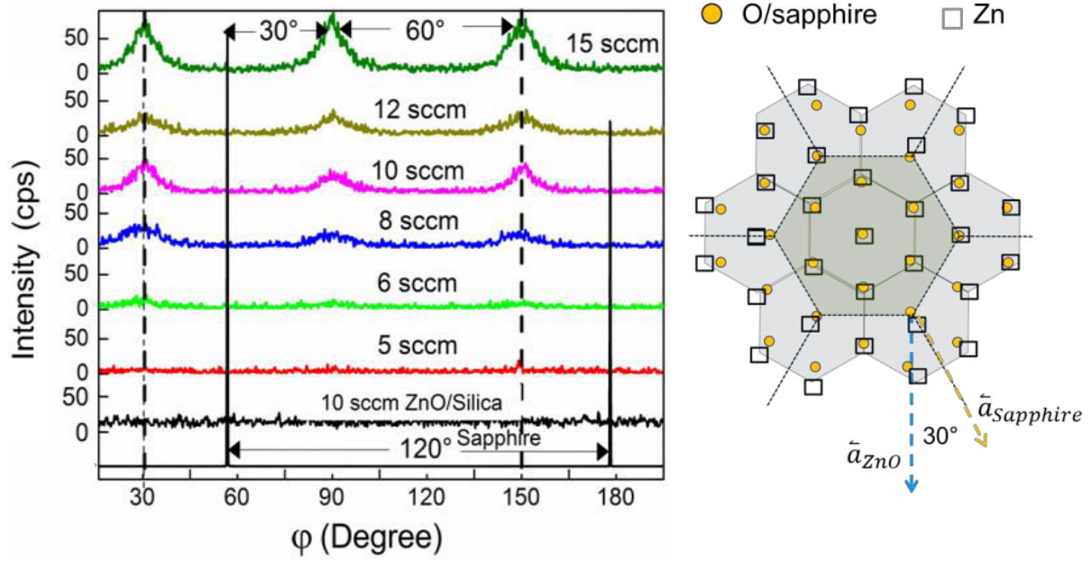
FIG. 3.5. (left) X-ray diffraction \phi -scans for the signal originating from \{10\bar{1}1\} ZnO films deposited on (0001)-sapphire for different oxygen flow rates. The signal from the \{10\bar{1}4\} planes of sapphire and from a ZnO film deposited on silica are used as references. (Right) Representation of the in-plane lattice orientation of ZnO with respect to the \text{Al}_2\text{O}_3 substrate showing the 30^\circ shift. The yellow lattice corresponds to the sapphire and the blue corresponds to the ZnO lattice. The yellow dots are oxygen atoms in the sapphire structure and black squares are the Zn atoms in the ZnO film.
