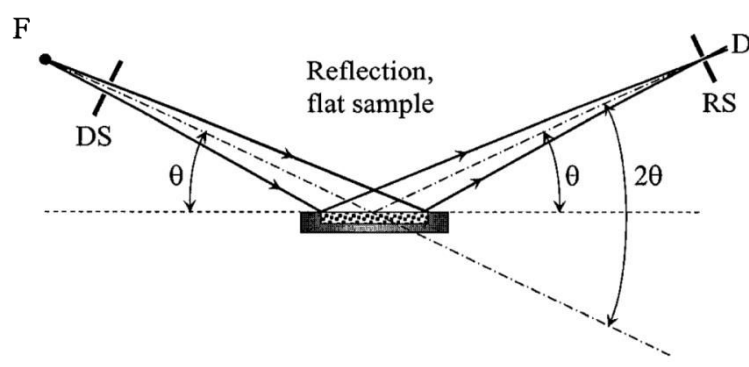
FIG. 2.10. Schematic representation of the Bragg-Brentano geometry. F- Focus of x-ray beam source, DS is the divergence slit, RS is the receiving slit, D is the detector and \theta the bragg angle. The incident beam reaches the sample surface at a determined \theta angle while the detector collects the diffracted beam at an angle 2\theta of the incident beam 119 .
