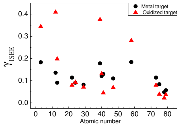
FIG. 2.5. Secondary electron emission for a series of metallic and oxidized targets (adapted from 107 ).
