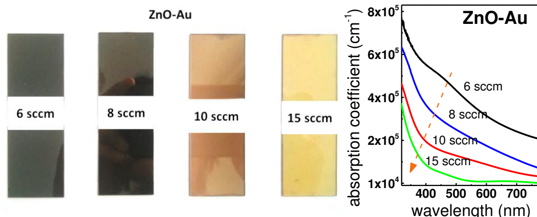
FIG. 4.17. As-deposited ZnO-Au nanocomposite thin film grown with different OFRs . (Left) Photographs of the films from low to high OFR . (Right) dispersion curves of the absorption coefficient of the corresponding films.
