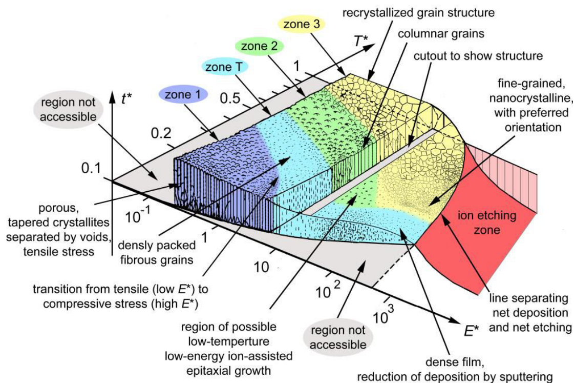
FIG. 2.7. Extended structure zone diagram including situations owing to highly energetic synthesis methods 116 .
