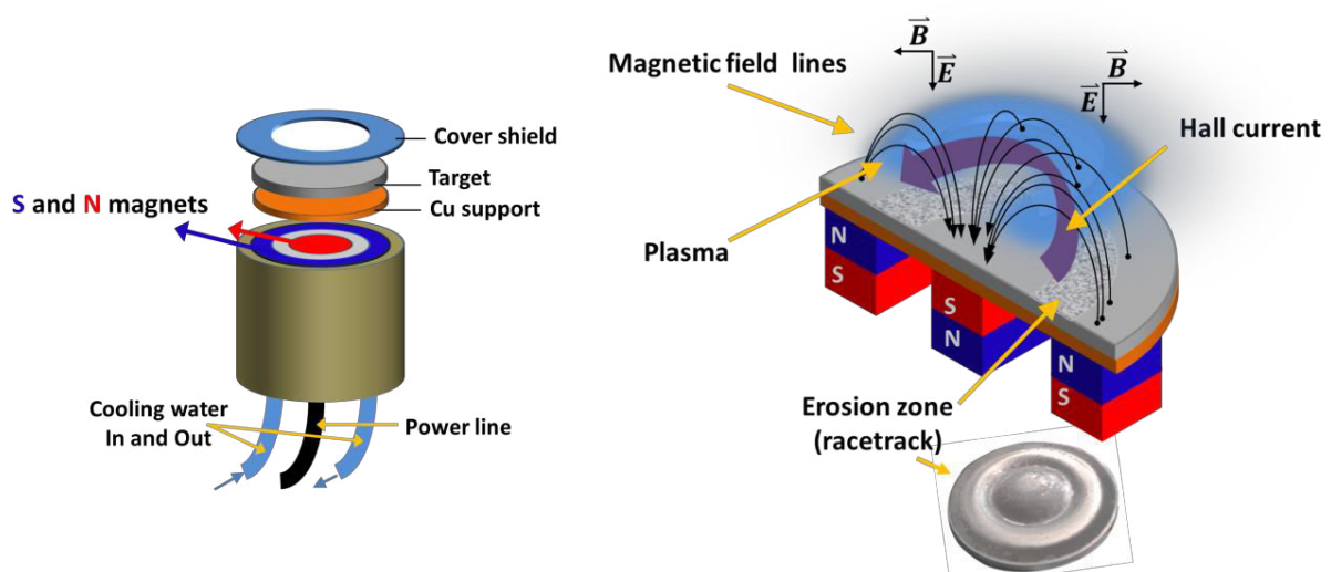
FIG. 2.6. (Left) schematic of the configuration of a magnetron. (Right) magnetron cross section indicating the magnetic field lines, the lorentz forces, the hall current, the erosion zone and the dense plasma region.
