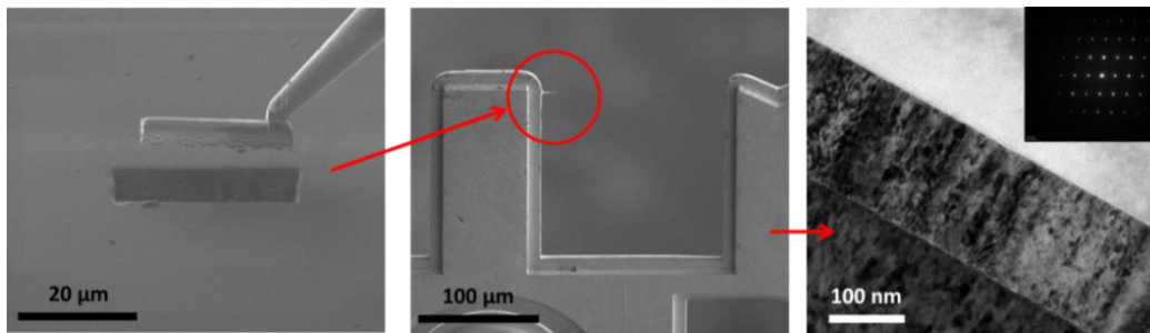
FIG. 2.14. Lift-out method step by step. Elaboration by FIB of a ZnO lamella for TEM measurements. (right) extraction of the specimen after cutting from the film bulk. (Center). Pasting of the TEM lamella to the holder grid. (Right) TEM image of a transverse section of the ZnO film and (inset) SAED pattern of the film.
