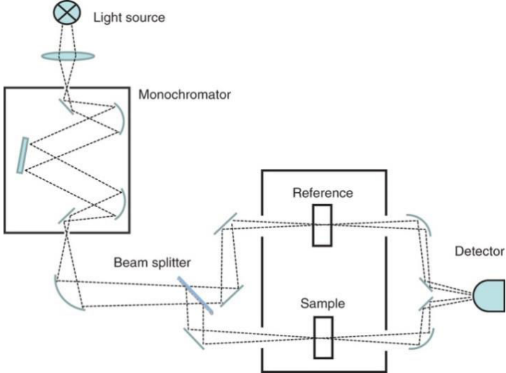
FIG. 2.16. Schematic of a double-beam absorption spectrometer 125 .
