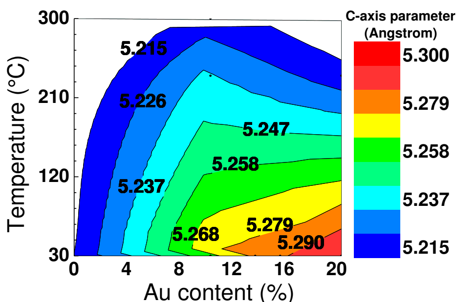
FIG. 4.8. 2D Contour plot of the c -axis parameter determined using the (0002) ZnO diffraction peak of ZnO and ZnO-Au nanocomposite films grown at 8 sccm as a function of the temperature and the gold content.
