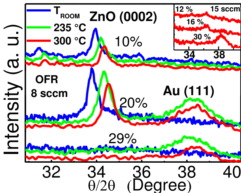
FIG. 4.7. X-ray diffractograms of ZnO-Au nanocomposite thin films grown with an OFR of 8 sccm with different Au contents. In the inset: films grown with an OFR of 15 sccm with 12%, 16% and 30 % Au. For all graphics: Blue line is for as-deposited film, green and red lines are for the films after an annealing process of 1h in air at 235 °C and 300 °C, respectively. Diffratogramms are offset on the y-axis for clarity.
