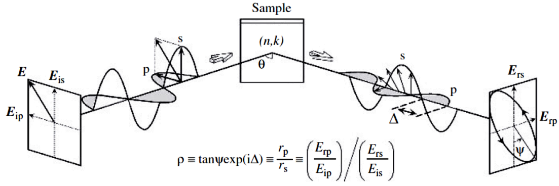
FIG. 2.18 schematic of the experimental configuration used for ellipsometry measurements 131 .
