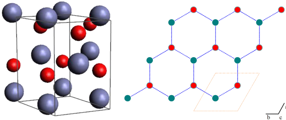
FIG. 1.1. Crystal structure of ZnO wurtzite hexagonal type. (left) side view, (right) top view showing the hexagonal symmetry. Blue and red balls represent Zn and O atoms, respectively.
