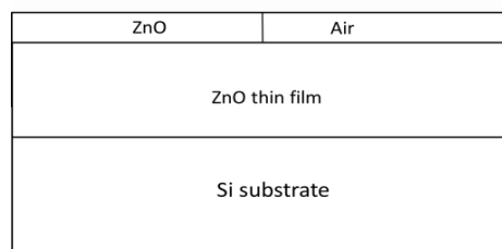
Fig. B.2. Ellipsometric model representing a ZnO thin film. Top layer models the roughness and the bottom layer represents the ZnO film and is treated with the FB dispersion model. The silicon substrate has a known contribution.
