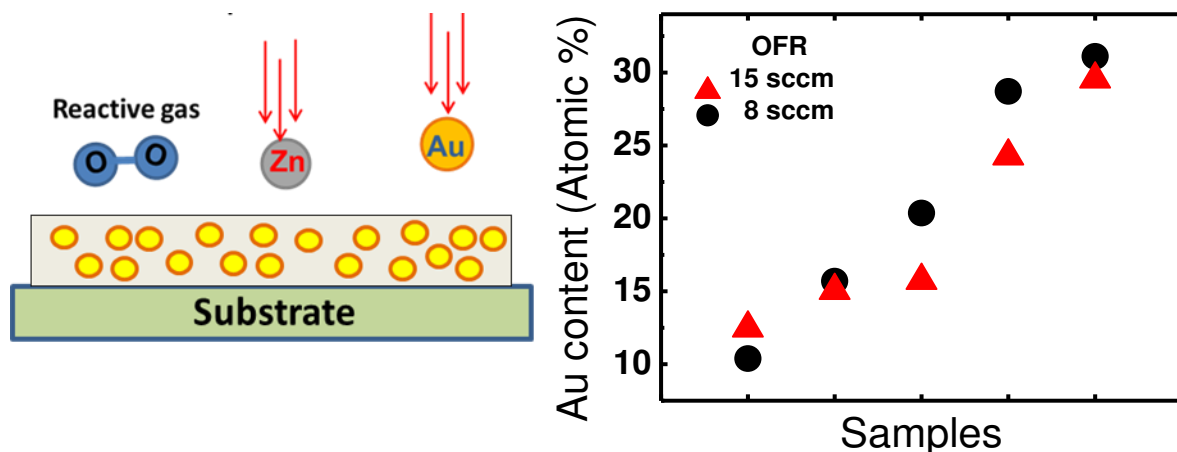
FIG. 4.1. (Left) Representation of the formation of ZnO-Au nanocomposite films. (Right) Au content obtained for ZnO-Au nanocomposite thin films grown at 8 sccm and at 15 sccm. Other samples have also been grown under different conditions that can be consulted in annex C.
