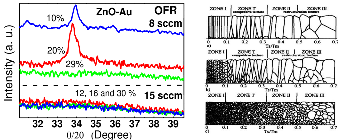
FIG. 4.3. (Left) X-ray diffractograms of ZnO-Au nanocomposite thin films with different Au contents. The films were grown at OFRs of 8 sccm (above the dotted line) and 15 sccm (below the dotted line). The main diffraction peak corresponds to the diffraction by (0002) ZnO planes. Diffractograms are offset on the y-axis for clarity. (Right) Barna and Adamik model showing the influence of the impurities level in the crystalline growth (from top to bottom) at low, medium and high contents 114 .
