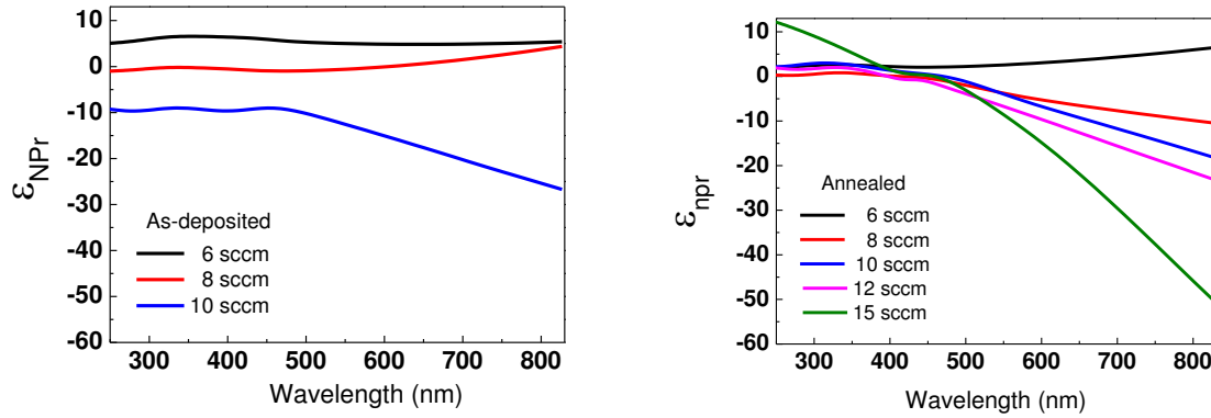
FIG. 4.21. Real part of the Au NPs dielectric function in as-deposited (left) and annealed at 300°C (right) ZnO-Au nanocomposite thin films grown at different OFRs .
