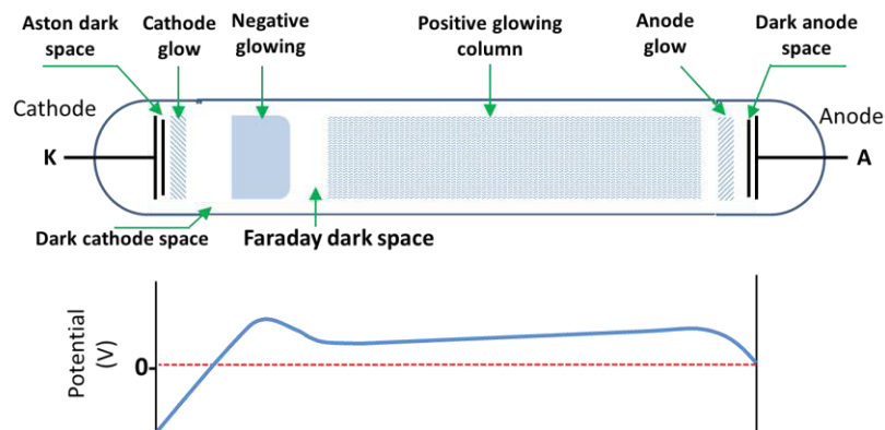
FIG. 2.2. Glow discharge and representation of the voltage profile in the plasma 95 .
