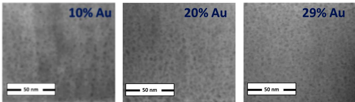
FIG. 4.4. STEM bright field images of transversal cut of ZnO-Au thin nanocomposite films grown with an OFR of 8 sccm with Au contents of (a) 10 %, (b) 20 % and (c) 29 %.
