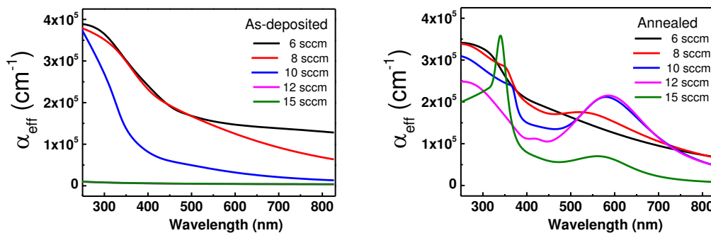
FIG. 4.18. Absorption coefficient of ZnO-Au nanocomposite thin films obtained from ellipsometric measurements and fitting of the data for films grown in the OFR interval from 6 to 15 sccm. The Au content is higher than 15 % in all the films. (Left) As-deposited films. (Right) Annealed films for 1h in air at 300 °C.
