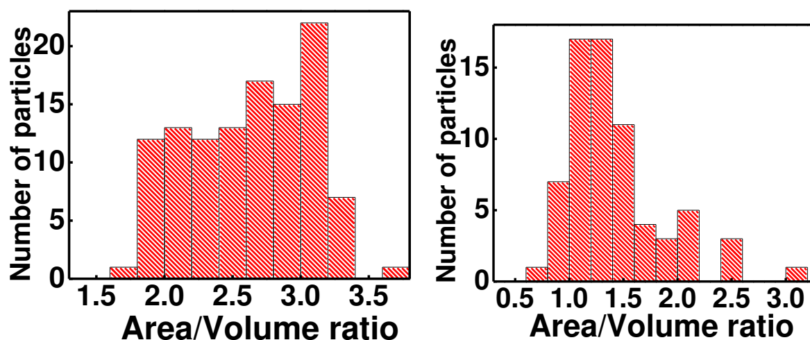
FIG. 4.11. Ratio of surface area to volume of Au NPs in nanocomposite films grown at 8 sccm. (left) As-deposited and (right) annealed at 300 °c, 1h in air.
