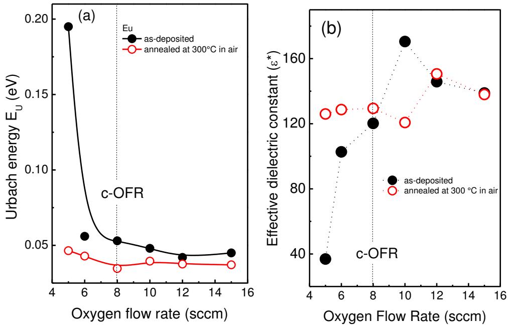
FIG. 3.13. (a). Evolution of the Urbach energy with the OFR. (b) The polaron effective dielectric constant \epsilon^* = (\epsilon_\infty^{-1} - \epsilon_0^{-1})^{-1} of ZnO films deposited at different OFRs as measured by spectroscopic ellipsometry. Full circles correspond to as deposited films and empty circles to ZnO films annealed in air at 300 °C, 1h.
