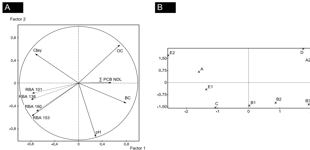
Figure 52 : Principal component analysis between RBA and each soil-characteristic Figure illustrates correlations between soil-characteristic (pH, clay and OC content, concentration of the four studied ND-L-PCBs (101, 138, 153 and 153; \Sigma PCB ND-L) and RBA estimates. PCB 153 was set as reference (RBA 153). PCB 101, 138 and 180 were added as illustrating variables (respectively RBA 101, RBA 138 and RBA 180). Figure A represent the space of variables whereas the figure A represent the space of the individuals.
