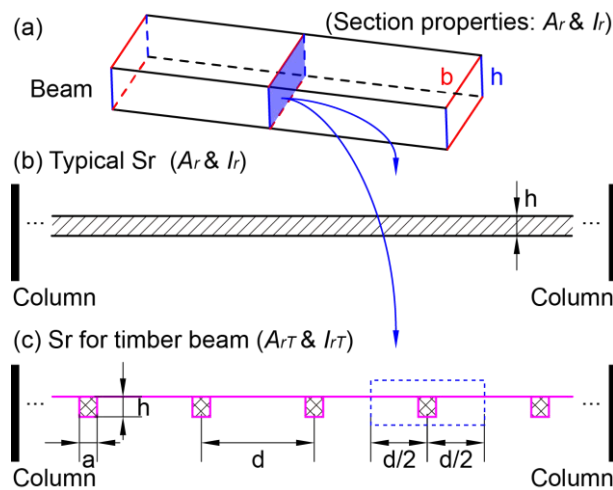
Figure 83. The rectangular cross section for a beam: (a) the cross section in a beam; (b) the typical rectangular cross section between two columns, used for the reinforce concrete buildings; (c) the special rectangular cross section between two columns, used for the unreinforced masonry buildings (ex. The 1 st floor) with the marital of timber
