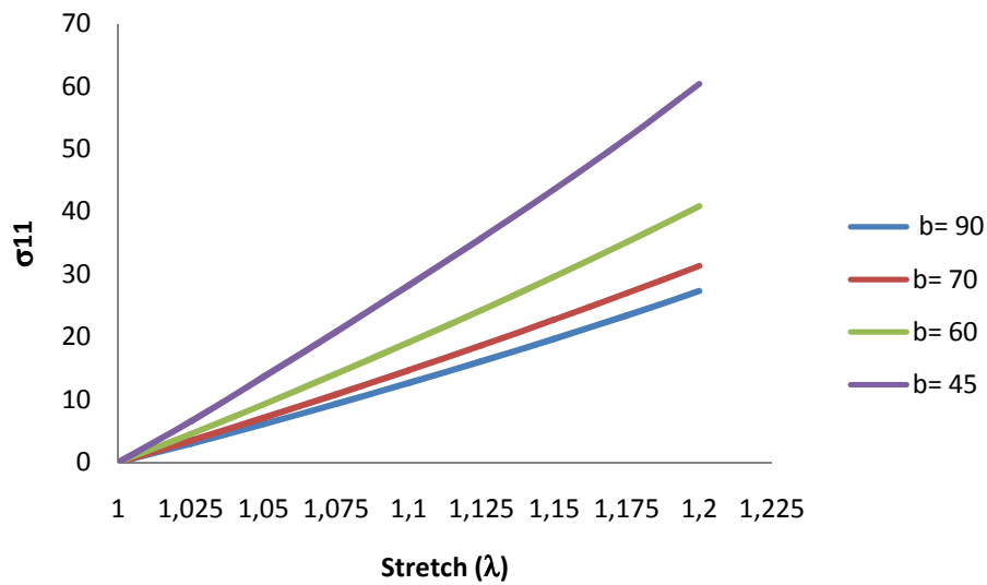
Fig. 5.7 Tensile Cauchy stress versus strain for the non-orthogonal plain weave \beta \in \{90^\circ, 70^\circ, 60^\circ, 45^\circ\}
