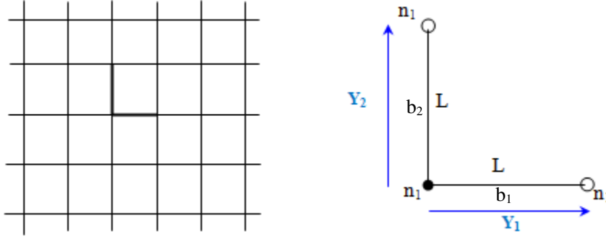
Fig. 7.4 square lattice
