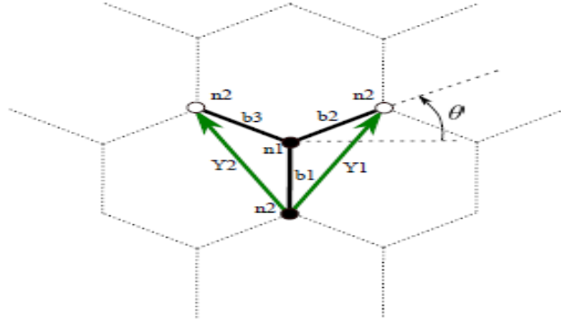
Fig. 7.5 Hexagonal lattice
