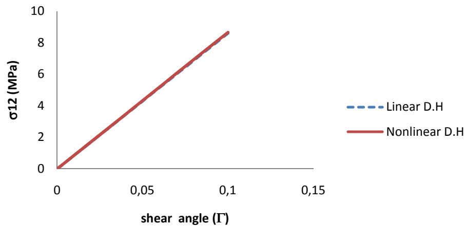
Fig. 3.14 Nonlinear response for the shear stress versus shear angle compared with linear predictions (dashed line)
