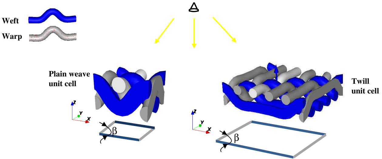
Fig. 5.1 Representative plain weave and twill unit cells top views ( \beta = 90^\circ ).
