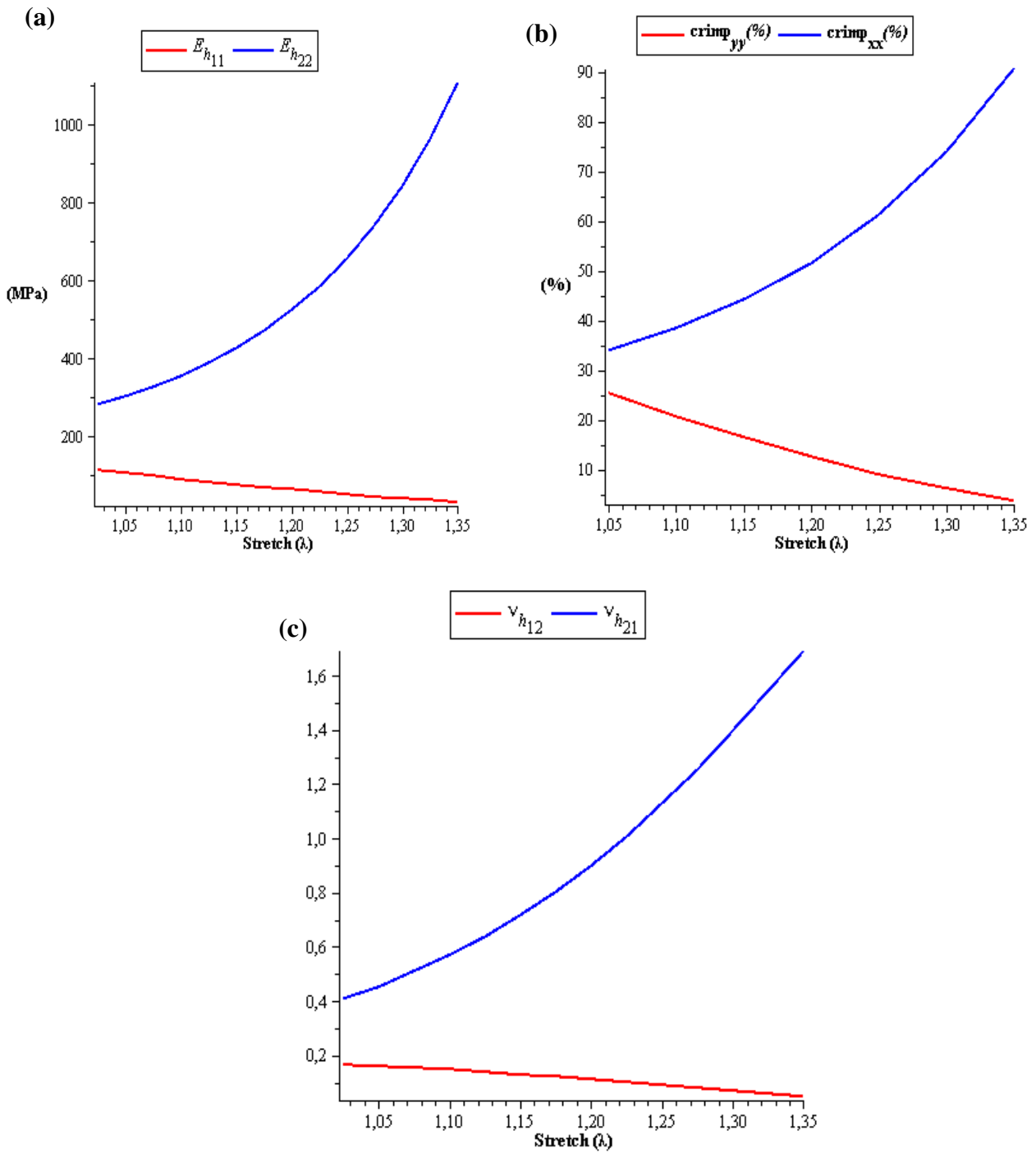
Fig. 5.5 homogenized mechanical and geometrical parameters (a) tensile moduli E_{h_{11}}, E_{h_{22}} (b) crimp ratio \% C_{h_{11}}, \% C_{h_{22}} . (c) Poisson's ratio \nu_{h_{12}}, \nu_{h_{21}} versus stretch in yy- direction.
