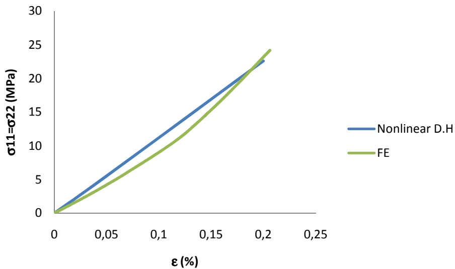
Fig. 5.28 Comparison of the equibiaxial tensile response for the balanced plain weave between the DH method and FEM simulations (ABAQUS).
