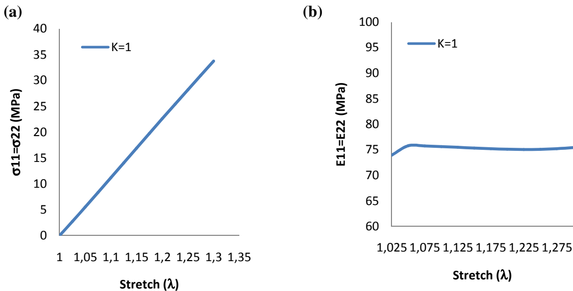
Fig. 5.13 Cauchy stress for the balanced plain weave in xx- direction, yy-direction and tensile moduli versus strain for different biaxial strain ratio, k = 1 .
