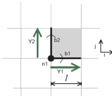
Fig. 3.32. Square unit cell for the erythrocyte network
