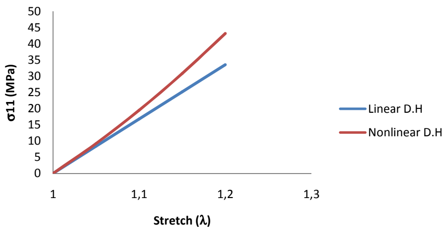
Figure 5.21 Cauchy stress in xx-direction versus stretch (in the same direction) for twill.
