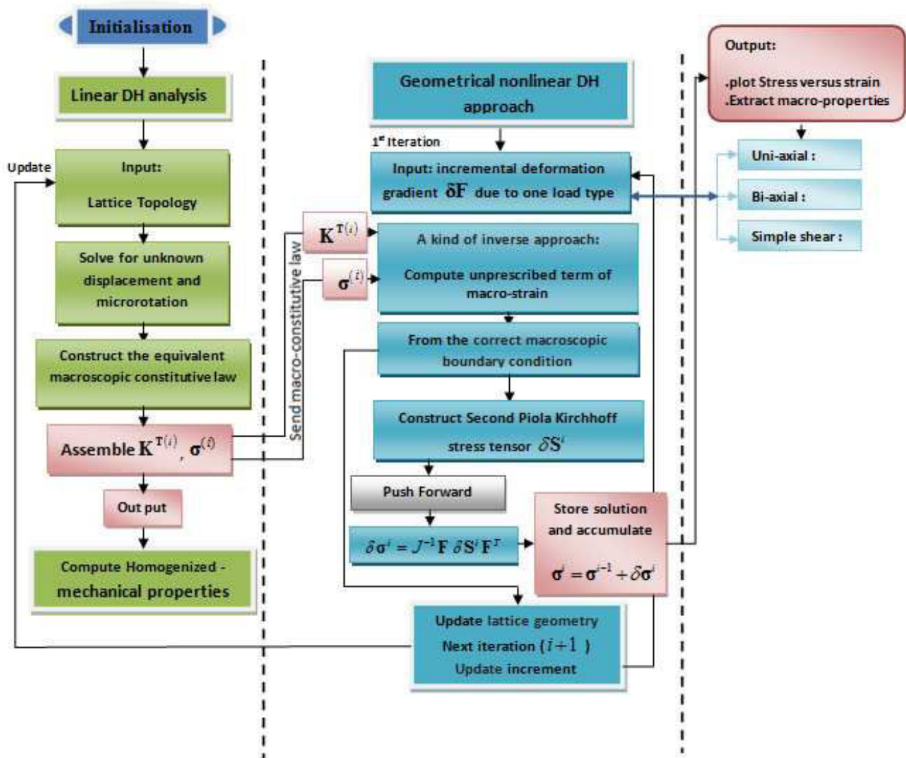
Fig. 4.5 Schematic view of the proposed methodology
