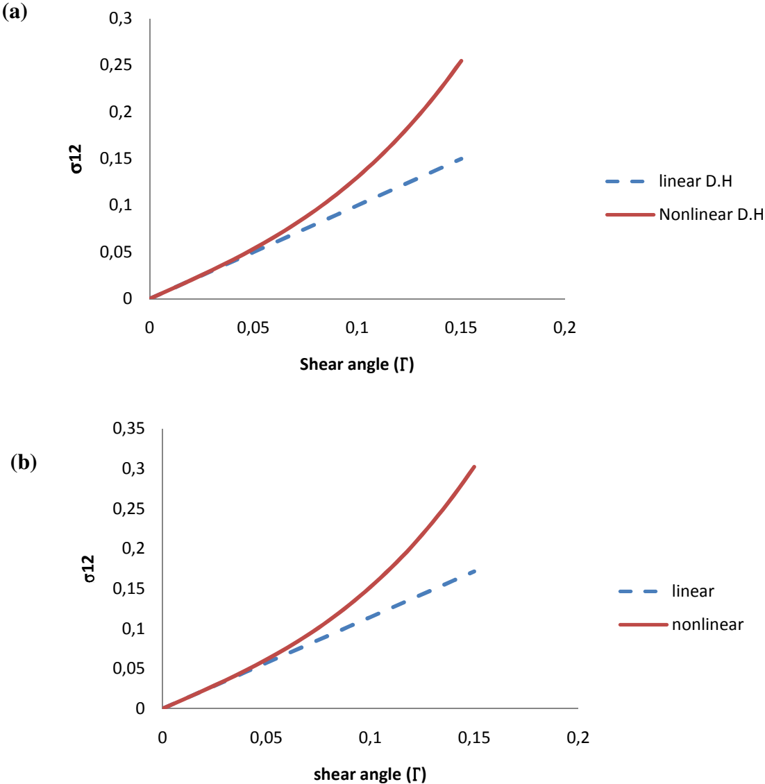
Fig. 3.7 Nonlinear response for the shear stress versus shear angle compared with linear predictions (dashed line)
