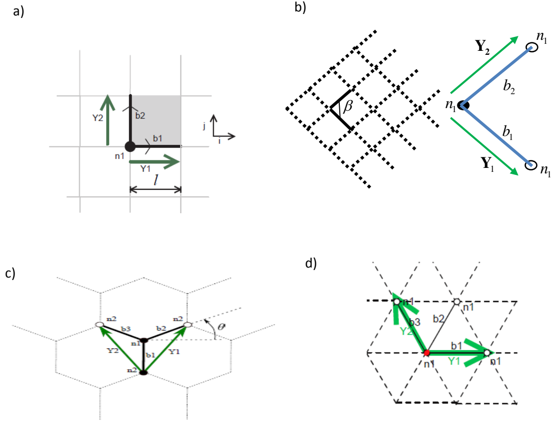
Fig. B.3.1 The analyzed 2D planar Unit cell: (a) square lattice (b) inclined square lattice (c) hexagonal lattice (d) Triangular lattice
