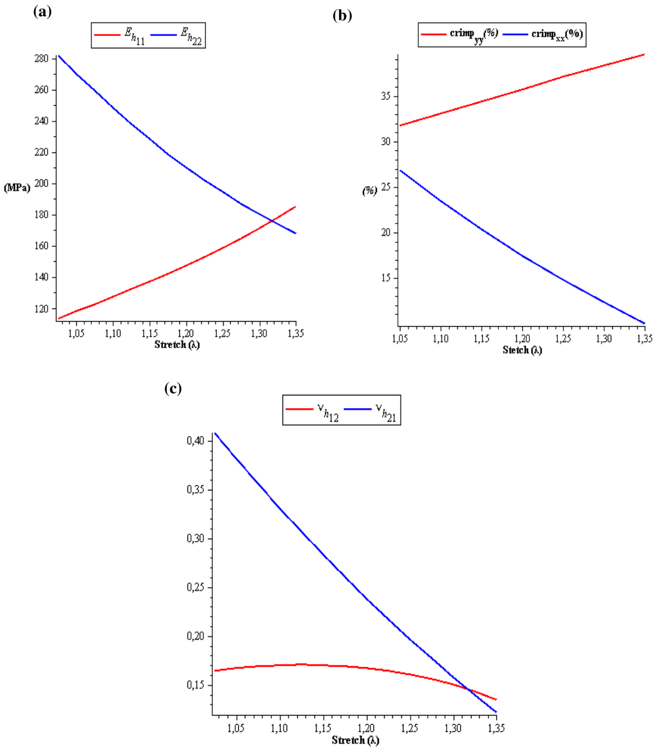
Fig. 5.3: homogenized mechanical and geometrical parameters (a) tensile moduli E_{h_{11}}, E_{h_{22}} (b) crimp ratio \% C_{r_{11}}, \% C_{r_{22}} . (c) Poisson's ratio \nu_{h_{12}}, \nu_{h_{21}} versus stretch in xx- direction.
