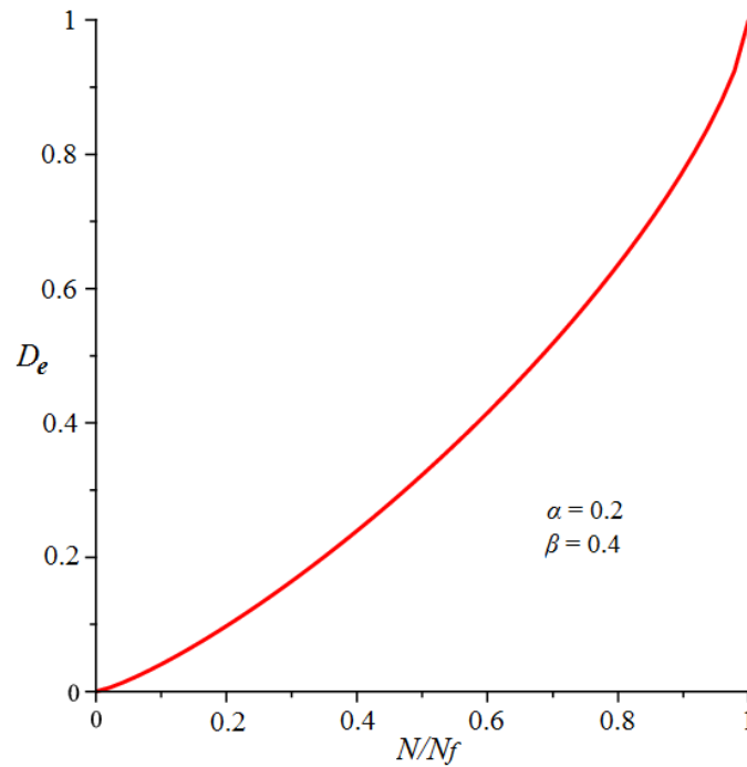
Figure 9.1: Evolution of damage variable ( D_e ) versus the normalized number of cycles (the ratio of the number of cycles N to the number of cycles to failure N_f ).
