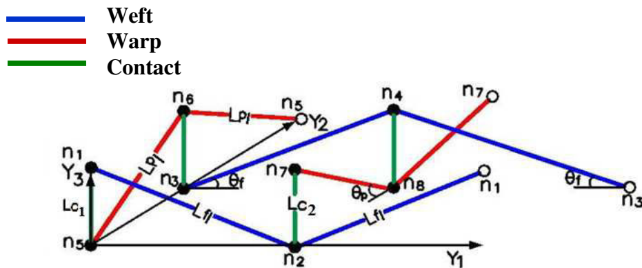
Figure 3.3: A 3D lattice model of 2D plain weave.
