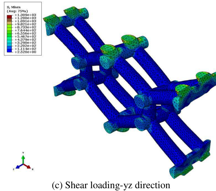
Figure 4.35: Contour plot of von Mises effective stress after uniaxial tensile ((a) and (b)) and shear (c) loading.
