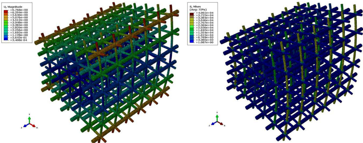
Figure 5.19: Displacement and Von Mises stress distributions due to bending curvature \chi_{yz} = 1 within 6 \times 6 \times 6 unit cells.
