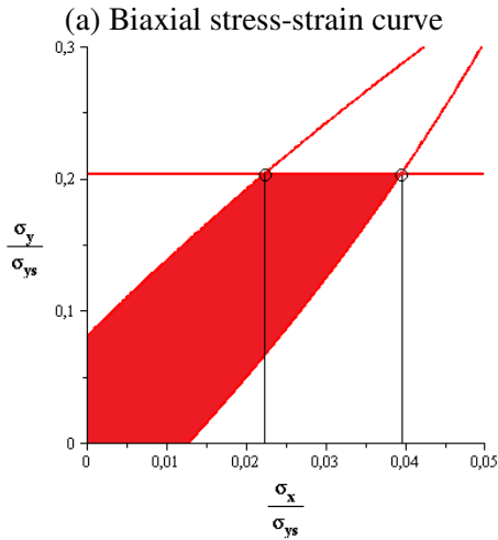
Figure 7.7: Biaxial plastic yield stress determined by FE model from biaxial tension test for trabecular bone lattice. (b) Plastic yield surface (c) Von Mises stress and (d) Equivalent plastic strain.
