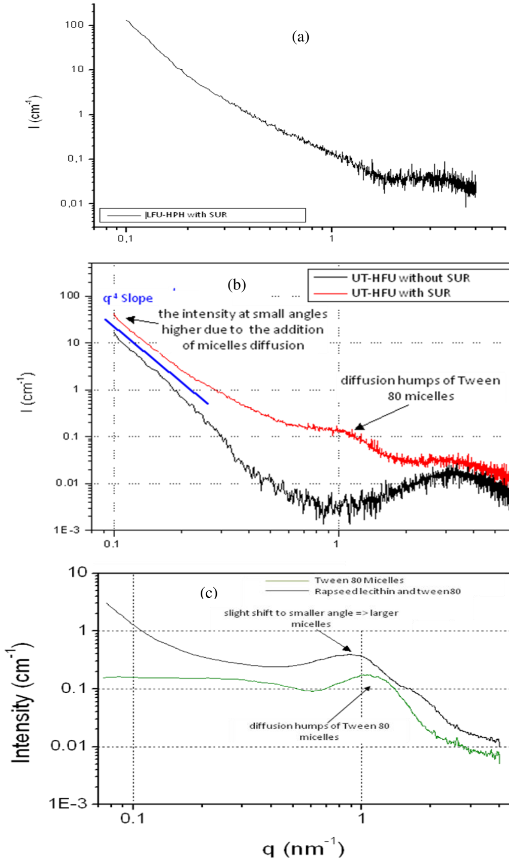
Figure 6: SAXS curves of (a) LFU-HPH emulsion with emulsifiers, (b) UT-HFU emulsion with emulsifiers and without emulsifiers, (c) Polysorbate 80 sample and Polysorbate 80 with rapeseed lecithin.
